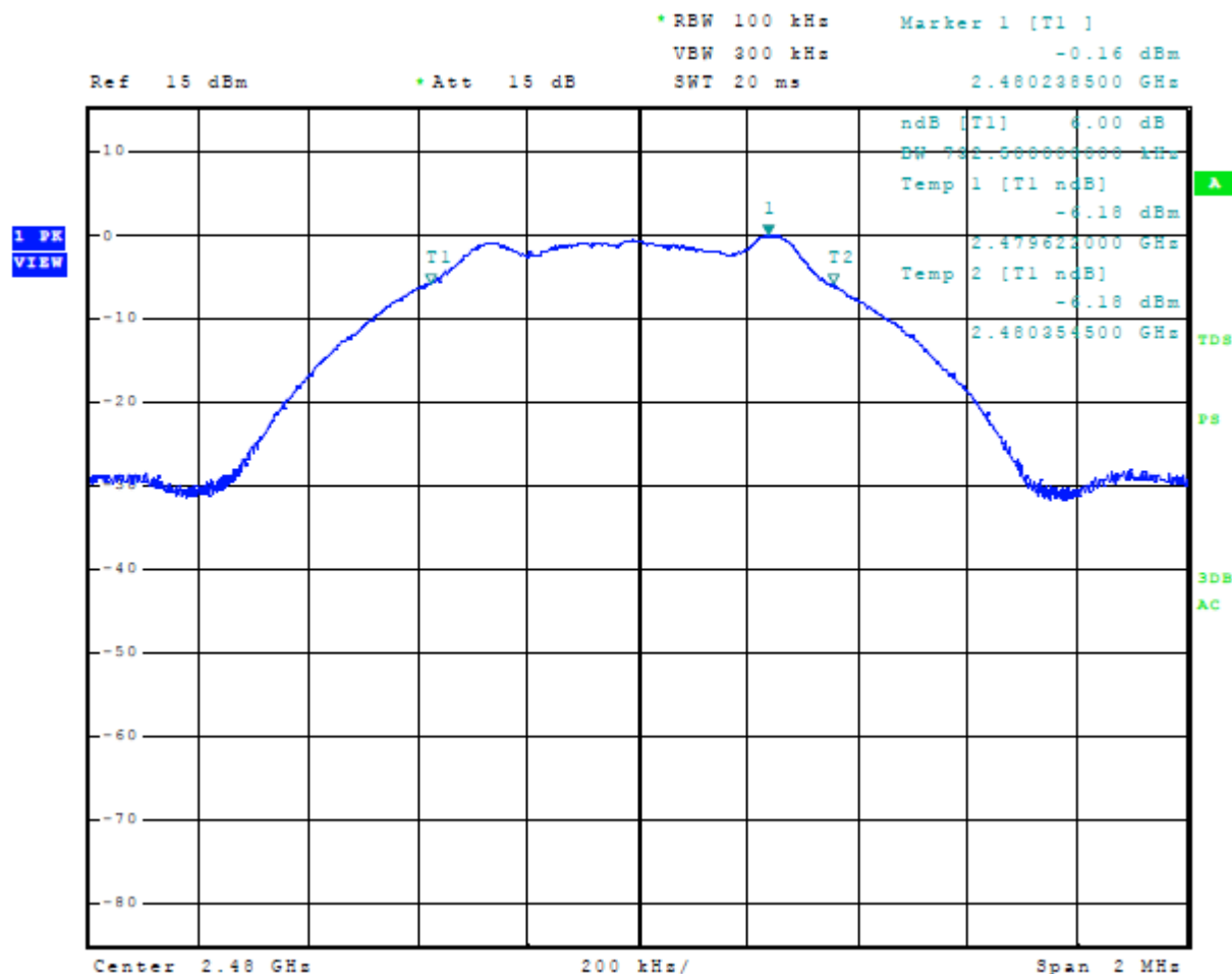
Figure 4 Plot of 6-dB Occupied Bandwidth Mode 1, BT BLE
