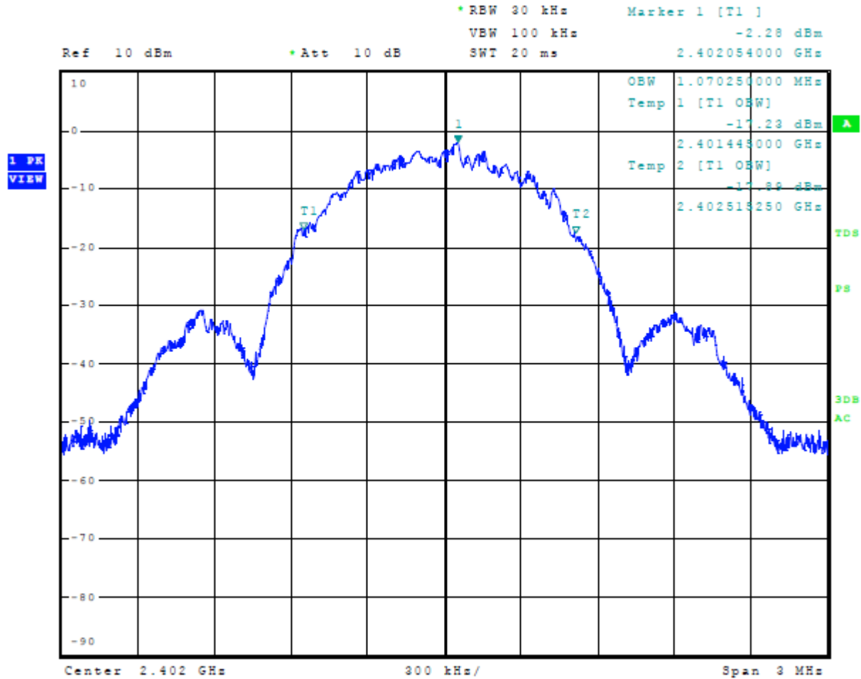
Figure 5 Plot of 99% Occupied Bandwidth Mode 1, BT BLE
