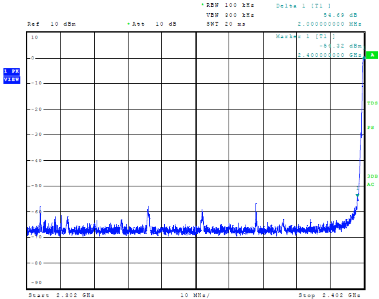
Figure 2 Plot of Emissions Low Band Edge Mode 1, BT BLE
