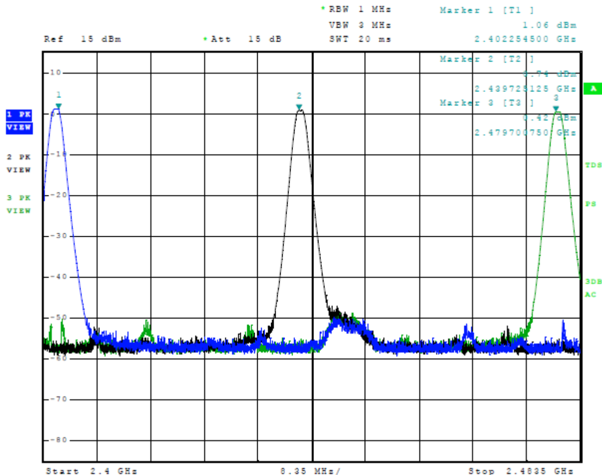
Figure 1 Plot of Transmitter Operation in 2402-2480 MHz Mode 1, BT BLE
