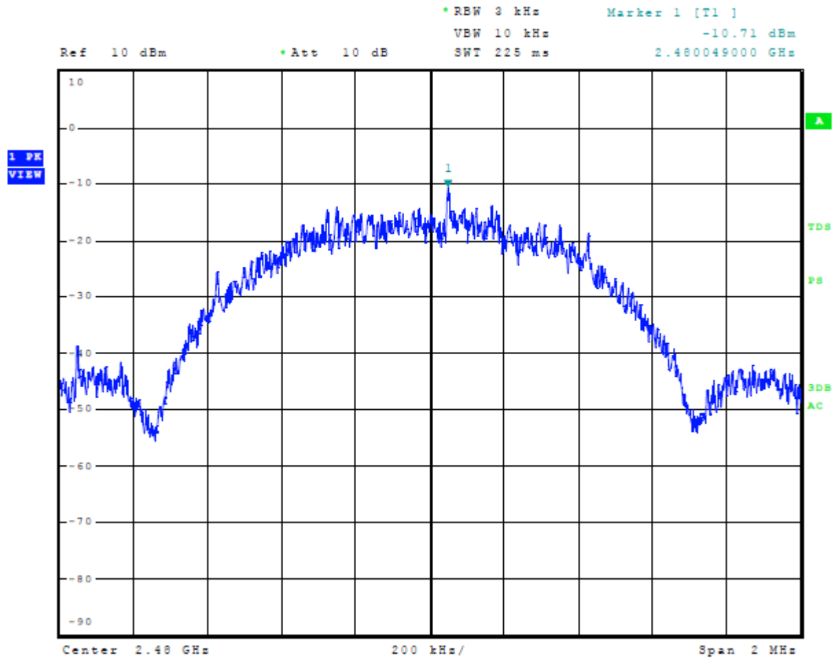
Figure 6 Plot of Transmitter Power Spectral Density Mode 1, BT BLE
