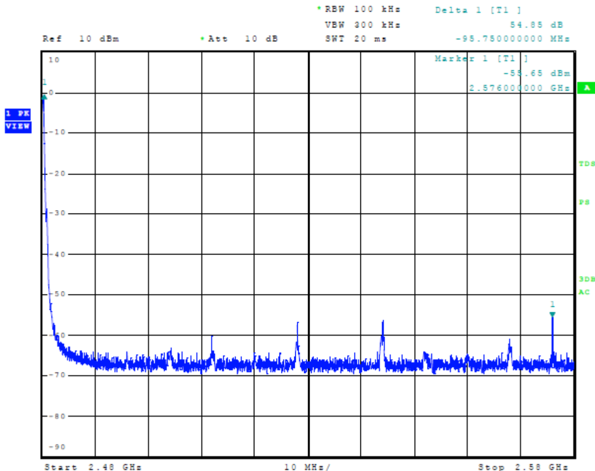
Figure 3 Plot of Transmitter Emissions High Band Edge Mode 1, BT BLE
