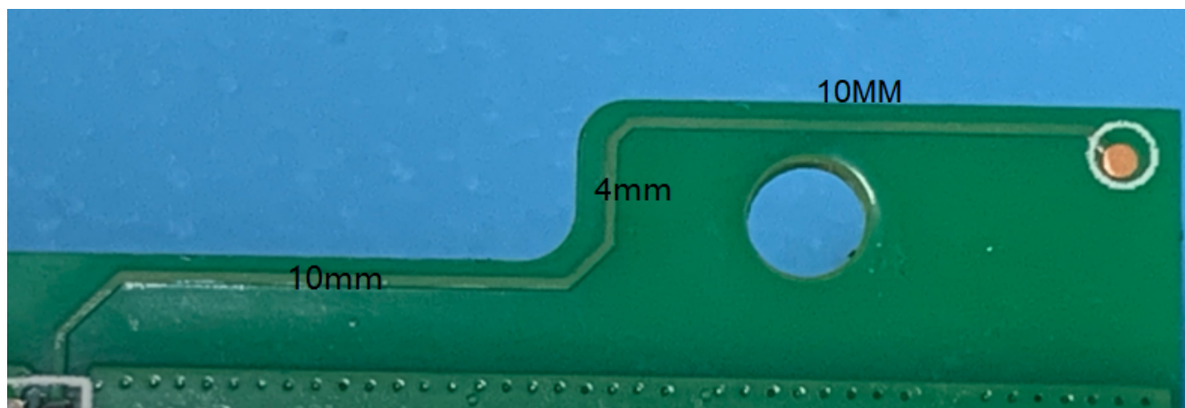
Antenna Photo & Length (mm)
