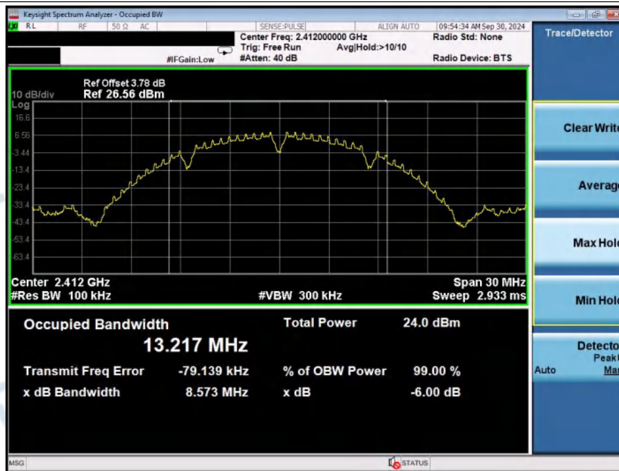
-6dB_Bandwidth_NVNT_ANT1_802_11b_2412
