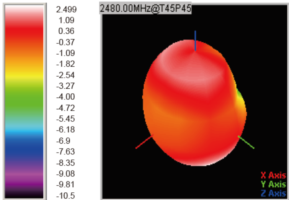
© 3D Gain Pattern (2480 MHz) Unit:dBi
