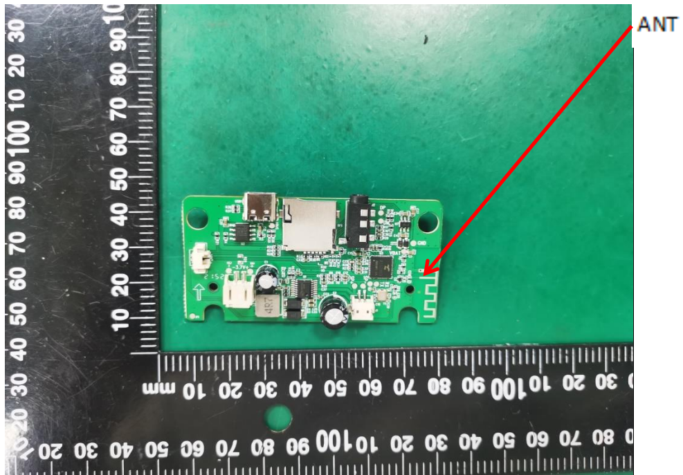
Internal Photo FCC ID: 2A6PZ-BT150
