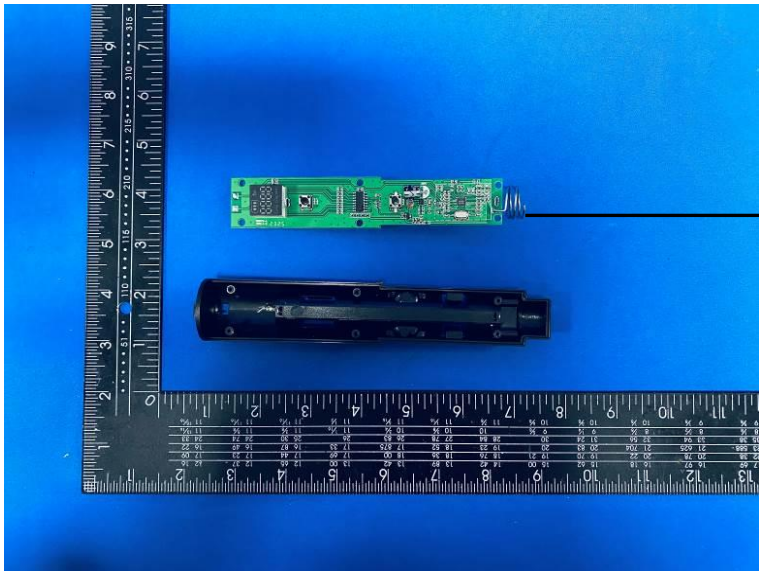
Spring Antenna
