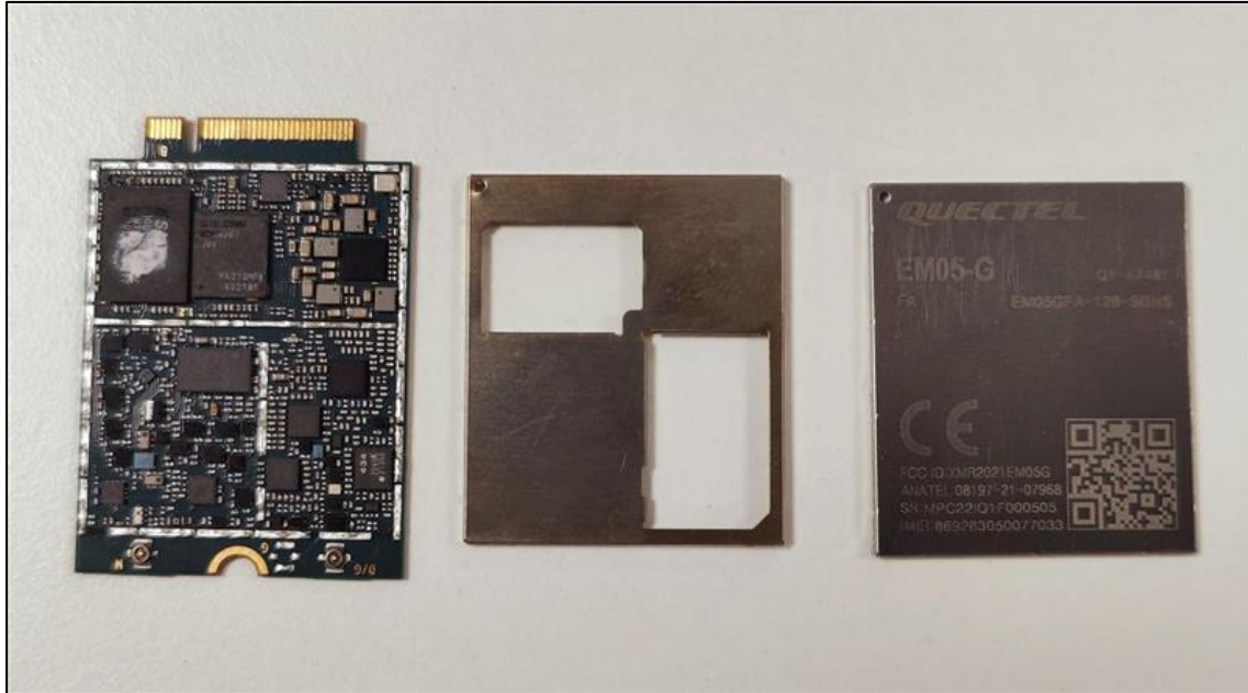
Module with outer & Inner shield removed
