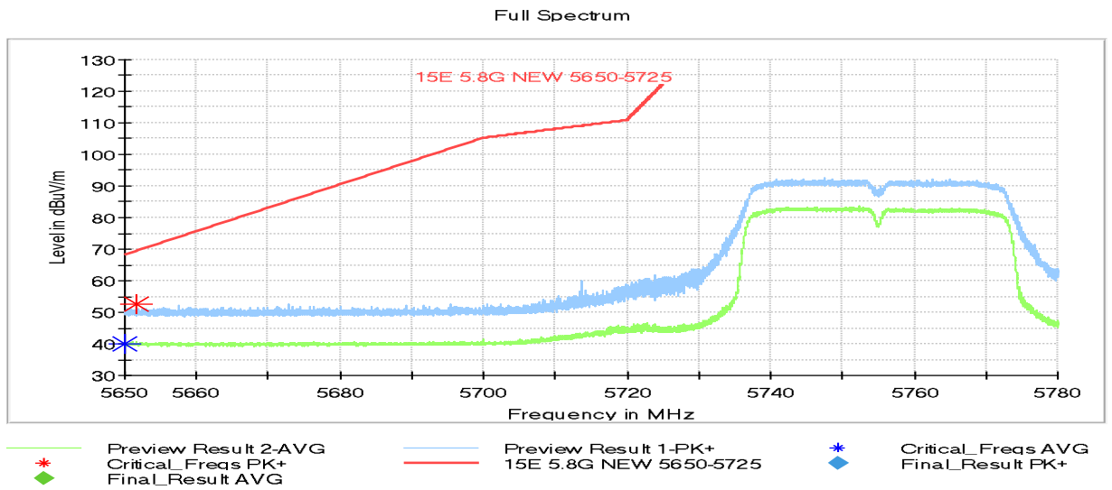
Fig. 5 Band Edges (802.11n-HT40 Ch151, 5755MHz)
