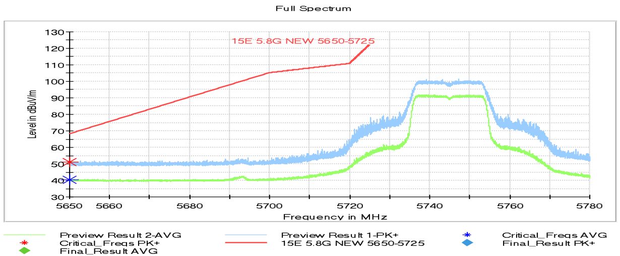
Fig. 3 Band Edges (802.11n-HT20 Ch149, 5745MHz)
