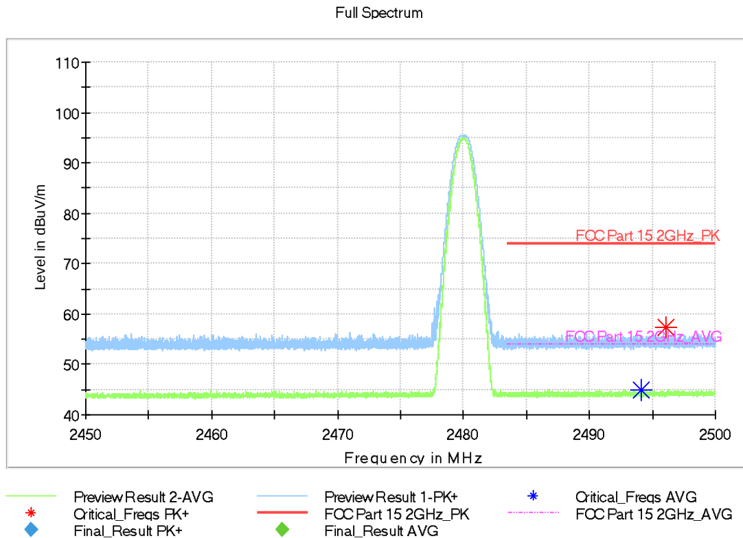
Fig.68. Frequency Band Edges: GFSK, Channel 78, Hopping Off, ch11, 2.45 GHz - 2.50GHz
