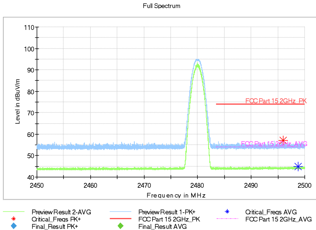
Fig.70. Frequency Band Edges: \pi/4 DQPSK, Channel 78, Hopping Off, 2.45 GHz - 2.50GHz
