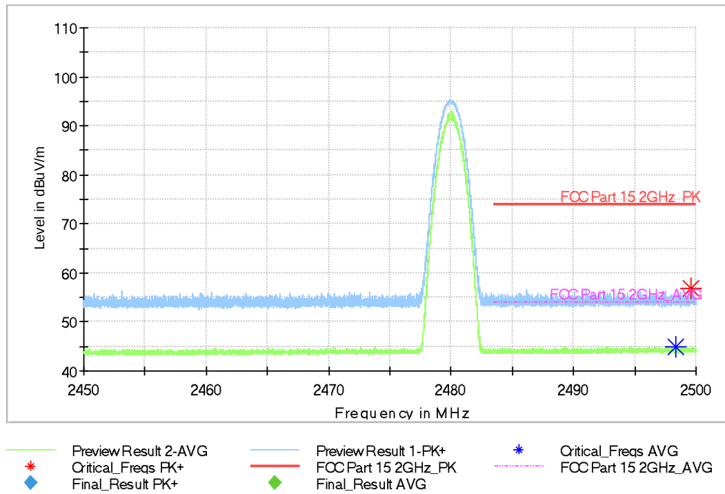
Fig.72. Frequency Band Edges: 8DPSK, Channel 78, 2.45 GHz - 2.50GHz
