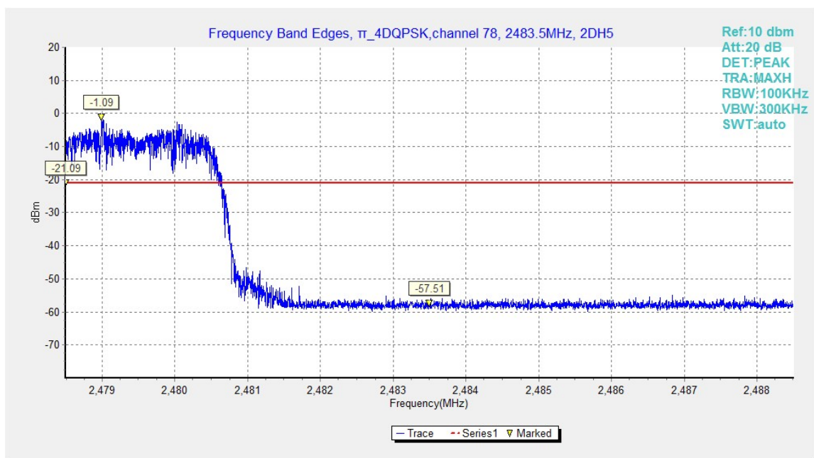
Fig.17. Frequency Band Edges: \pi/4 DQPSK, Channel 78, Hopping On
