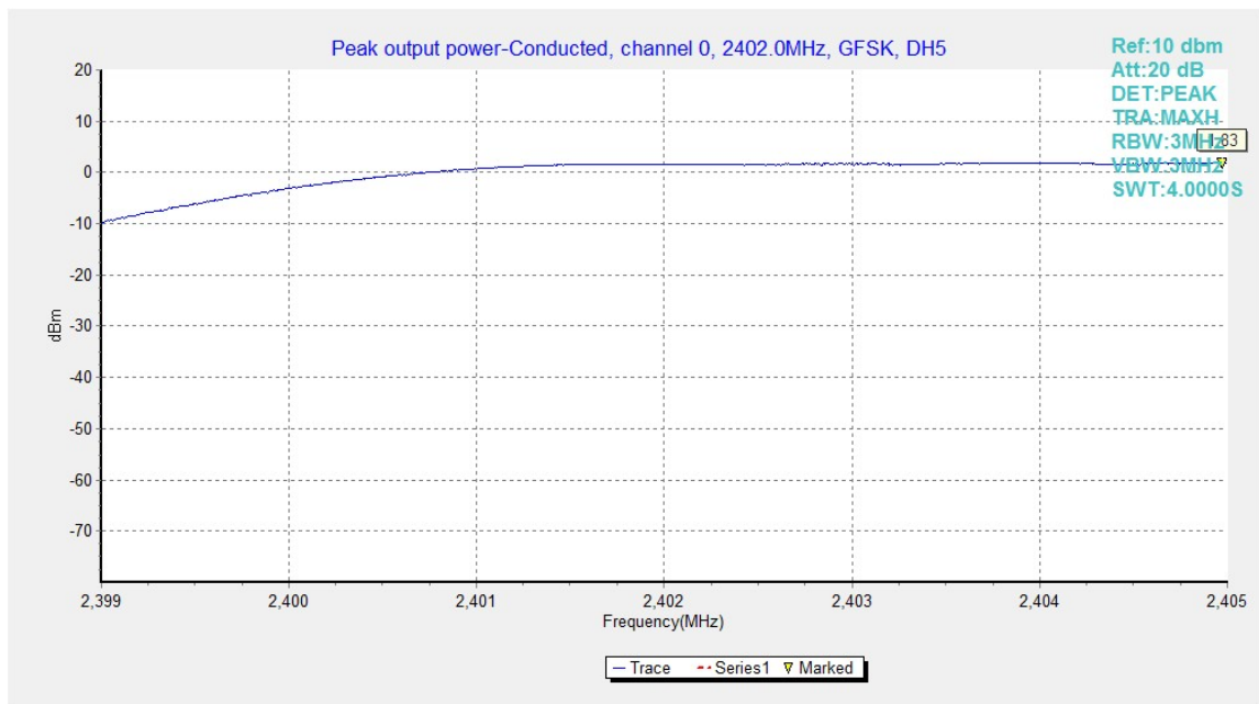
Fig.1. Peak Output Power -Conducted: GFSK, Channel 0,
