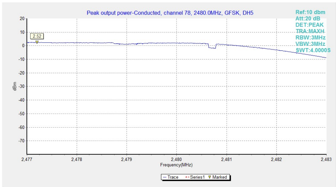
Fig.3. Peak Output Power -Conducted: GFSK, Channel 78,
