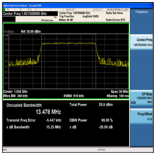
Band2-15MHz-QPSK-18675-75RB#0-13.478
