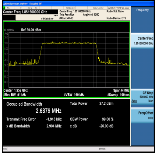
Band2-3MHz-16QAM-18615-15RB#0-2.6879
