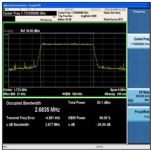
Band4-3MHz-16QAM-20175-15RB#0-2.6835
