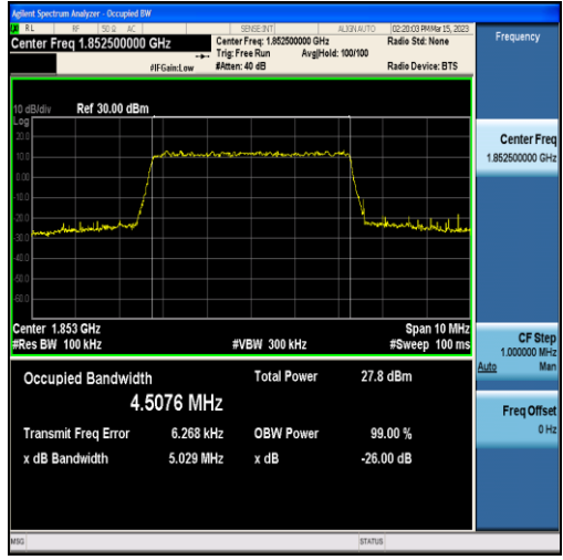
Band2-5MHz-16QAM-18625-25RB#0-4.5076
