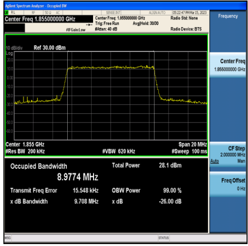
Band2-10MHz-16QAM-18650-50RB#0-8.9774
