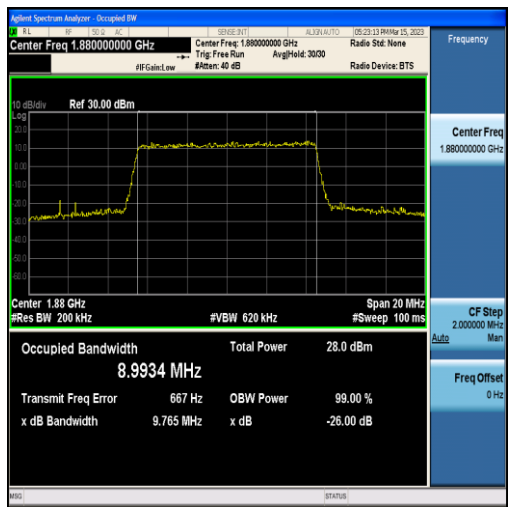
Band2-10MHz-16QAM-18900-50RB#0-8.9934
