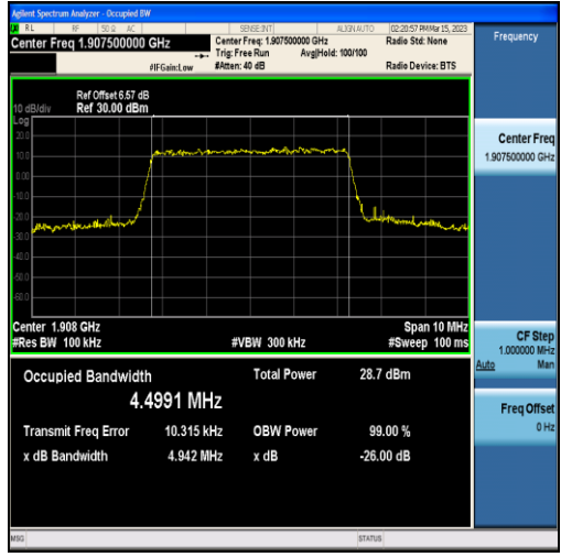
Band2-5MHz-QPSK-19175-25RB#0-4.4991
