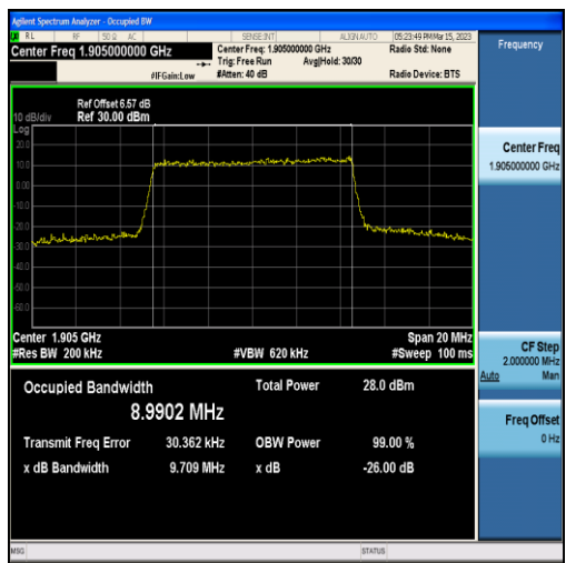
Band2-10MHz-16QAM-19150-50RB#0-8.9902
