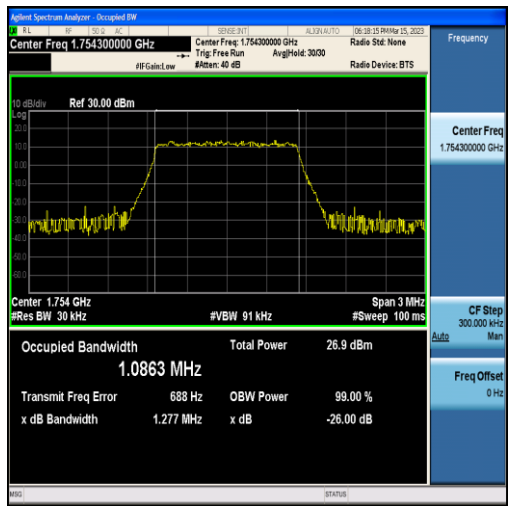
Band4-1.4MHz-QPSK-20393-6RB#0-1.0863
