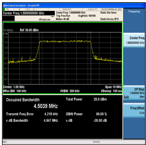
Band2-5MHz-QPSK-18900-25RB#0-4.5039
