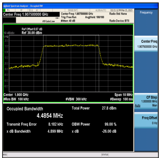
Band2-5MHz-16QAM-19175-25RB#0-4.4854
