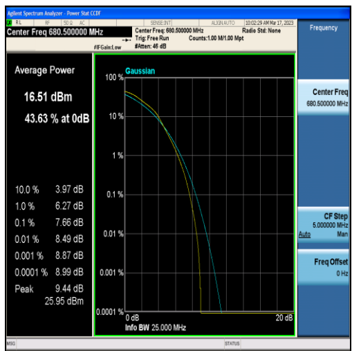
Band71-5MHz-16QAM-133297-25RB#0
