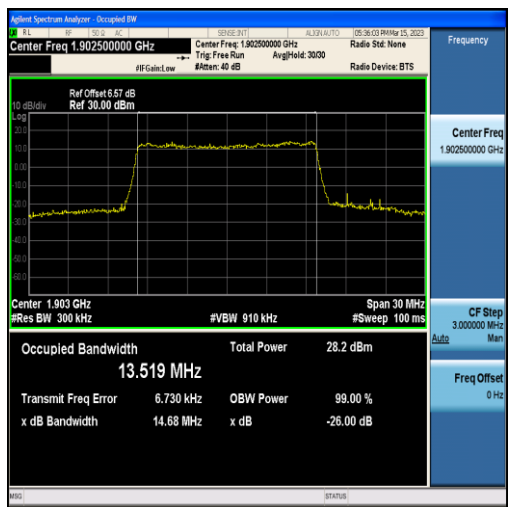
Band2-15MHz-16QAM-19125-75RB#0-13.519
