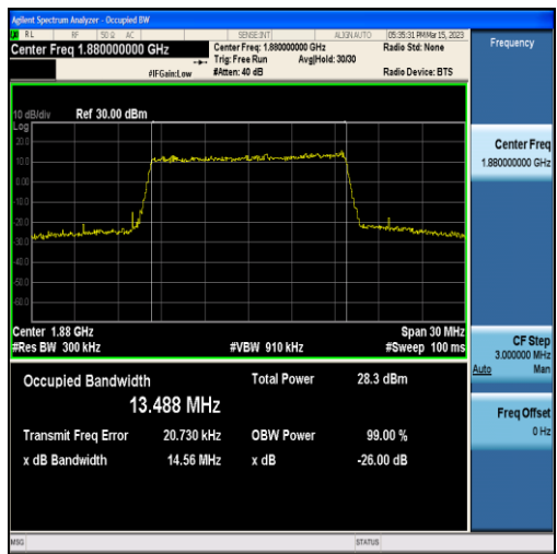
Band2-15MHz-16QAM-18900-75RB#0-13.488
