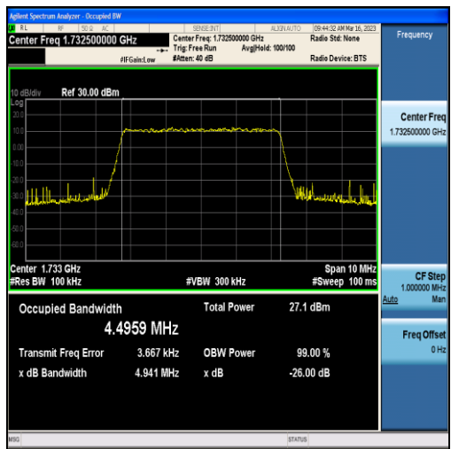
Band4-5MHz-16QAM-20175-25RB#0-4.4959
