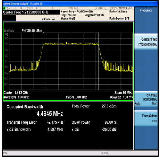
Band4-5MHz-16QAM-19975-25RB#0-4.4845
