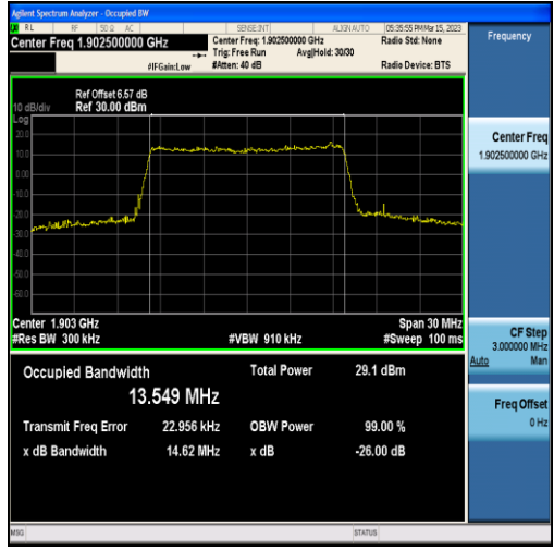
Band2-15MHz-QPSK-19125-75RB#0-13.549
