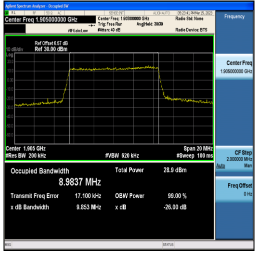
Band2-10MHz-QPSK-19150-50RB#0-8.9837
