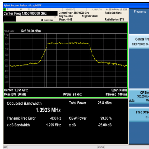
Band2-1.4MHz-16QAM-18607-6RB#0-1.0933
