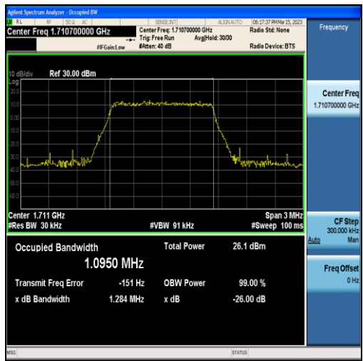
Band4-1.4MHz-16QAM-19957-6RB#0-1.0950
