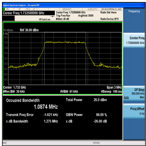
Band4-1.4MHz-16QAM-20175-6RB#0-1.0874
