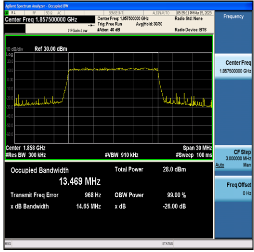
Band2-15MHz-16QAM-18675-75RB#0-13.469
