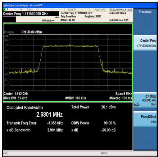
Band4-3MHz-16QAM-19965-15RB#0-2.6801
