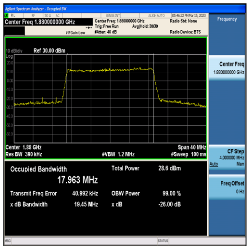
Band2-20MHz-16QAM-18900-100RB#0-17.963
