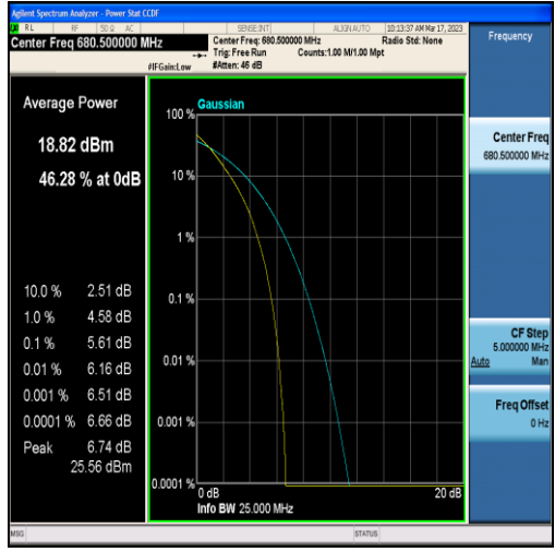
Band71-10MHz-QPSK-133297-50RB#0
