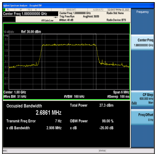
Band2-3MHz-16QAM-18900-15RB#0-2.6861
