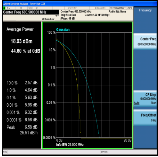
Band71-15MHz-QPSK-133297-75RB#0
