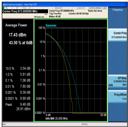
Band71-20MHz-16QAM-133222-100RB#0
