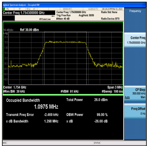
Band4-1.4MHz-16QAM-20393-6RB#0-1.0975
