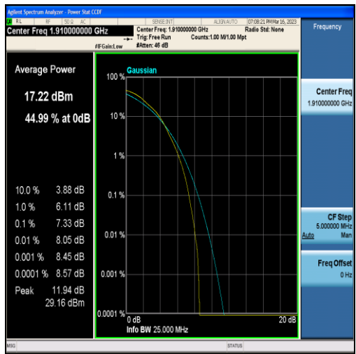
Band25-10MHz-16QAM-26640-50RB#0
