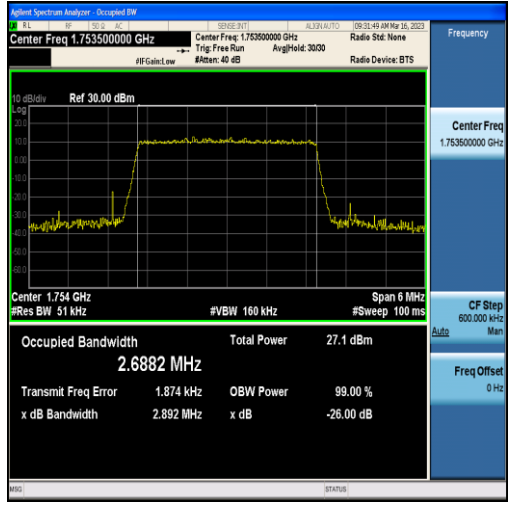
Band4-3MHz-QPSK-20385-15RB#0-2.6882
