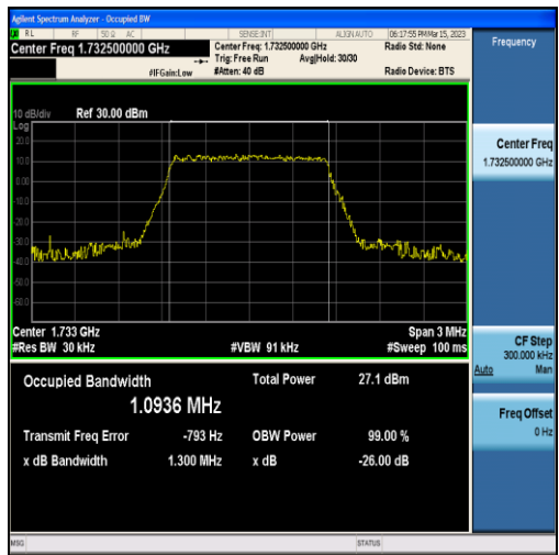
Band4-1.4MHz-QPSK-20175-6RB#0-1.0936
