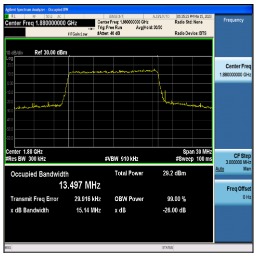
Band2-15MHz-QPSK-18900-75RB#0-13.497
