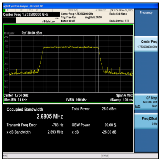
Band4-3MHz-16QAM-20385-15RB#0-2.6805
