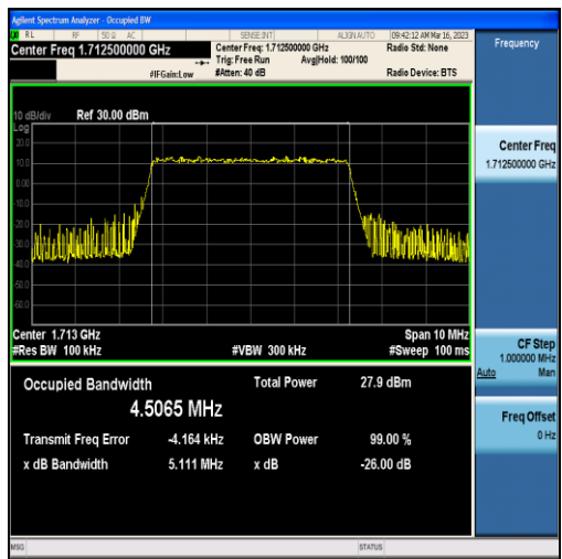
Band4-5MHz-QPSK-19975-25RB#0-4.5065
