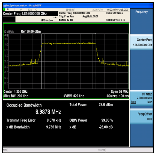
Band2-10MHz-QPSK-18650-50RB#0-8.9878
