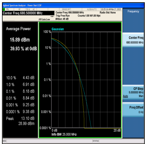
Band71-15MHz-16QAM-133297-75RB#0
