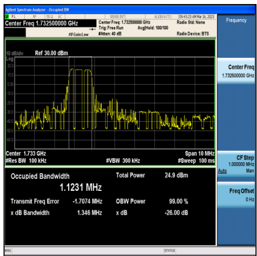
Band4-5MHz-QPSK-20175-25RB#0-1.1231
