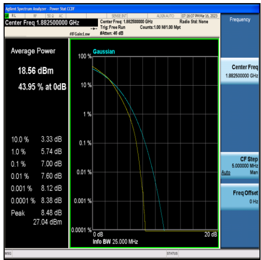
Band25-15MHz-16QAM-26365-75RB#0
