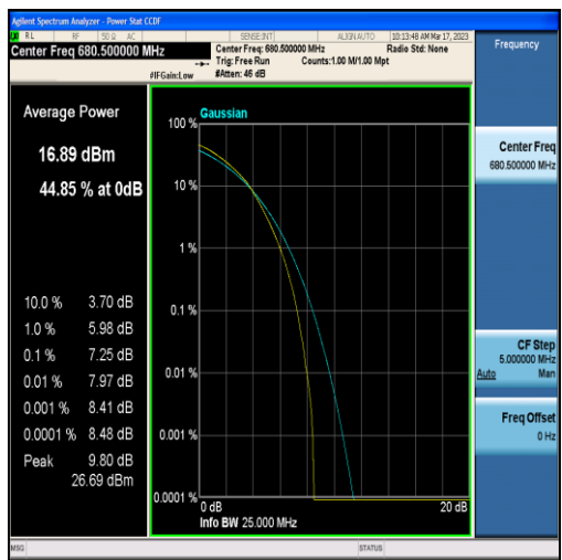
Band71-10MHz-16QAM-133297-50RB#0
