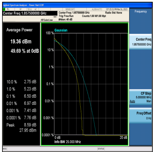
Band25-15MHz-QPSK-26115-75RB#0
