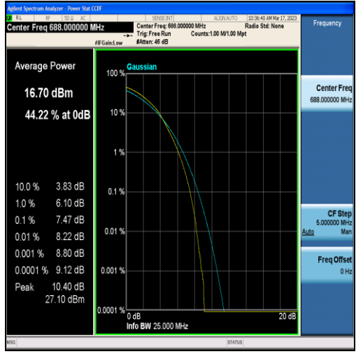
Band71-20MHz-16QAM-133372-100RB#0
