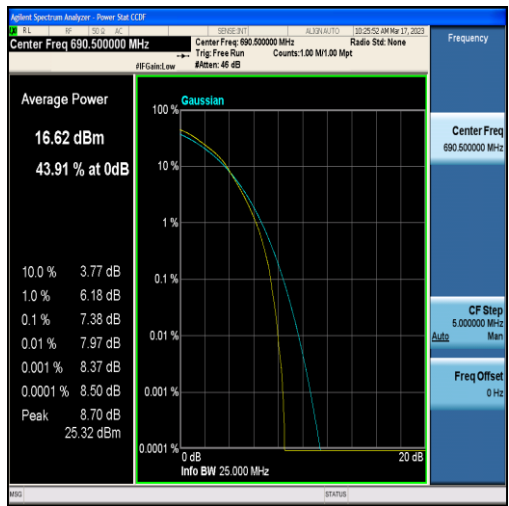
Band71-15MHz-16QAM-133397-75RB#0
