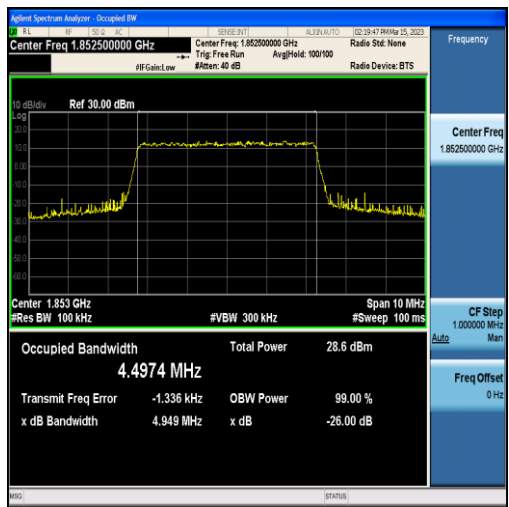
Band2-5MHz-QPSK-18625-25RB#0-4.4974
