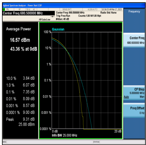
Band71-20MHz-16QAM-133297-100RB#0
