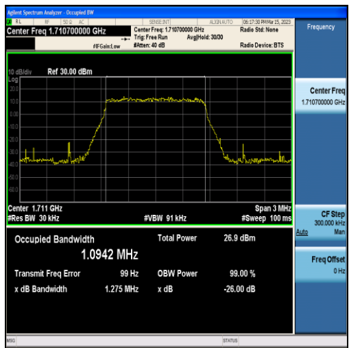
Band4-1.4MHz-QPSK-19957-6RB#0-1.0942
