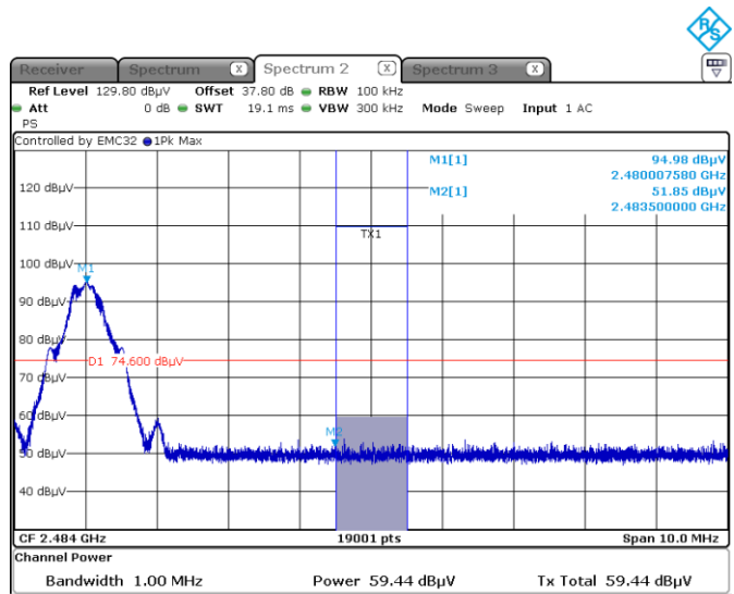
Figure 8.9-2: Radiated Band edge, peak at high channel
