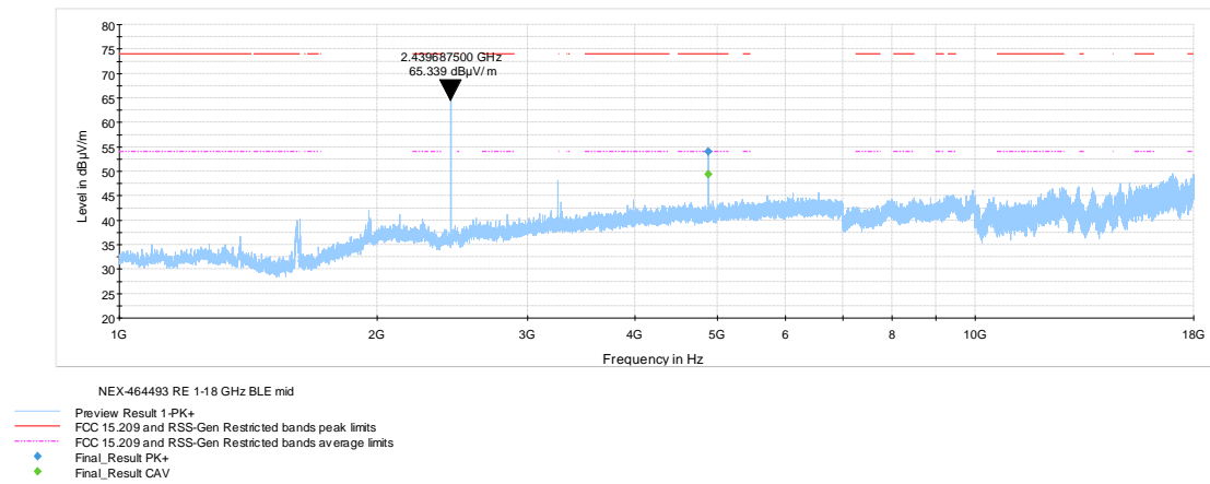
Figure 8.9-14: Radiated spurious emissions 1-18 GHz mid channel
