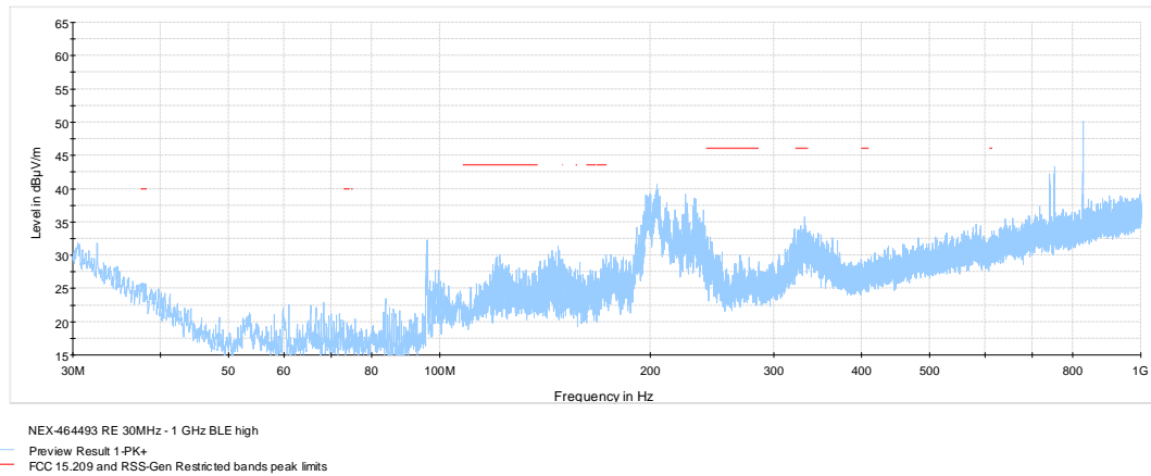
Figure 8.9-16: Radiated spurious emissions below 1 GHz high channel
