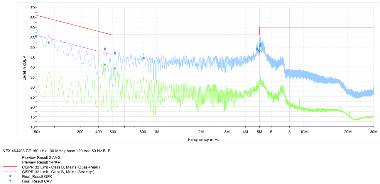
Plot 8.6-1: Conducted emissions on phase line
