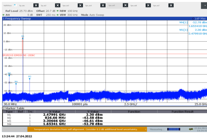
Figure 8.9-7: Conducted spurious emissions on high channel
