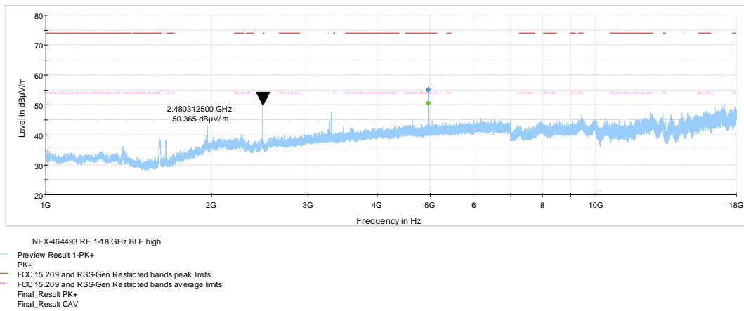
Figure 8.9-17: Radiated spurious emissions 1 -18 GHz high channel
