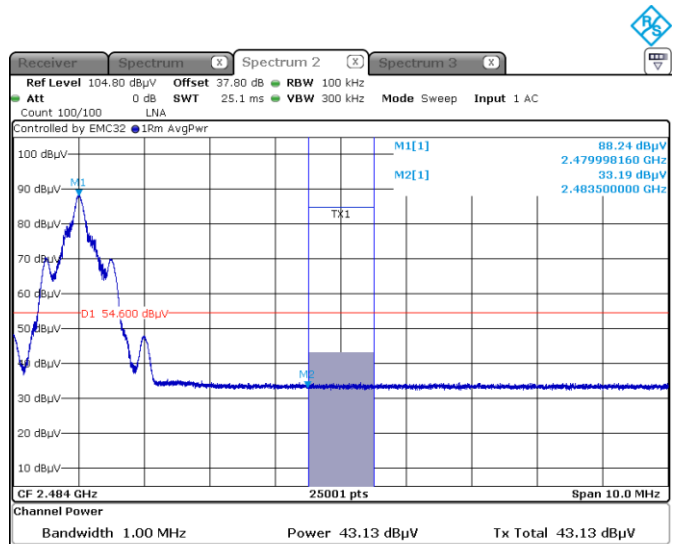
Figure 8.9-4: Radiated Band edge, average at high channel
