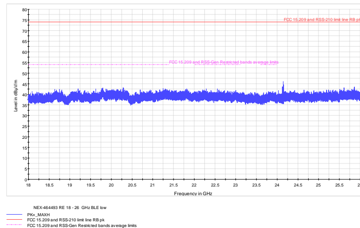
Figure 8.9-12: Radiated spurious emissions 18-26 GHz low channel
