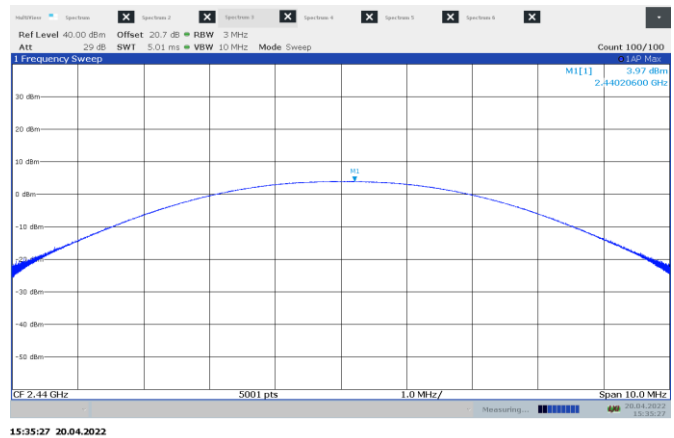
Figure 8.8-2: Output power on mid channel
