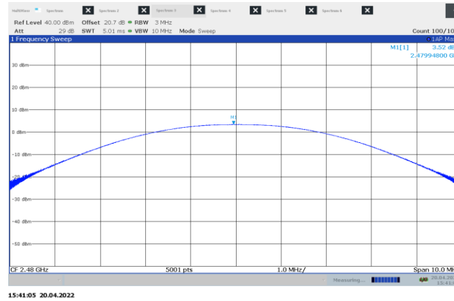
Figure 8.8-3: Output power on high channel
