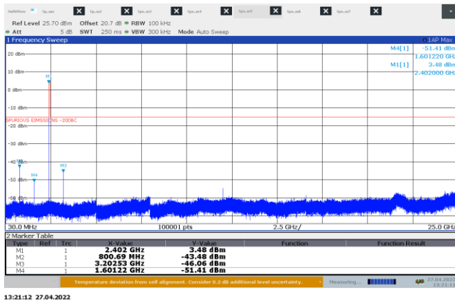
Figure 8.9-5: Conducted spurious emissions on low channel
