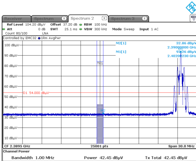
Figure 8.9-3: Radiated Band edge, average at low channel
