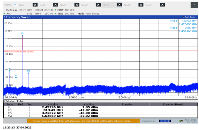
Figure 8.9-6: Conducted spurious emissions on mid channel
