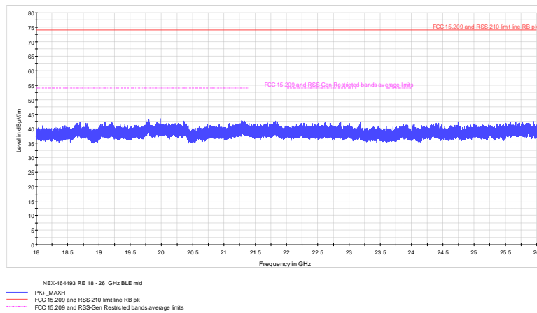
Figure 8.9-15: Radiated spurious emissions 18-26 GHz mid channel
