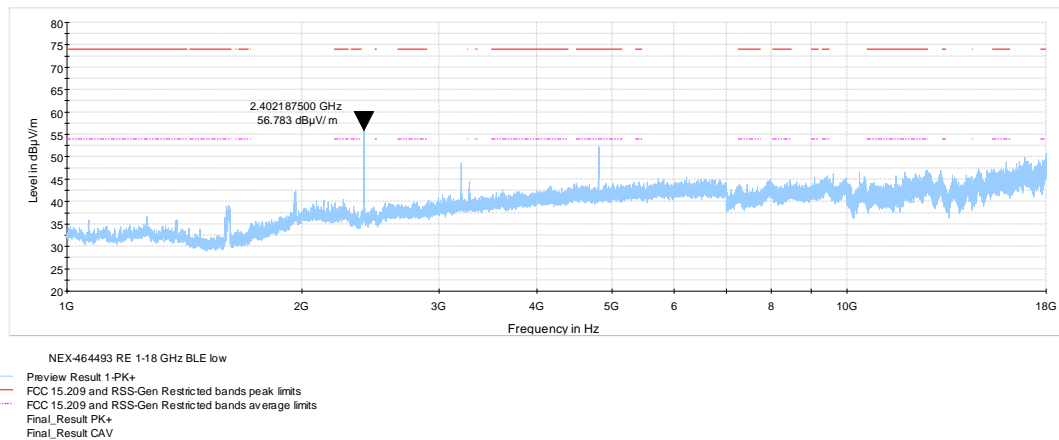
Figure 8.9-11: Radiated spurious emissions 1-18 GHz low channel
