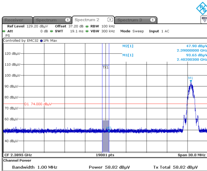
Figure 8.9-1: Radiated Band edge, peak at low channel
