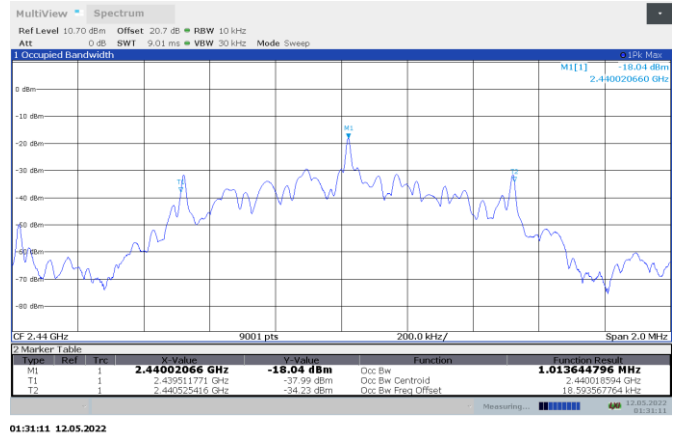
Figure 8.7-2: 99% OBW , sample plot
