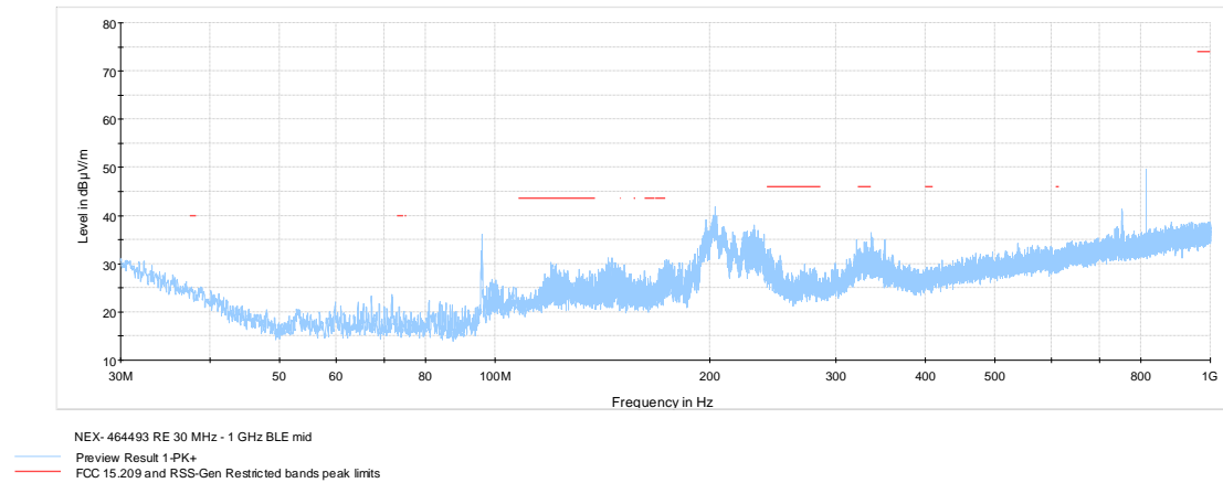
Figure 8.9-13: Radiated spurious emissions below 1 GHz mid channel
