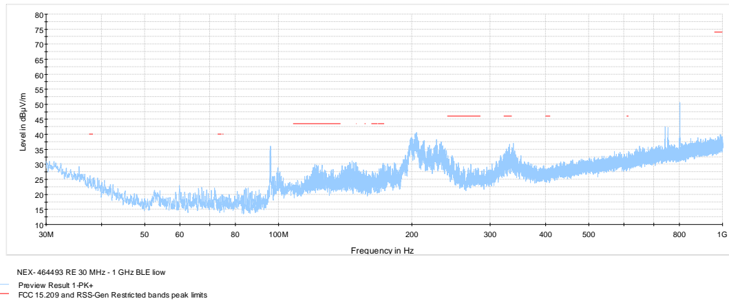
Figure 8.9-10: Radiated spurious emissions below 1 GHz low channel
