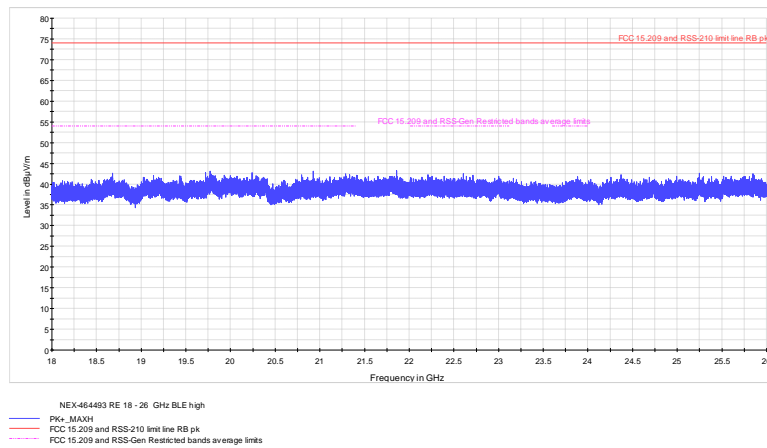
Figure 8.9-18: Radiated spurious emissions 18-26 GHz high channel
