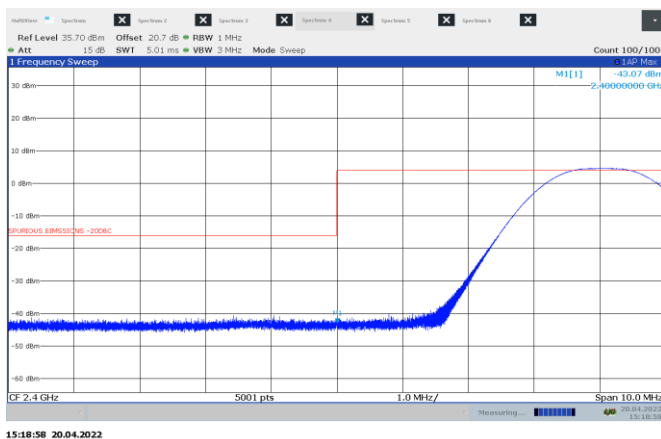
Figure 8.9-8: Conducted Band edge spurious at low channel
