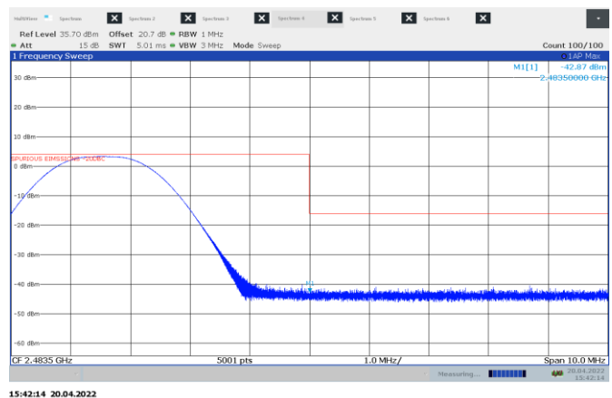
Figure 8.9-9: Conducted Band edge spurious emissions at high channel
