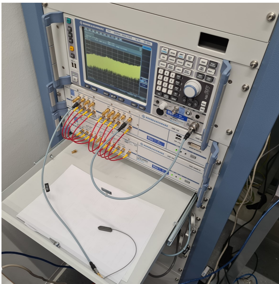
Figure 5: Conducted measurements test setup
