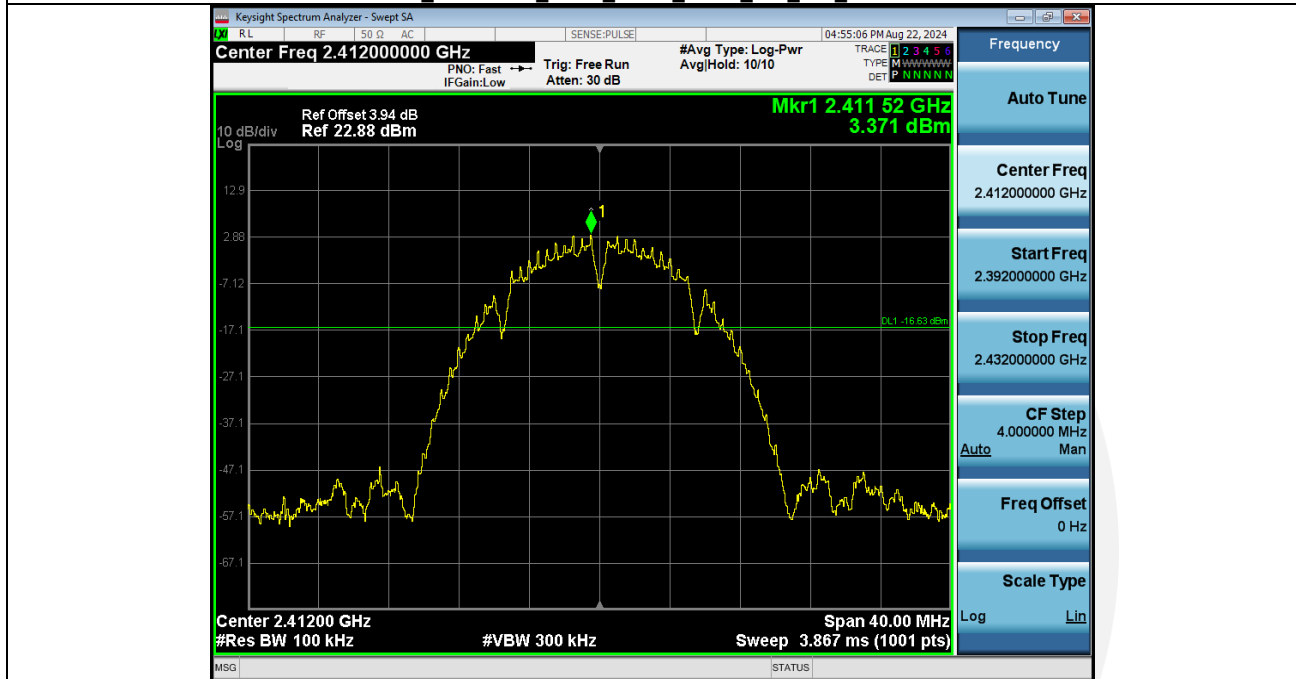
2_Bandedge_NVNT_ANT1_802_11b_2412
