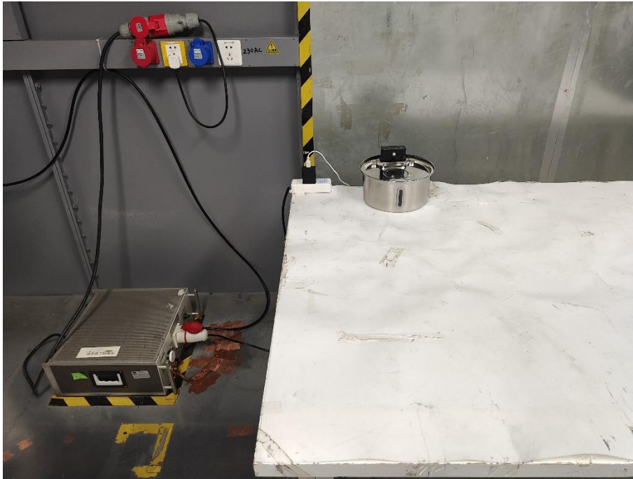
Photographs of the Test Set-up for Power Line Conducted Emission Test
