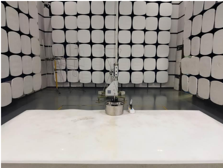
Photographs of the Test Set-up for Radiated Emissions(30-1000MHz)
