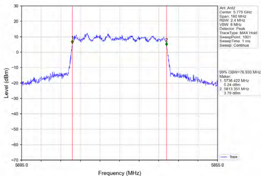
802.11ac(VHT80)_MCH_5775MHz_Ant2_NTNV
