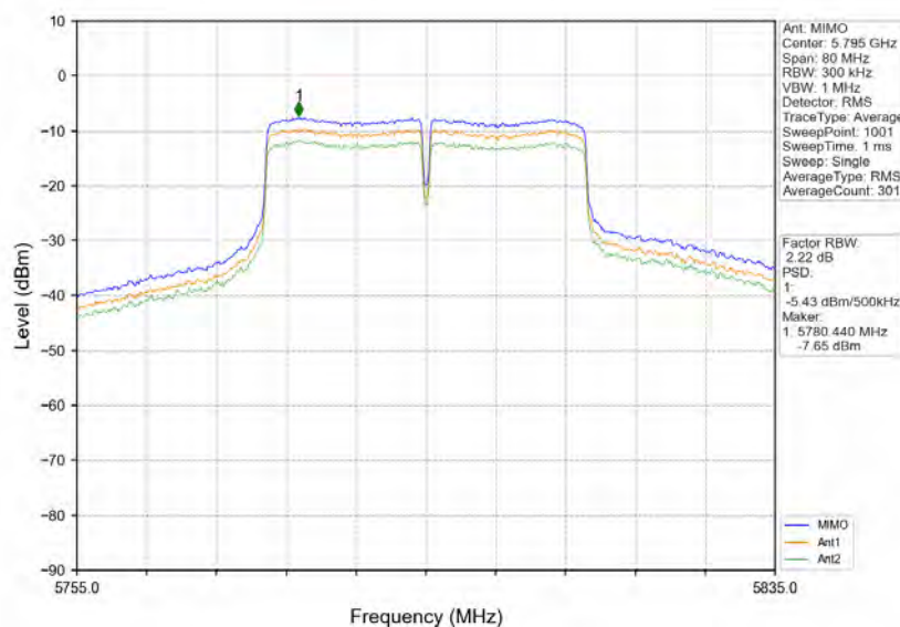
802.11ac(VHT40)_HCH_5795MHz_MIMO_NTNV
