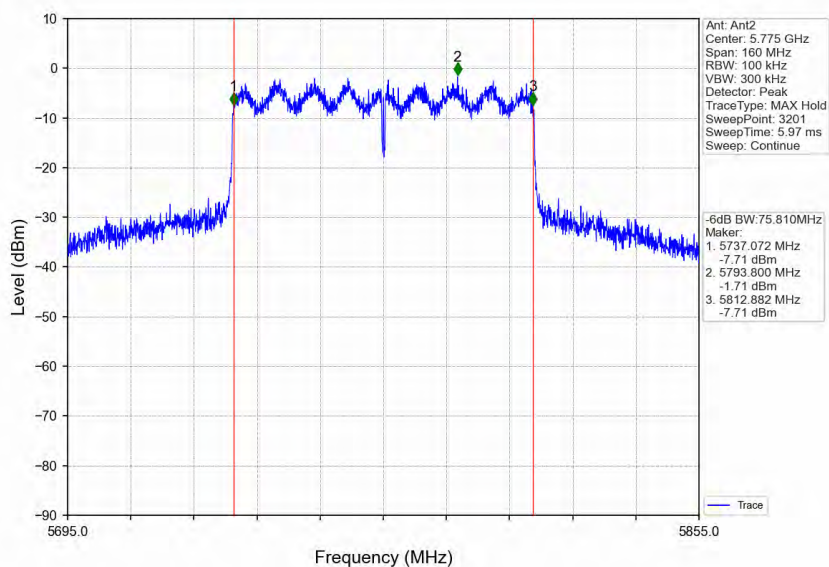
802.11ac(VHT80)_MCH_5775MHz_Ant2_NTNV
