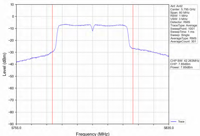
802.11ac(VHT40)_HCH_5795MHz_Ant2_NTNV
