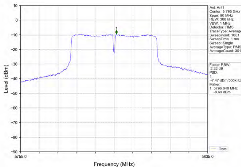
802.11ac(VHT40)_HCH_5795MHz_Ant1_NTNV
