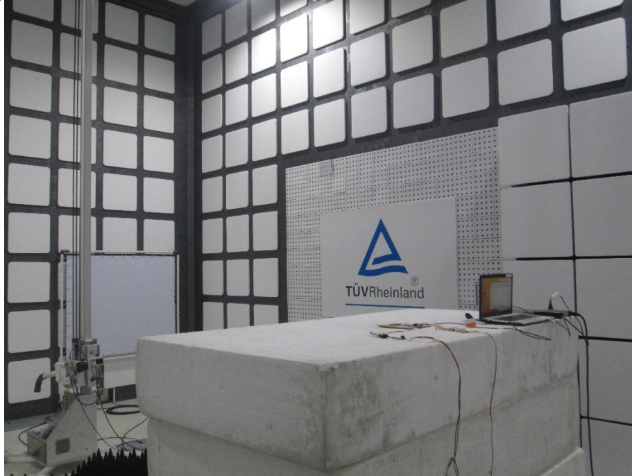
Photograph 9: Test Setup for Spurious Emissions (Back View 2)
