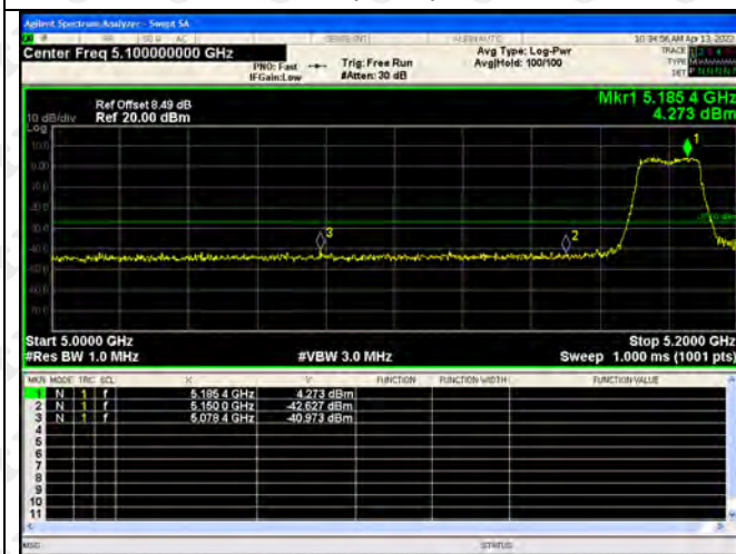
802.11n(HT40)-5190
