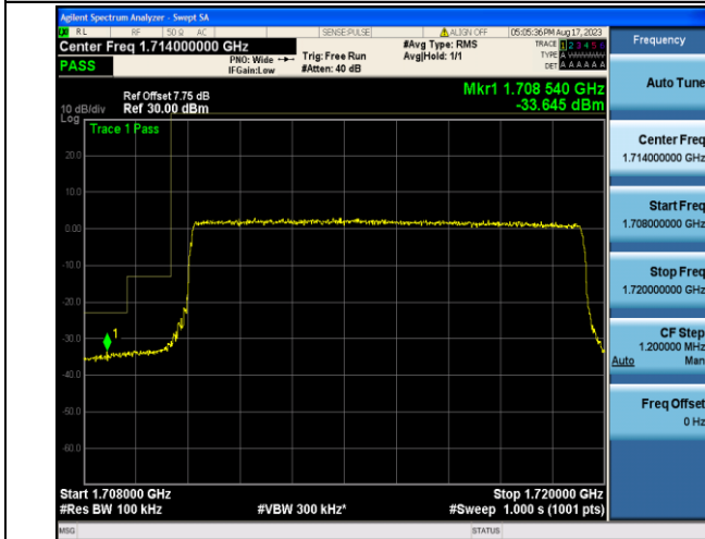
Band4_10MHz_QPSK_20000_50RB#0
