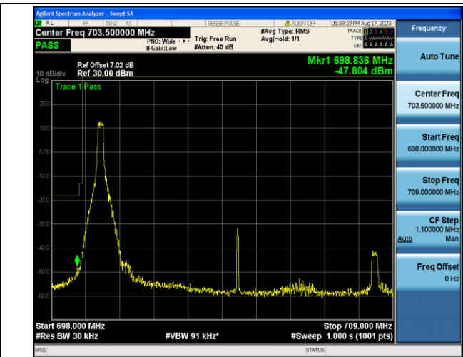
Band12_10MHz_16QAM_23060_1RB#0
