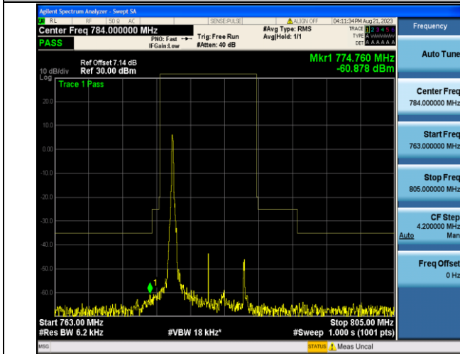
Band13_10MHz_QPSK_23230_1RB#0
