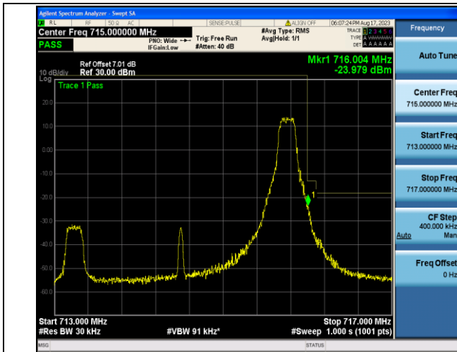
Band12_3MHz_QPSK_23165_1RB#14
