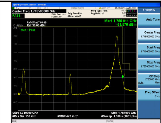
Band4_15MHz_16QAM_20325_1RB#74
