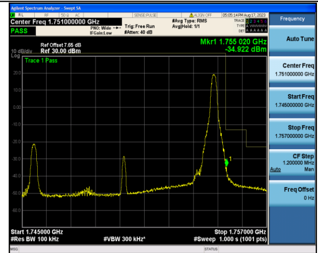
Band4_10MHz_16QAM_20350_1RB#49
