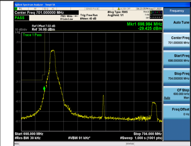
Band12_5MHz_16QAM_23035_1RB#0
