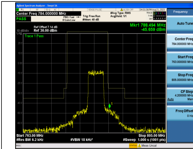
Band13_5MHz_QPSK_23255_25RB#0
