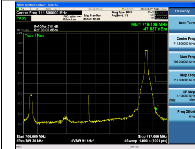
Band12_10MHz_QPSK_23130_1RB#49
