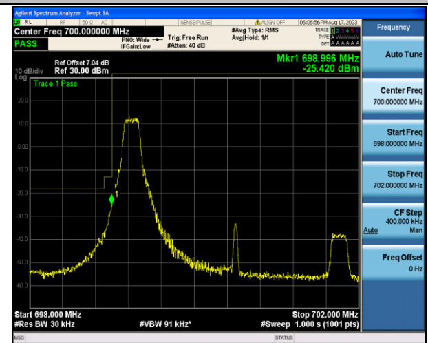
Band12_3MHz_16QAM_23025_1RB#0
