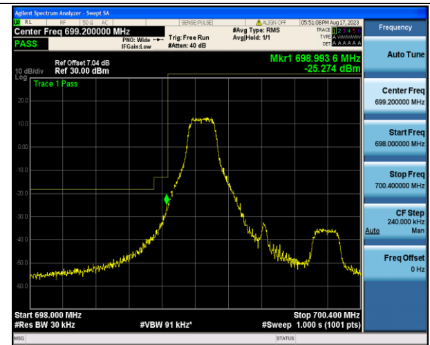
Band12_1.4MHz_16QAM_23017_1RB#0
