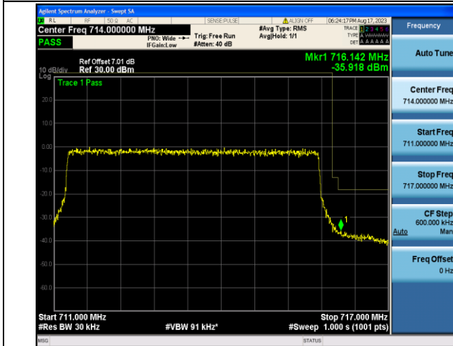
Band12_5MHz_QPSK_23155_25RB#0
