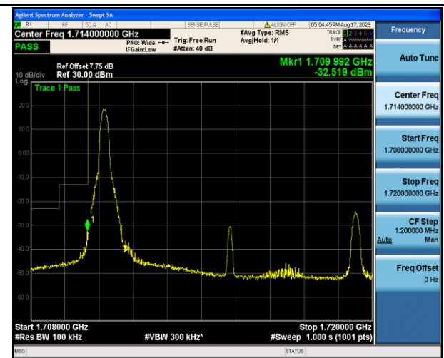
Band4_10MHz_16QAM_20000_1RB#0
