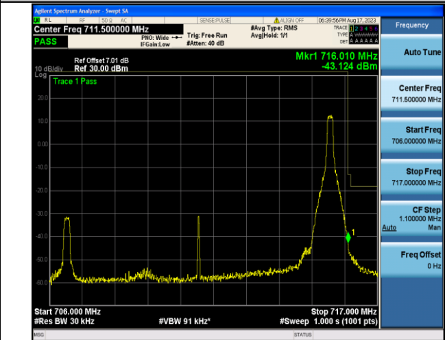
Band12_10MHz_16QAM_23130_1RB#49
