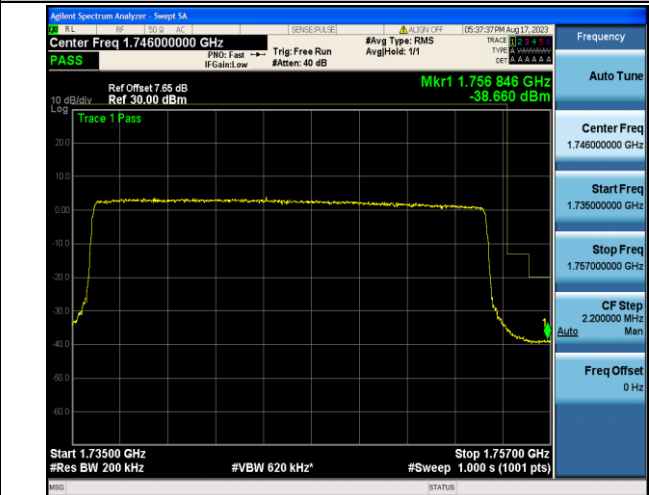
Band4_20MHz_QPSK_20300_100RB#0
