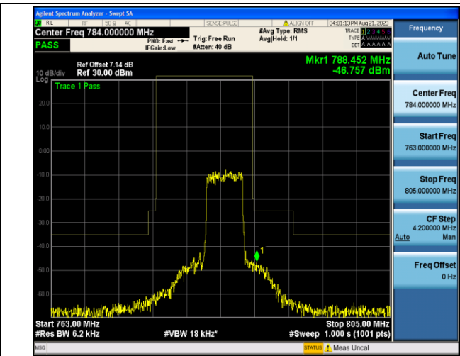
Band13_5MHz_16QAM_23255_25RB#0
