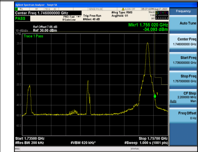
Band4_20MHz_16QAM_20300_1RB#99
