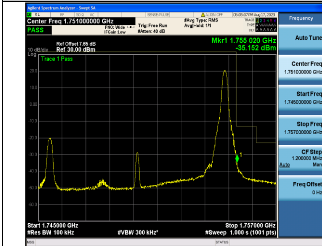
Band4_10MHz_QPSK_20350_1RB#49
