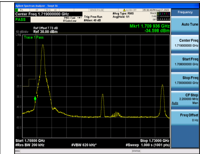
Band4_20MHz_16QAM_20050_1RB#0
