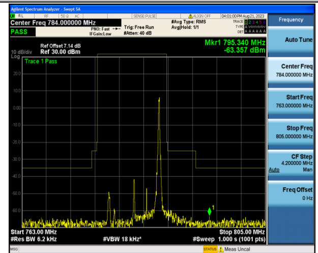
Band13_5MHz_16QAM_23255_1RB#24
