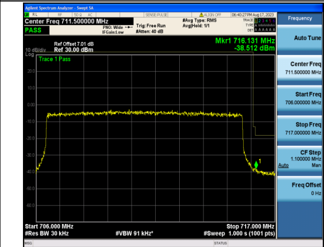
Band12_10MHz_QPSK_23130_50RB#0
