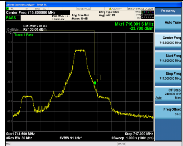
Band12_1.4MHz_16QAM_23173_1RB#5
