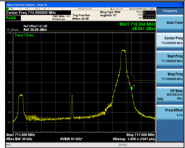
Band12_5MHz_16QAM_23155_1RB#24
