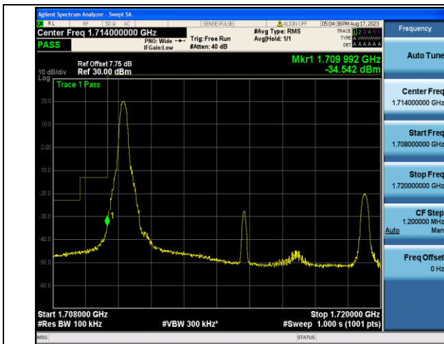
Band4_10MHz_QPSK_20000_1RB#0
