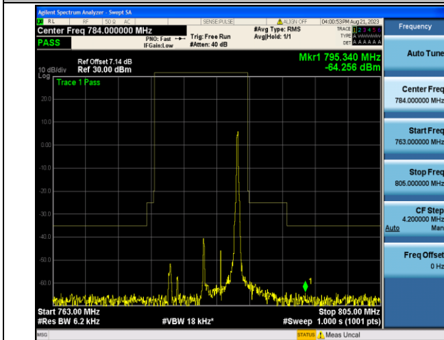
Band13_5MHz_QPSK_23255_1RB#24
