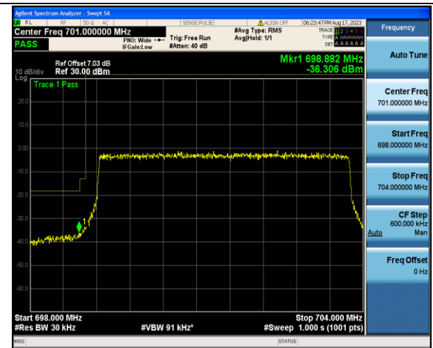
Band12_5MHz_16QAM_23035_25RB#0
