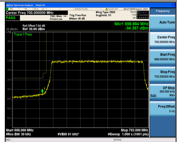
Band12_3MHz_16QAM_23025_15RB#0
