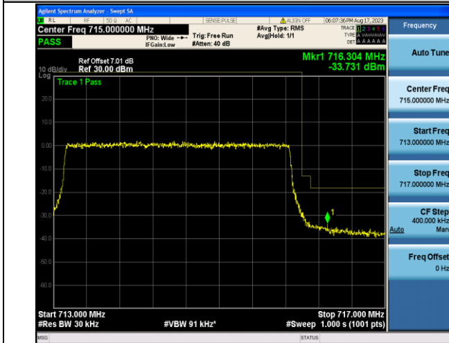
Band12_3MHz_QPSK_23165_15RB#0
