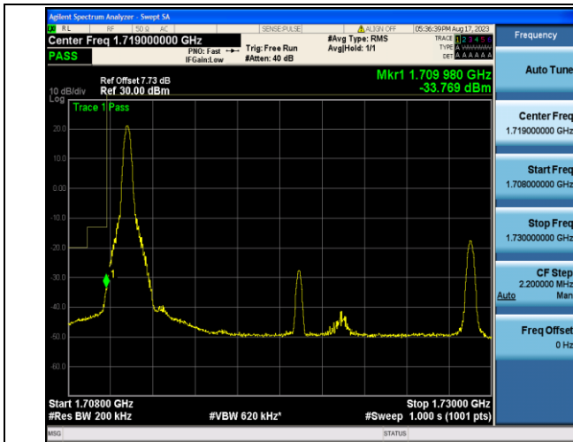
Band4_20MHz_QPSK_20050_1RB#0
