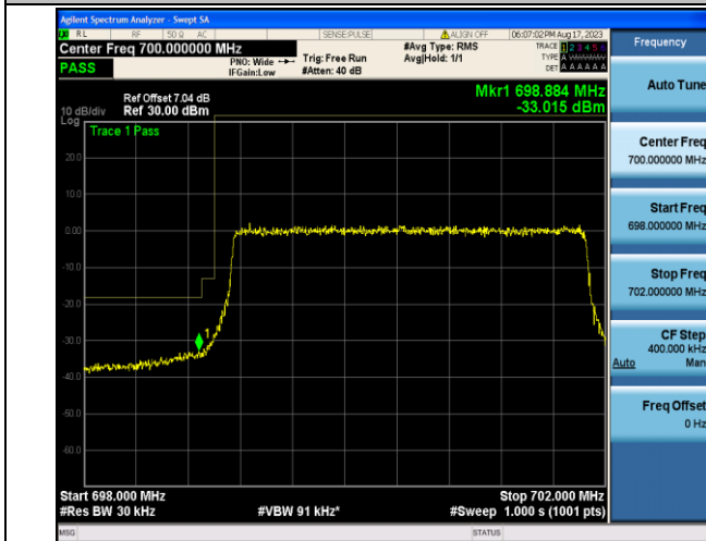
Band12_3MHz_QPSK_23025_15RB#0
