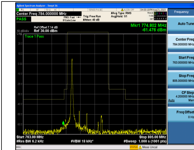
Band13_5MHz_QPSK_23205_1RB#0
