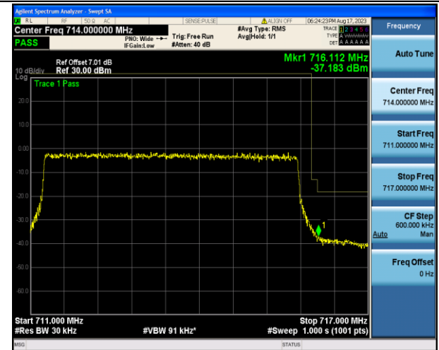
Band12_5MHz_16QAM_23155_25RB#0
