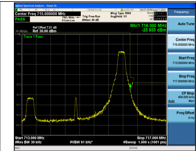
Band12_3MHz_16QAM_23165_1RB#14
