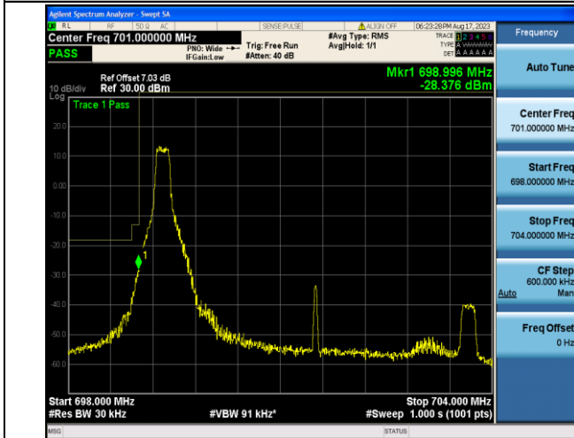
Band12_5MHz_QPSK_23035_1RB#0
