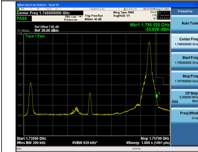
Band4_20MHz_QPSK_20300_1RB#99
