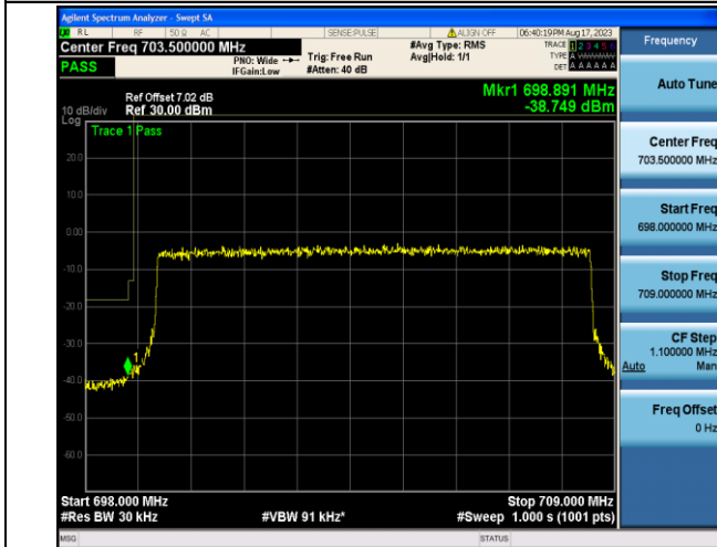
Band12_10MHz_QPSK_23060_50RB#0
