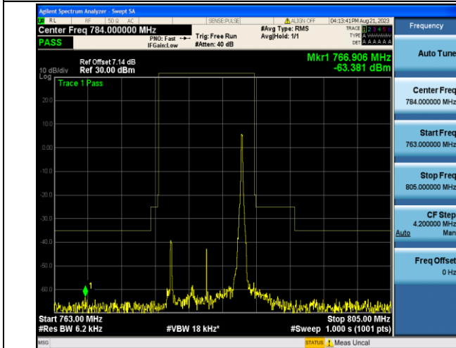
Band13_10MHz_QPSK_23230_1RB#49
