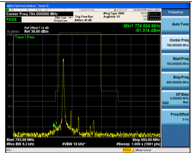
Band13_5MHz_16QAM_23205_1RB#0
