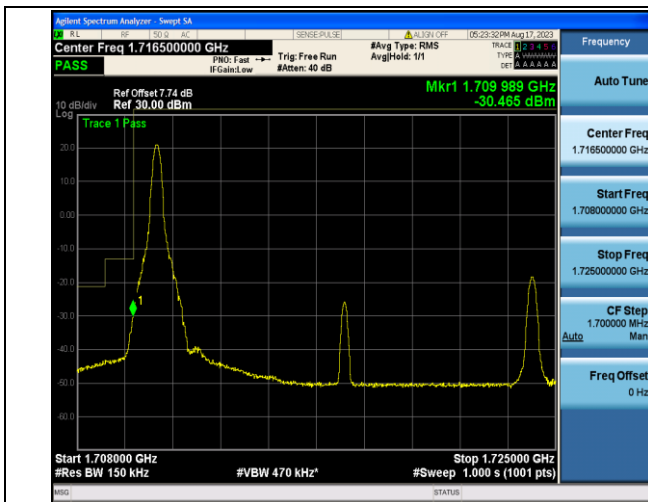
Band4_15MHz_QPSK_20025_1RB#0
