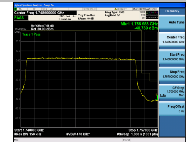
Band4_15MHz_QPSK_20325_75RB#0
