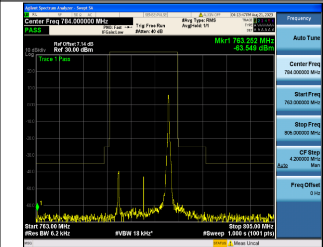
Band13_10MHz_16QAM_23230_1RB#49
