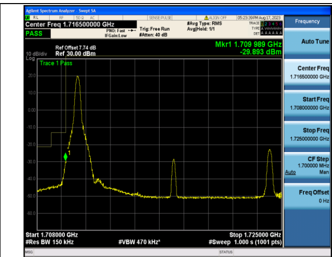
Band4_15MHz_16QAM_20025_1RB#0
