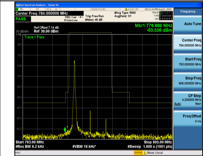
Band13_10MHz_16QAM_23230_1RB#0
