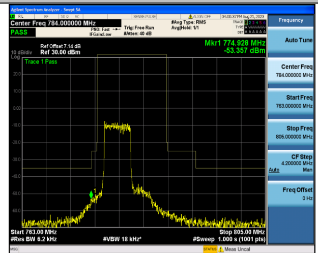
Band13_5MHz_16QAM_23205_25RB#0
