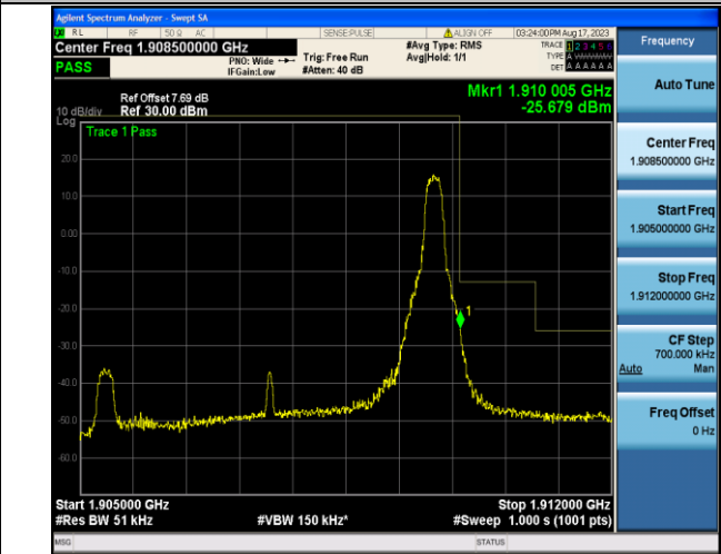
Band2_5MHz_16QAM_19175_1RB#24
