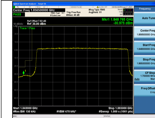
Band2_15MHz_QPSK_18675_75RB#0
