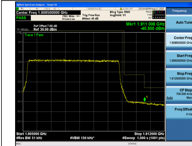
Band2_5MHz_QPSK_19175_25RB#0
