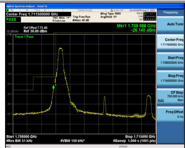
Band4_5MHz_16QAM_19975_1RB#0
