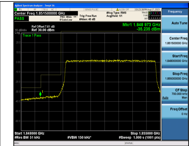
Band2_5MHz_16QAM_18625_25RB#0
