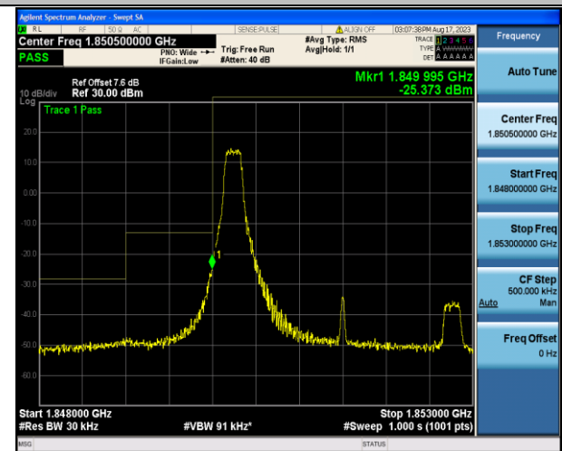
Band2_3MHz_16QAM_18615_1RB#0
