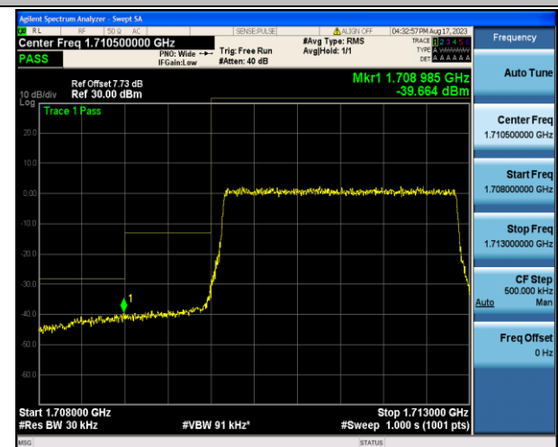
Band4_3MHz_16QAM_19965_15RB#0
