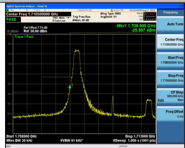
Band4_3MHz_16QAM_19965_1RB#0
