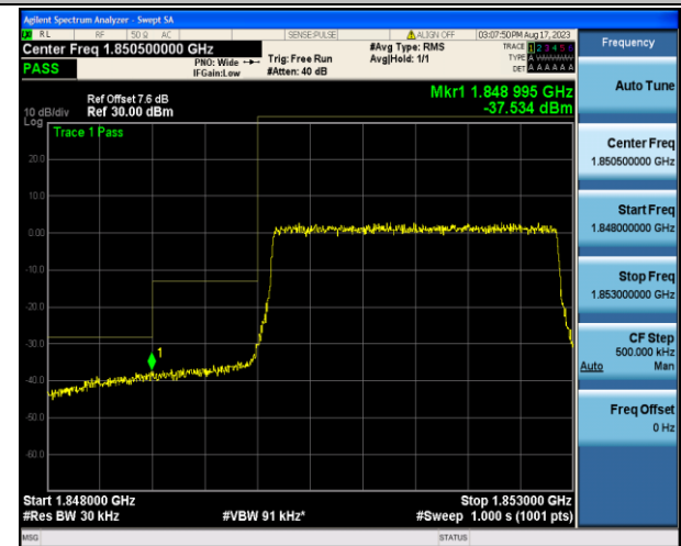
Band2_3MHz_16QAM_18615_15RB#0
