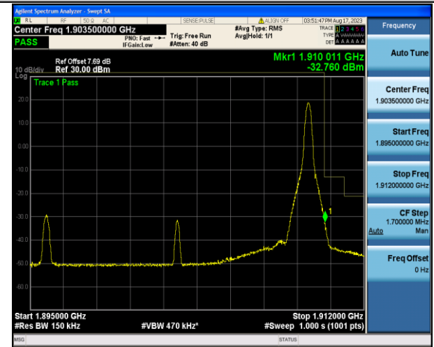
Band2_15MHz_16QAM_19125_1RB#74
