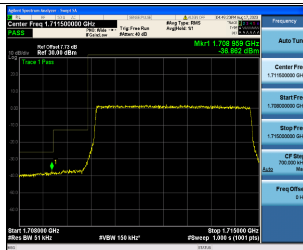
Band4 5MHz 16QAM 19975 25RB#0
