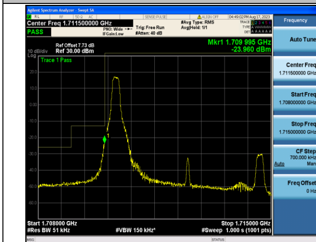
Band4_5MHz_QPSK_19975_1RB#0
