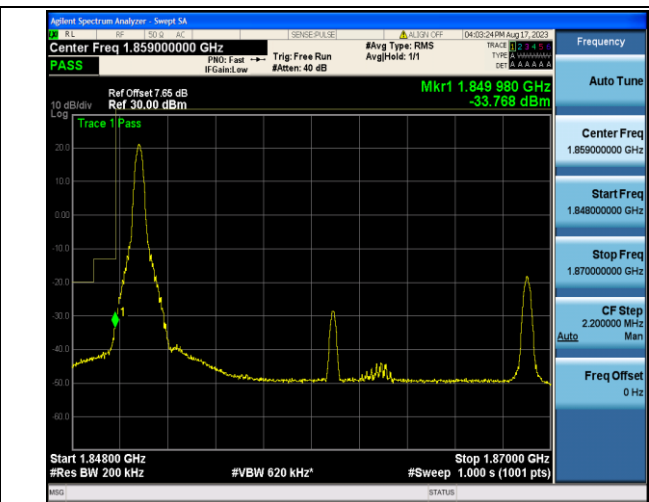
Band2_20MHz_16QAM_18700_1RB#0
