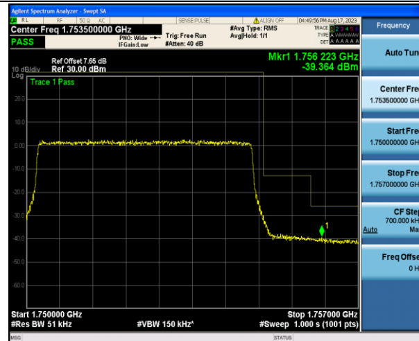
Band4_5MHz_16QAM_20375_25RB#0
