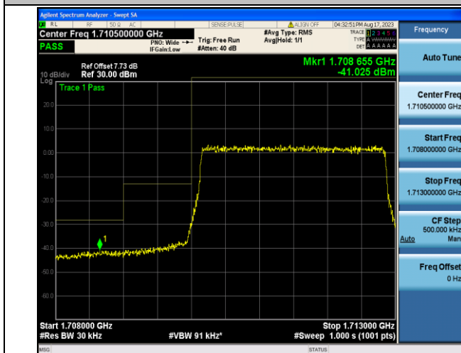
Band4_3MHz_QPSK_19965_15RB#0
