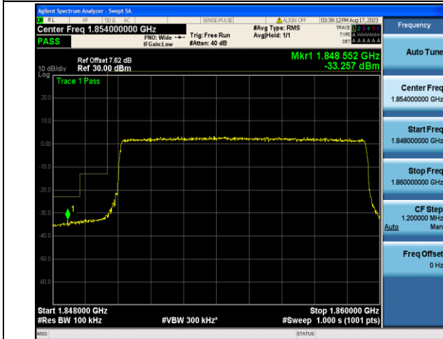
Band2_10MHz_QPSK_18650_50RB#0
