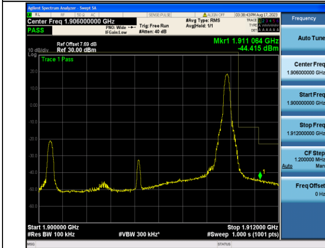
Band2_10MHz_QPSK_19150_1RB#49
