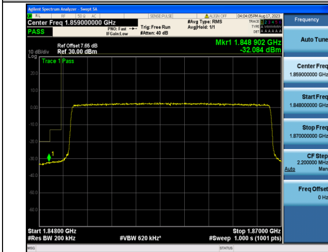
Band2_20MHz_QPSK_18700_100RB#0
