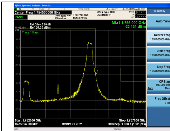
Band4_3MHz_QPSK_20385_1RB#14
