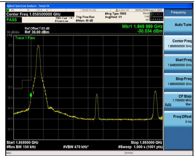
Band2_15MHz_16QAM_18675_1RB#0
