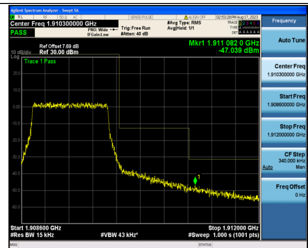
Band2_1.4MHz_16QAM_19193_6RB#0
