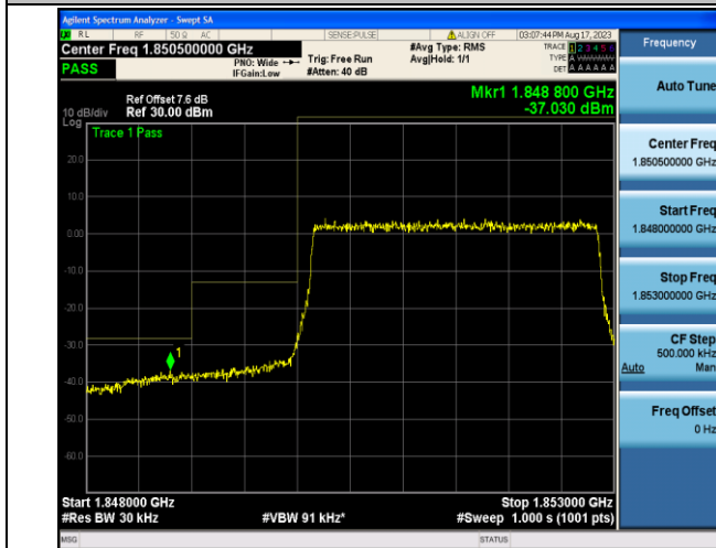
Band2_3MHz_QPSK_18615_15RB#0
