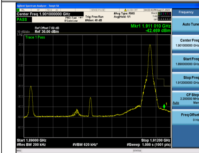
Band2_20MHz_QPSK_19100_1RB#99
