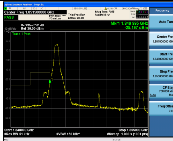
Band2 5MHz 16QAM 18625 1RB#0
