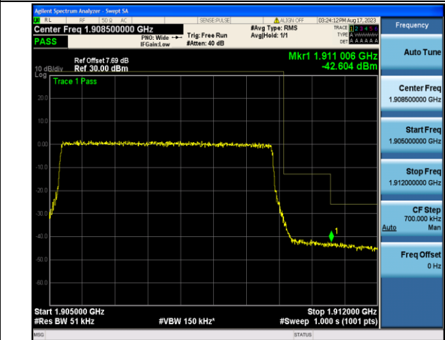
Band2_5MHz_16QAM_19175_25RB#0
