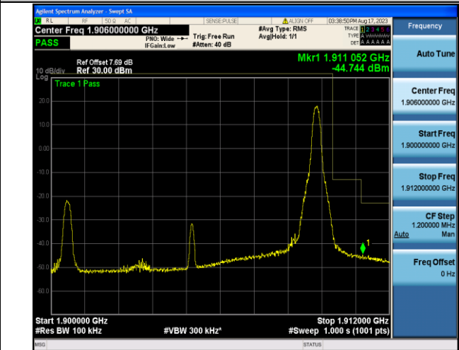
Band2_10MHz_16QAM_19150_1RB#49
