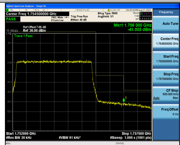
Band4_3MHz_16QAM_20385_15RB#0
