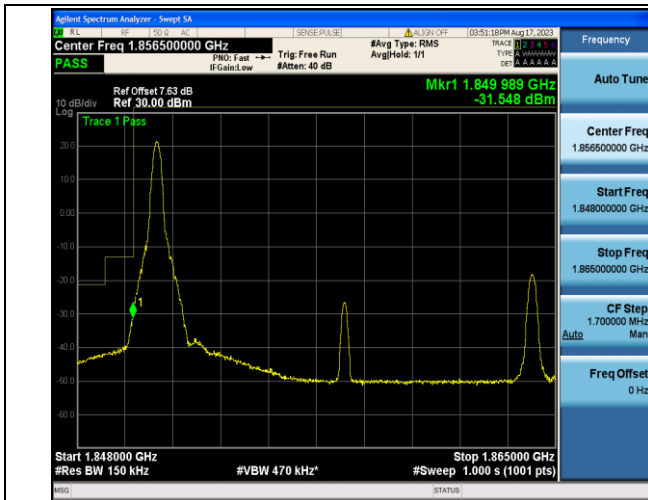
Band2_15MHz_QPSK_18675_1RB#0
