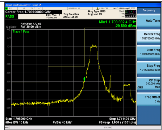
Band4_1.4MHz_16QAM_19957_1RB#0
