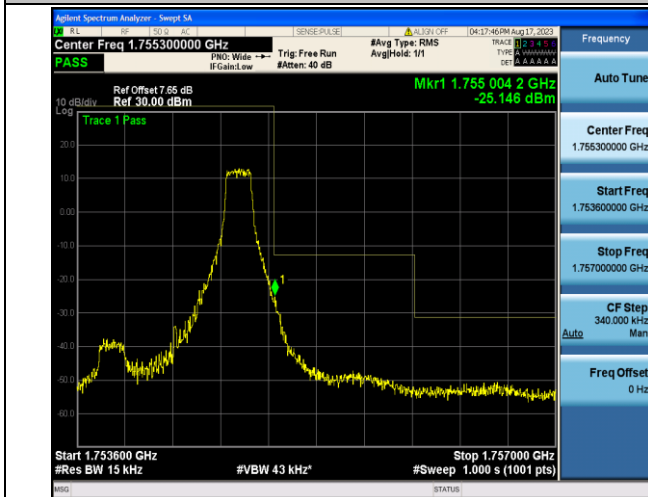
Band4_1.4MHz_QPSK_20393_1RB#5
