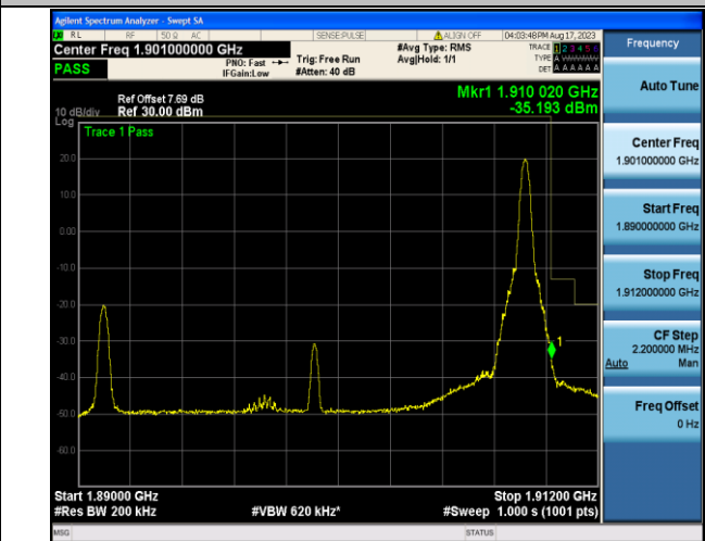
Band2_20MHz_16QAM_19100_1RB#99
