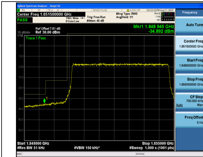
Band2_5MHz_QPSK_18625_25RB#0
