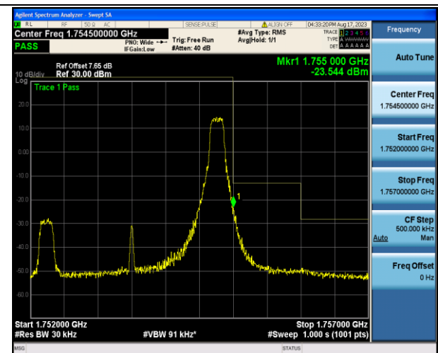
Band4_3MHz_16QAM_20385_1RB#14
