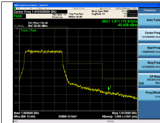
Band2_1.4MHz_QPSK_19193_6RB#0
