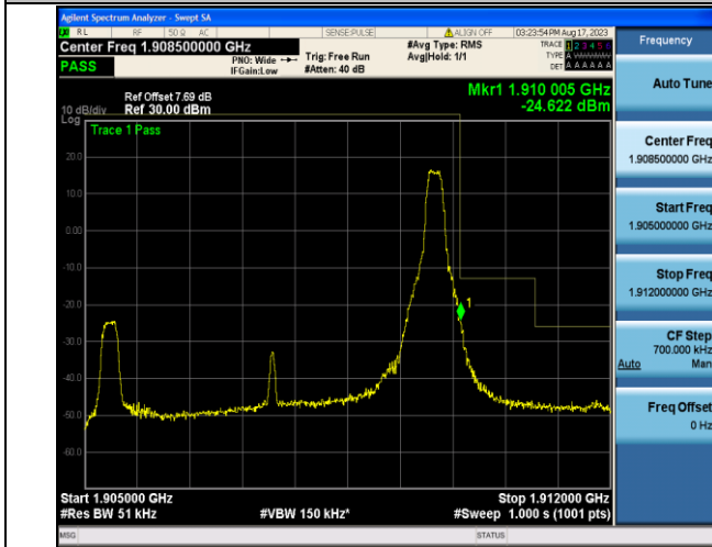
Band2_5MHz_QPSK_19175_1RB#24
