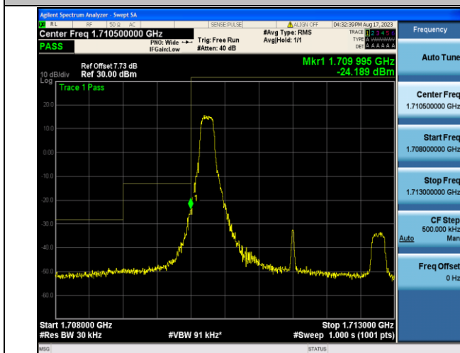
Band4_3MHz_QPSK_19965_1RB#0
