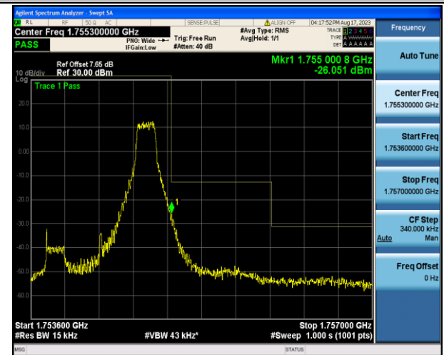
Band4_1.4MHz_16QAM_20393_1RB#5
