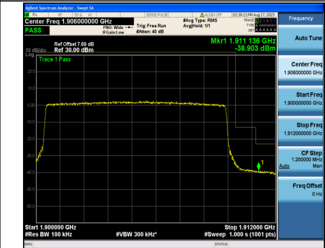
Band2_10MHz_QPSK_19150_50RB#0
