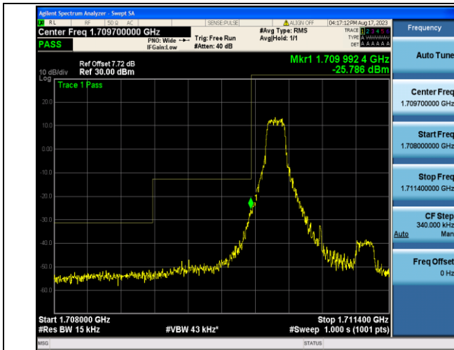
Band4_1.4MHz_QPSK_19957_1RB#0
