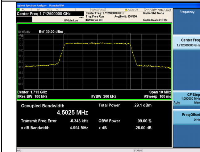
Band4-5MHz-16QAM-19975-25RB#0-PASS
