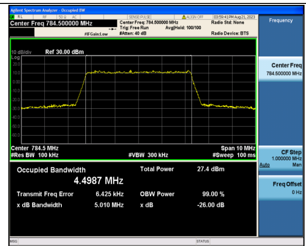
Band13-5MHz-QPSK-23255-25RB#0-PASS
