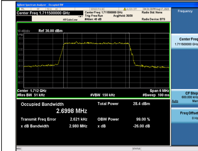
Band4-3MHz-16QAM-19965-15RB#0-PASS
