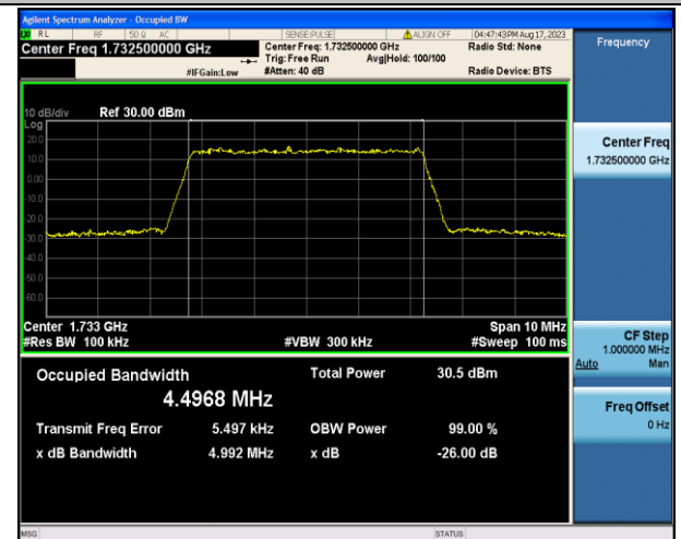
Band4-5MHz-QPSK-20175-25RB#0-PASS
