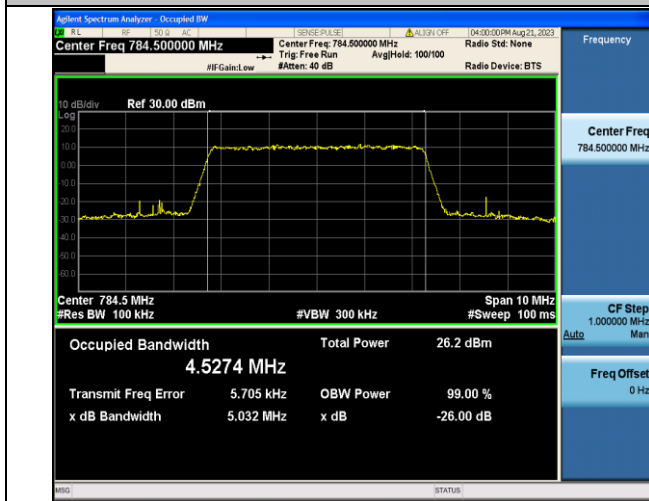
Band13-5MHz-16QAM-23255-25RB#0-PASS
