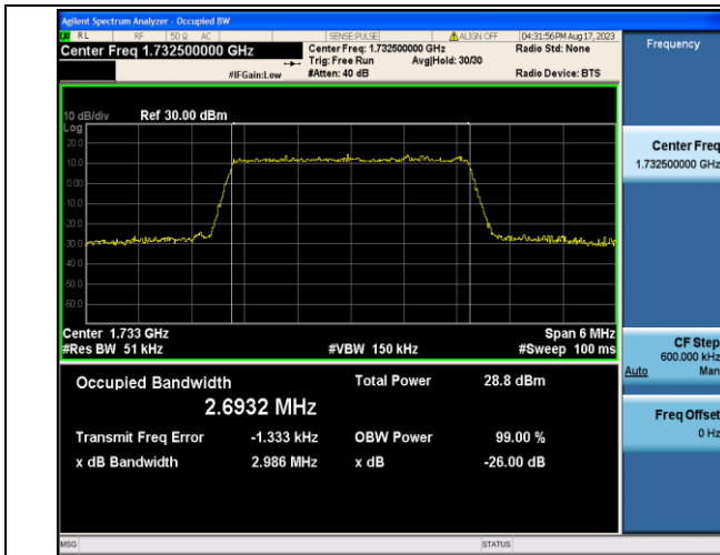
Band4-3MHz-16QAM-20175-15RB#0-PASS
