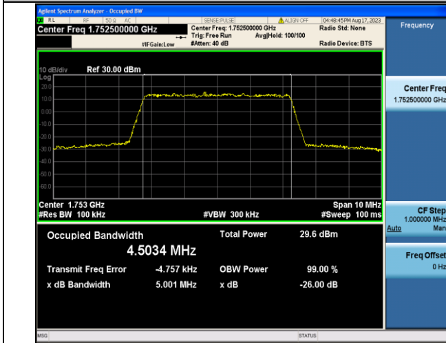
Band4-5MHz-16QAM-20375-25RB#0-PASS
