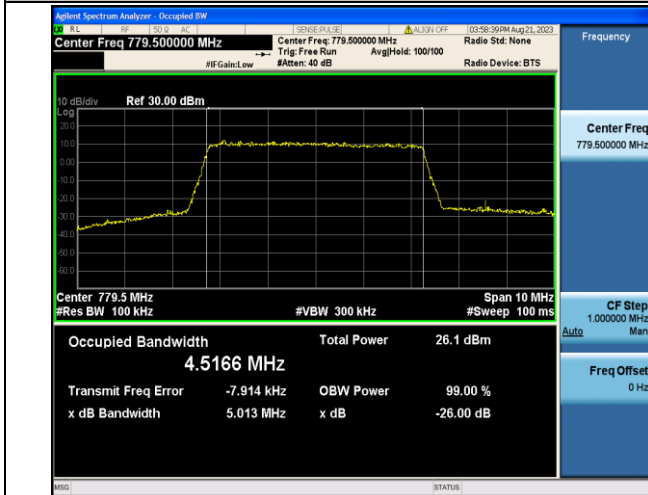
Band13-5MHz-16QAM-23205-25RB#0-PASS
