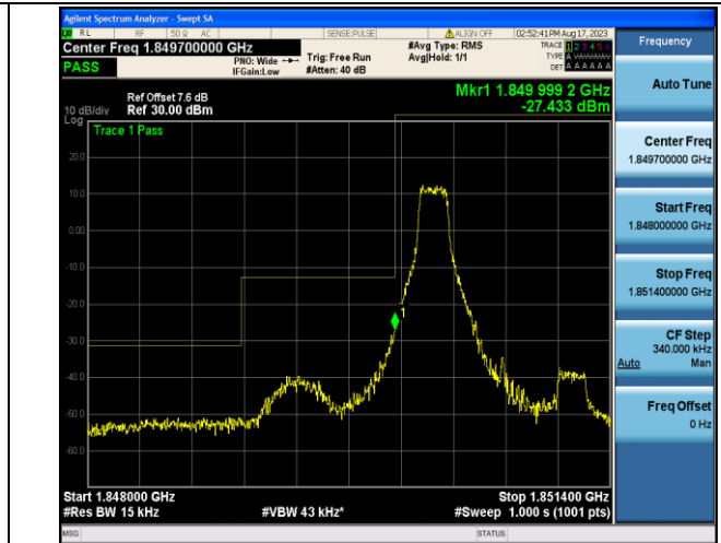
Band2_1.4MHz_16QAM_18607_1RB#0
