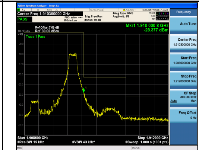
Band2_1.4MHz_16QAM_19193_1RB#5
