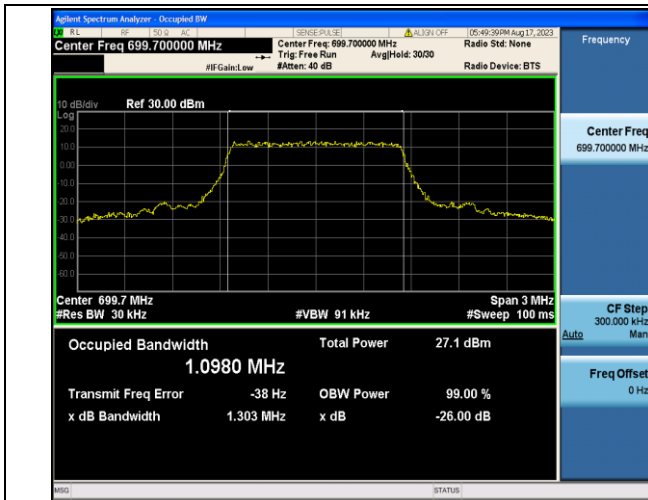
Band12-1.4MHz-QPSK-23017-6RB#0-PASS
