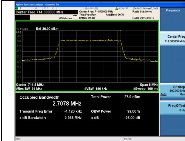
Band12-3MHz-QPSK-23165-15RB#0-PASS
