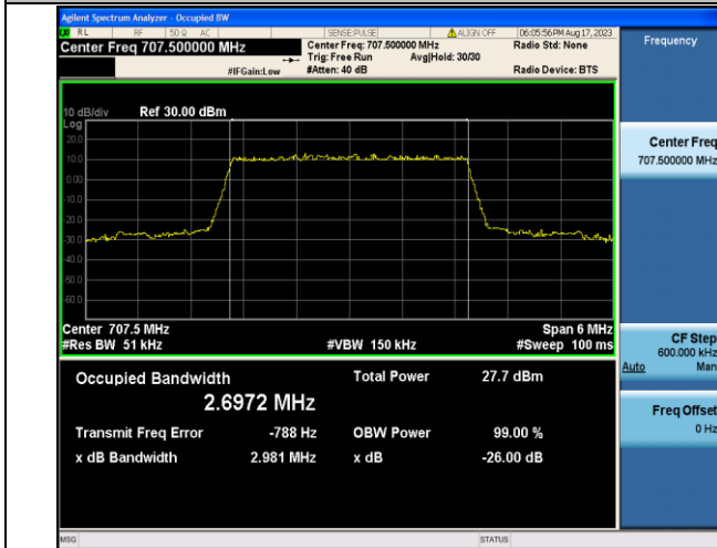
Band12-3MHz-QPSK-23095-15RB#0-PASS
