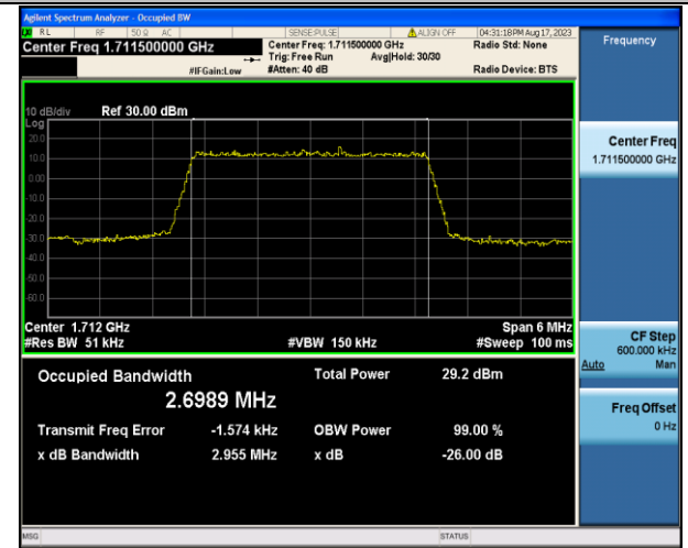
Band4-3MHz-QPSK-19965-15RB#0-PASS
