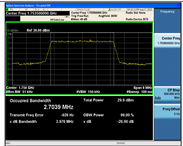
Band4-3MHz-QPSK-20385-15RB#0-PASS
