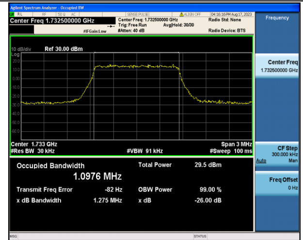
Band4-1.4MHz-QPSK-20175-6RB#0-PASS
