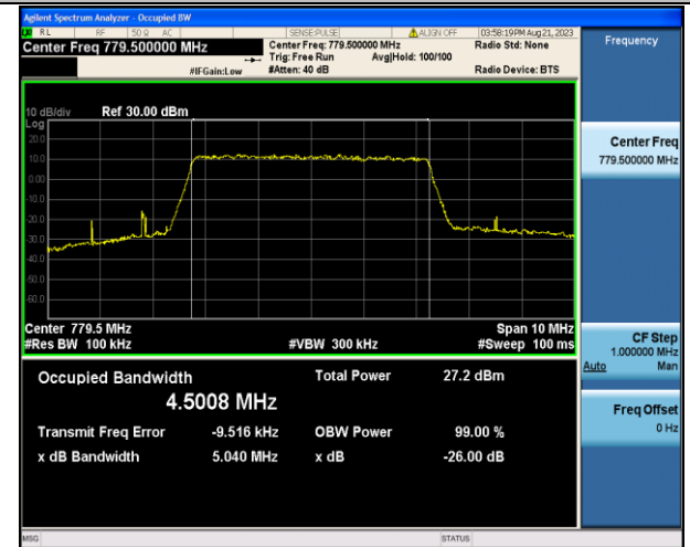
Band13-5MHz-QPSK-23205-25RB#0-PASS
