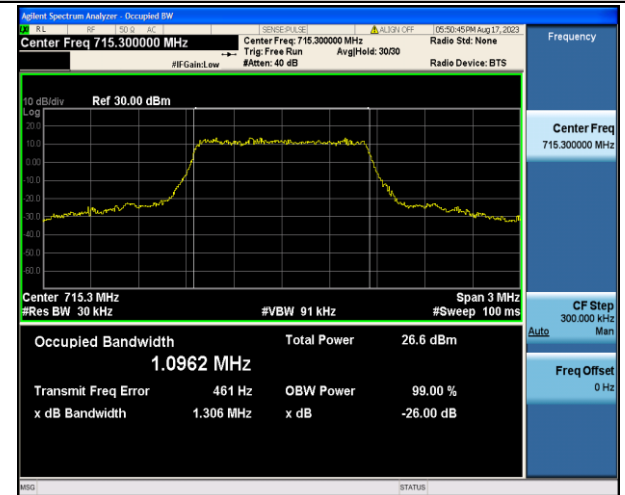
Band12-1.4MHz-16QAM-23173-6RB#0-PASS
