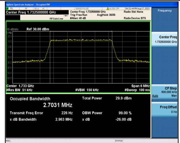
Band4-3MHz-QPSK-20175-15RB#0-PASS
