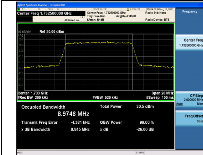
Band4-10MHz-QPSK-20175-50RB#0-PASS
