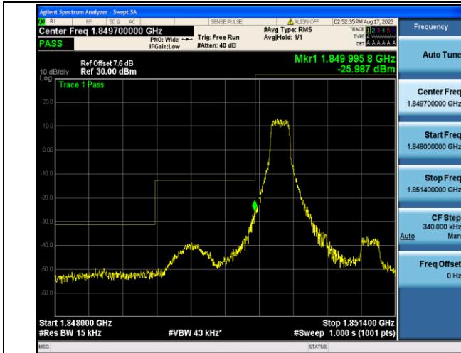
Band2_1.4MHz_QPSK_18607_1RB#0
