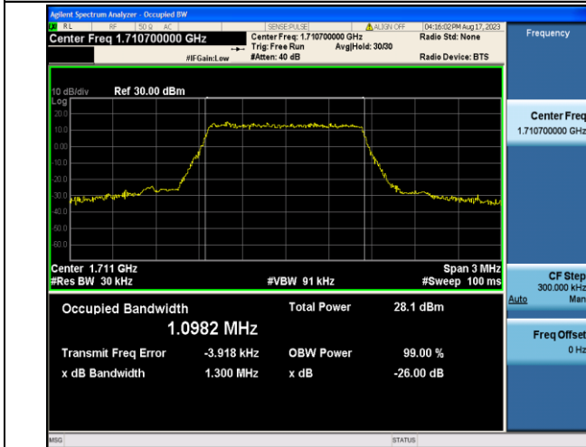
Band4-1.4MHz-16QAM-19957-6RB#0-PASS
