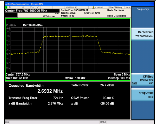
Band12-3MHz-16QAM-23095-15RB#0-PASS
