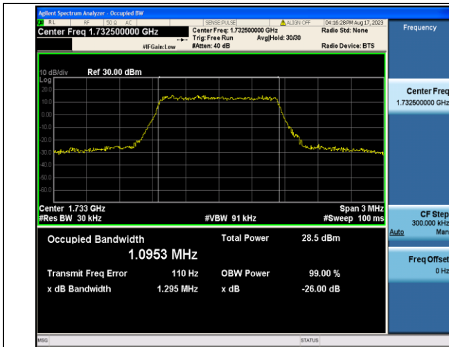
Band4-1.4MHz-16QAM-20175-6RB#0-PASS
