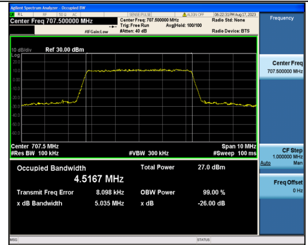
Band12-5MHz-16QAM-23095-25RB#0-PASS
