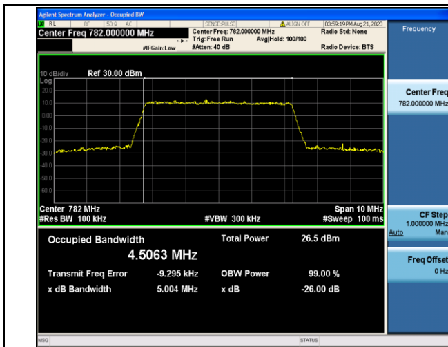
Band13-5MHz-16QAM-23230-25RB#0-PASS
