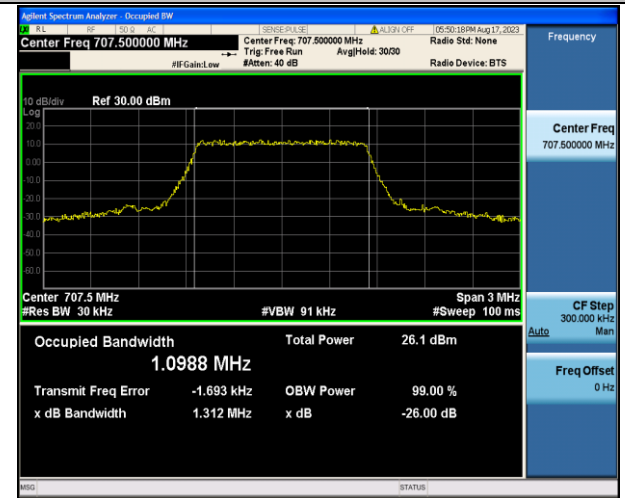
Band12-1.4MHz-16QAM-23095-6RB#0-PASS
