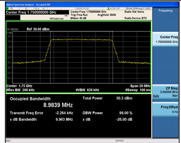
Band4-10MHz-QPSK-20350-50RB#0-PASS
