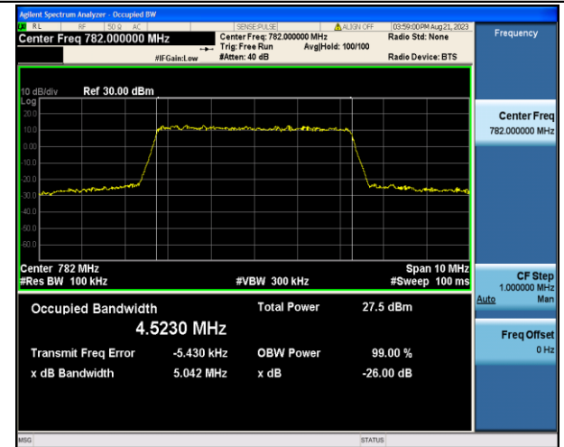
Band13-5MHz-QPSK-23230-25RB#0-PASS
