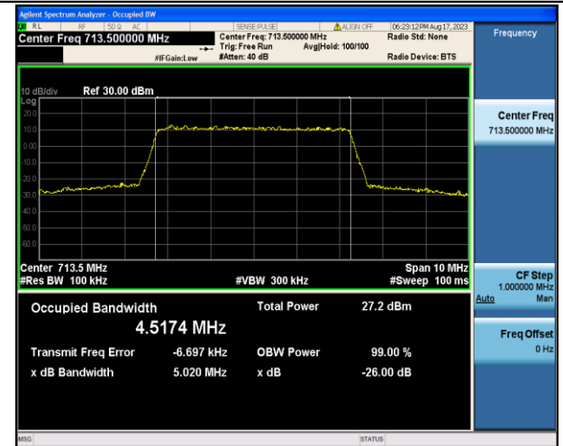
Band12-5MHz-16QAM-23155-25RB#0-PASS
