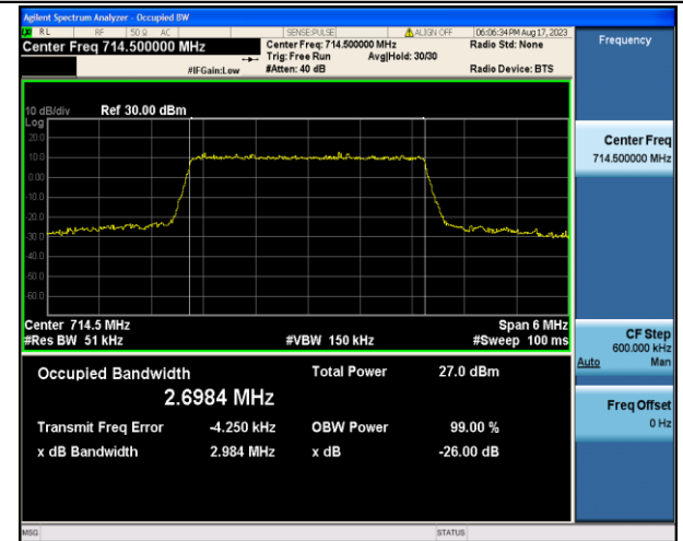
Band12-3MHz-16QAM-23165-15RB#0-PASS
