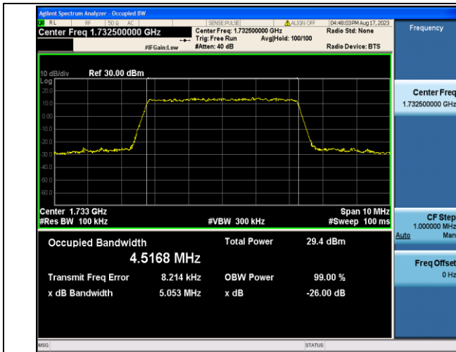
Band4-5MHz-16QAM-20175-25RB#0-PASS
