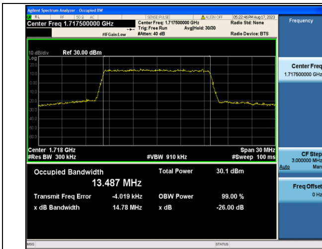
Band4-15MHz-QPSK-20025-75RB#0-PASS
