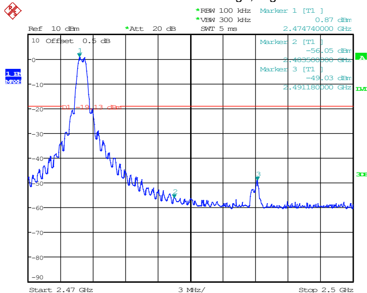
GFSK: Band Edge, Right Side
