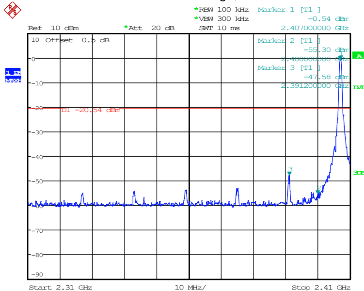
GFSK: Band Edge, Left Side
