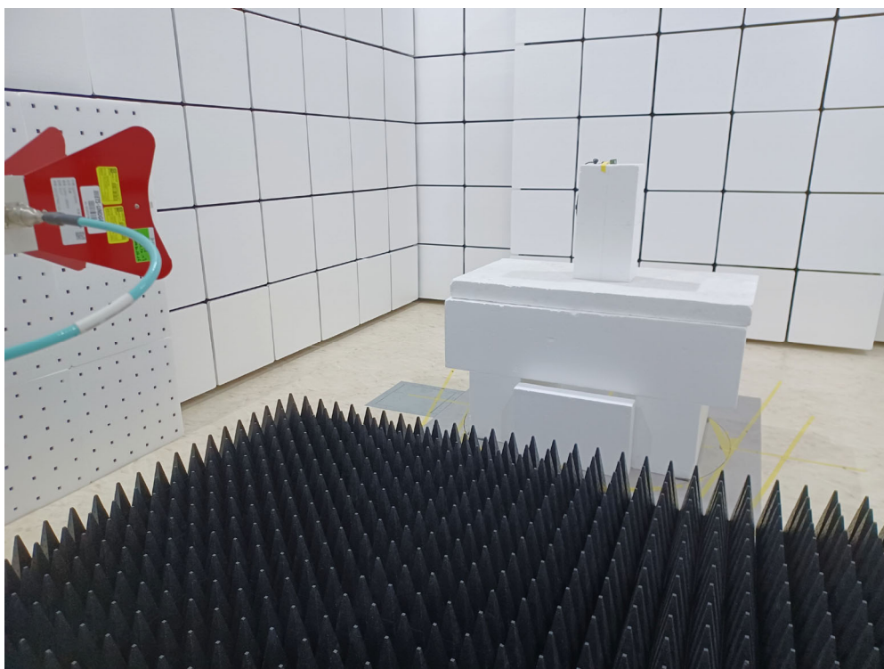
Radiated Test (Horn) (1GHz-18GHz)
