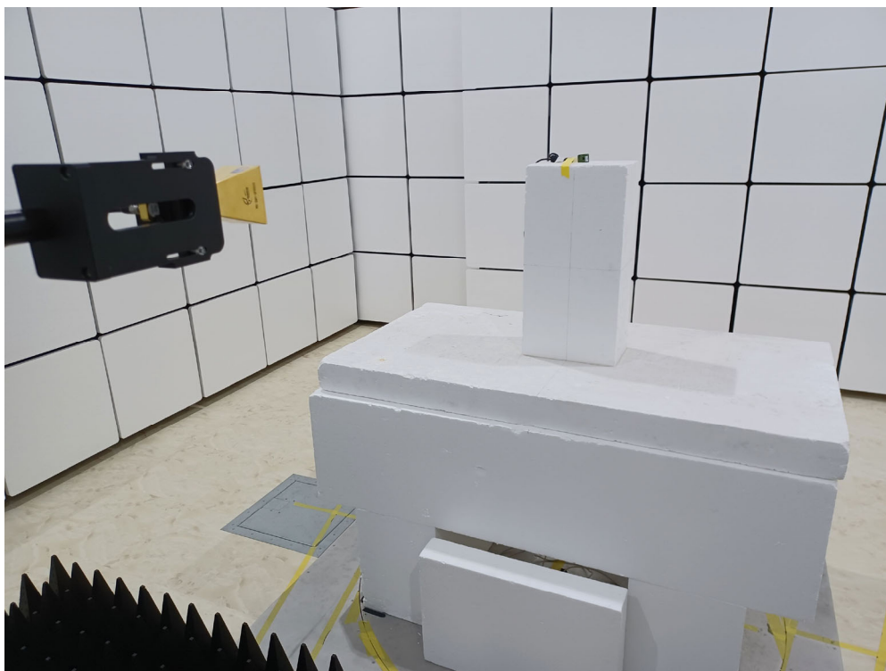
Radiated Test (Horn) (40GHz-50GHz)
