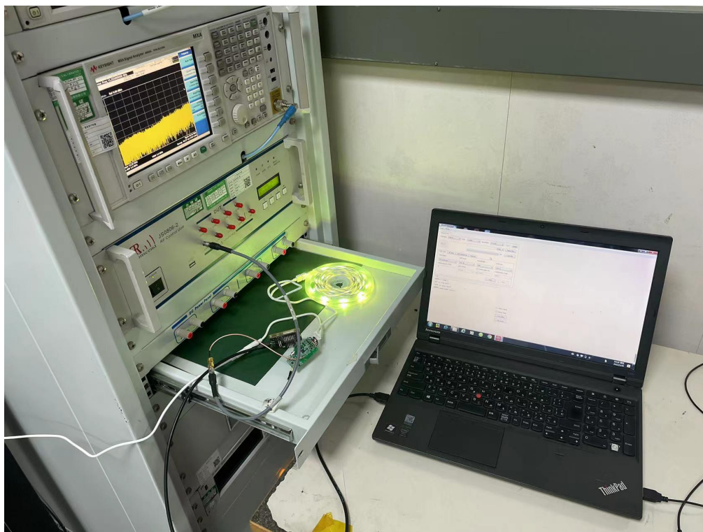
Conducted Test-WIFI
