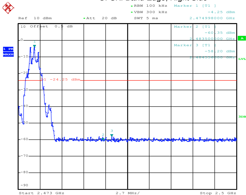
GFSK: Band Edge, Right Side
