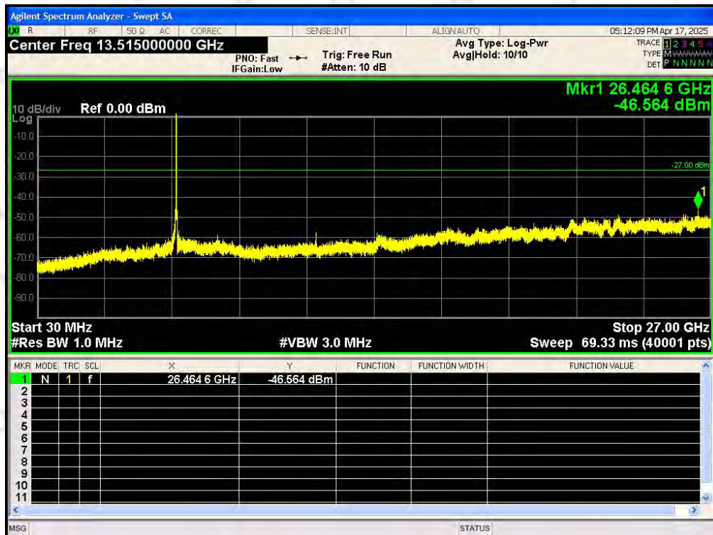
Tx. Spurious NVNT 802.11ax40 5590MHz Ant0 Emission
