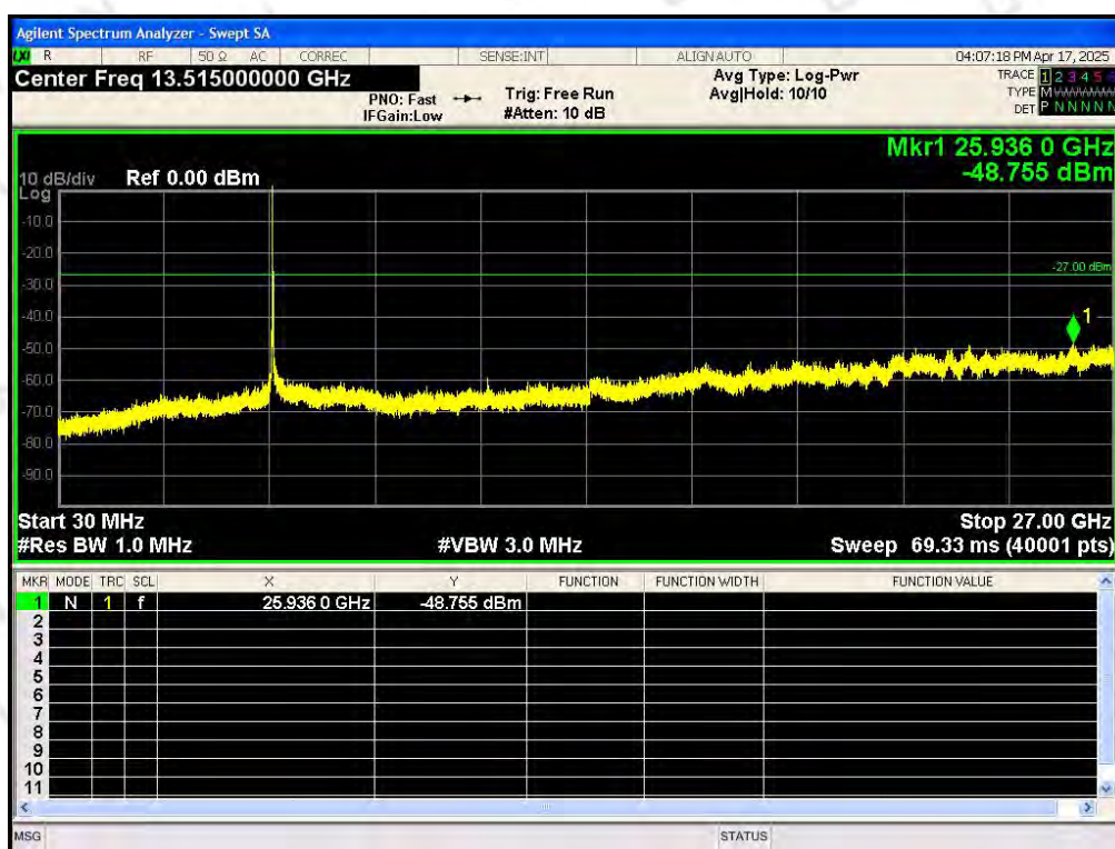
Tx. Spurious NVNT 802.11a 5500MHz Ant0 Emission
