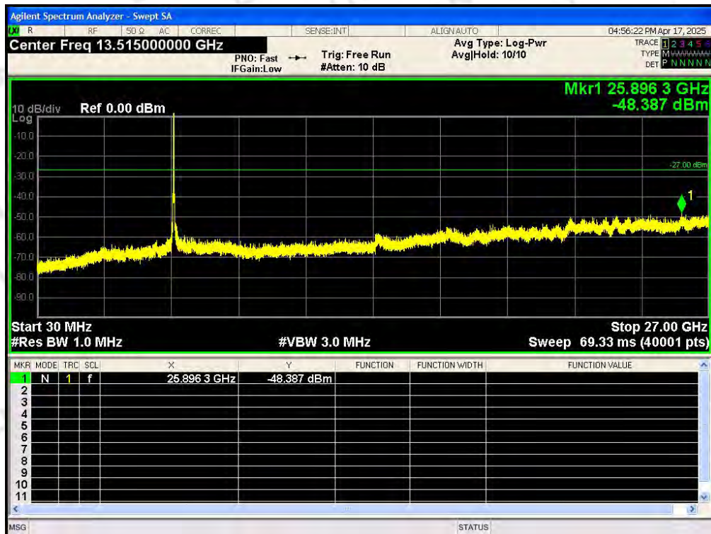
Tx. Spurious NVNT 802.11n(HT40) 5510MHz Ant0 Emission
