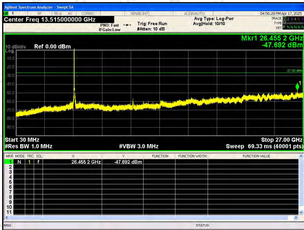
Tx. Spurious NVNT 802.11n(HT40) 5590MHz Ant0 Emission
