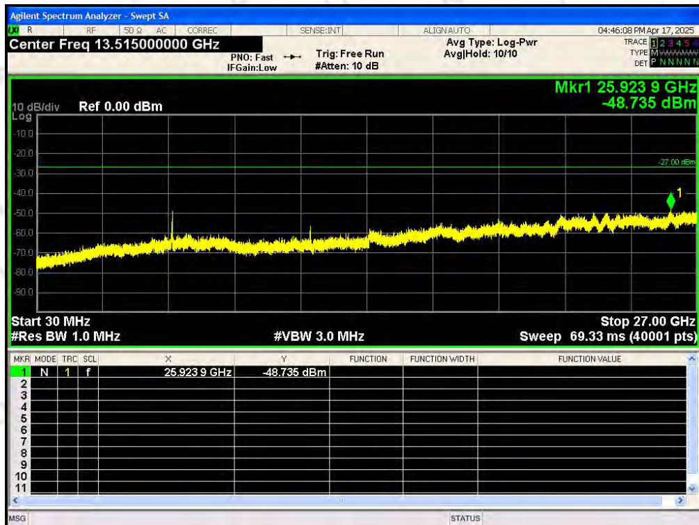
Tx. Spurious NVNT 802.11n(HT20) 5600MHz Ant0 Emission
