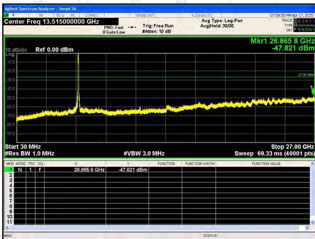
Tx. Spurious NVNT 802.11n(HT20) 5500MHz Ant0 Emission
