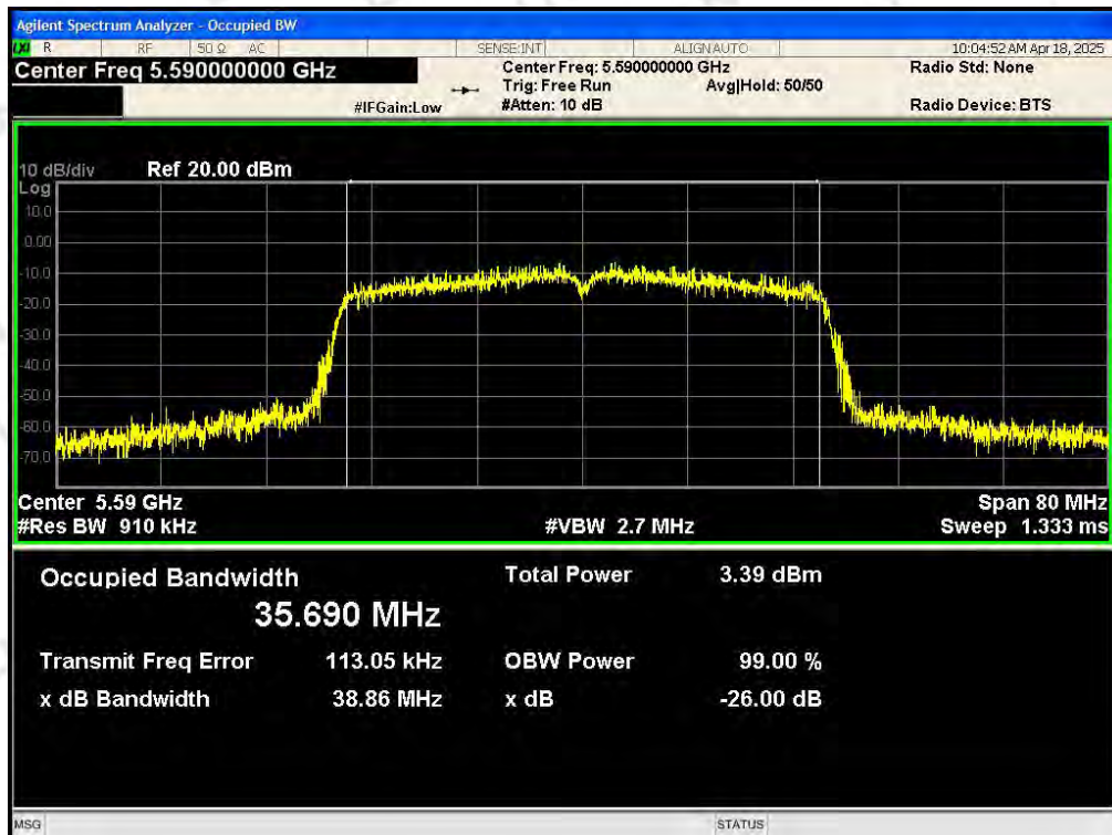
-26 dB Bandwidth NVNT 802.11n(HT40) 5590MHz Ant0
