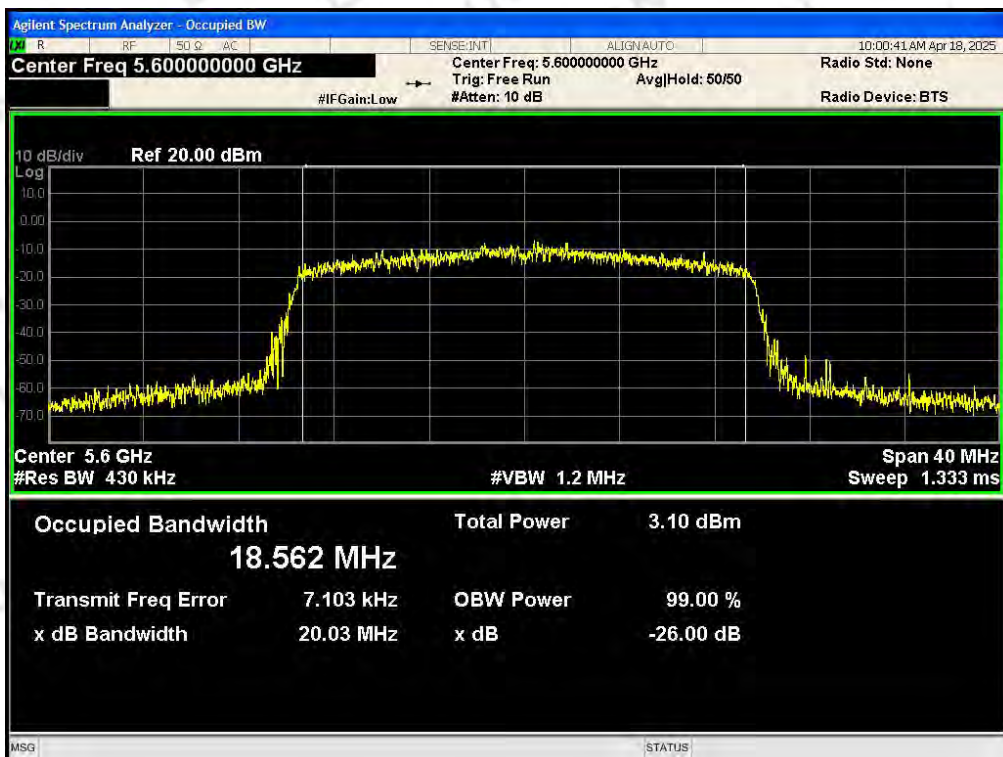
-26 dB Bandwidth NVNT 802.11ax20 5600MHz Ant0
