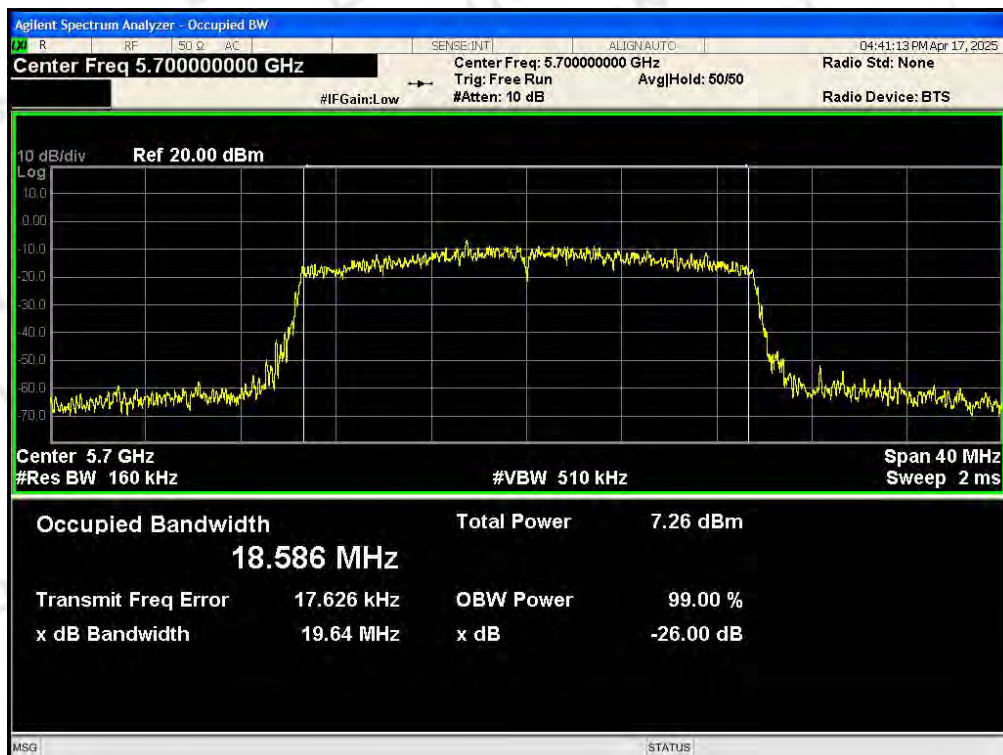
OBW NVNT 802.11ax20 5700MHz Ant0
