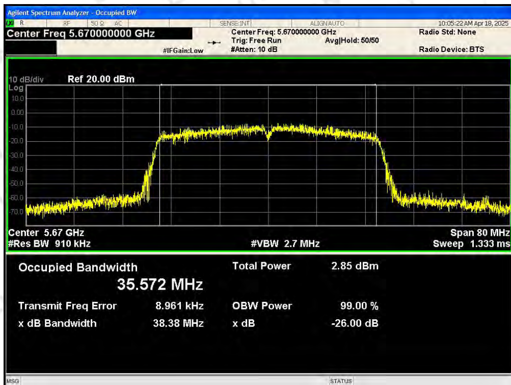
-26 dB Bandwidth NVNT 802.11n(HT40) 5670MHz Ant0
