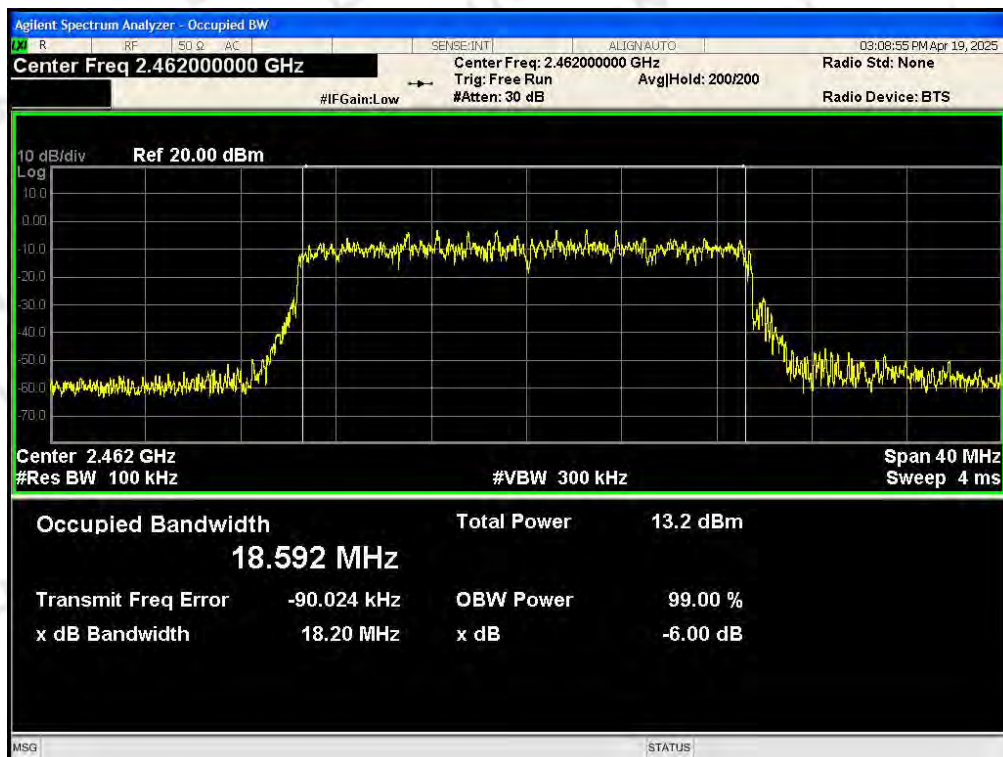
OBW NVNT 802.11ax20 2462MHz Ant1
