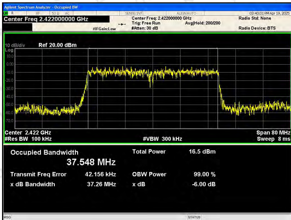
OBW NVNT 802.11ax40 2422MHz Ant1
