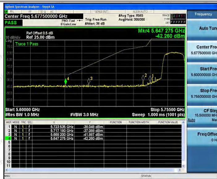
11A_Ant2_Low_5745
