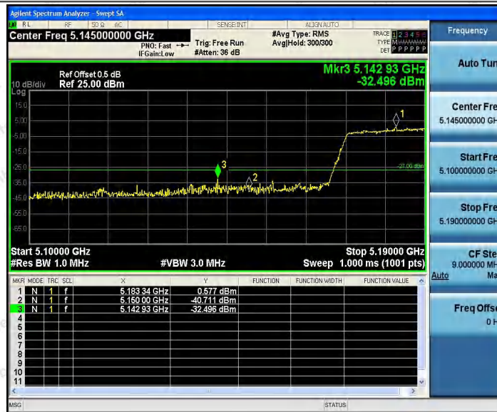
11AC80SISO_Ant2_Low_5210
