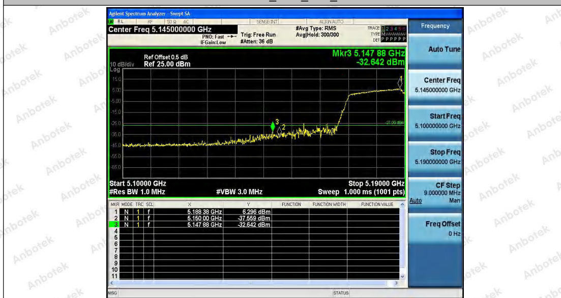
11N40SISO_Ant2_Low_5190
