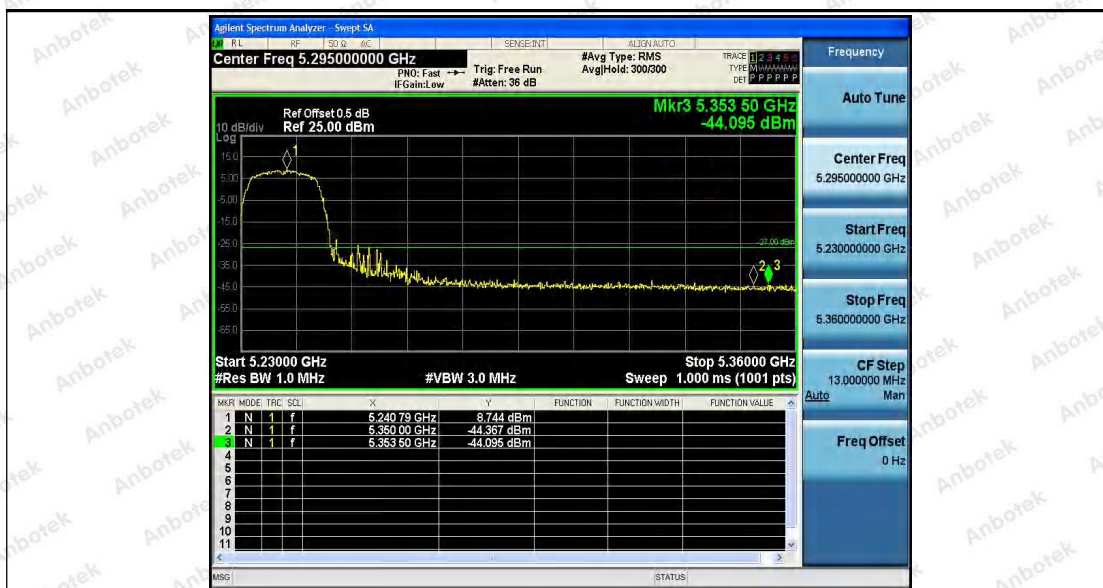
11A_Ant2_High_5240
