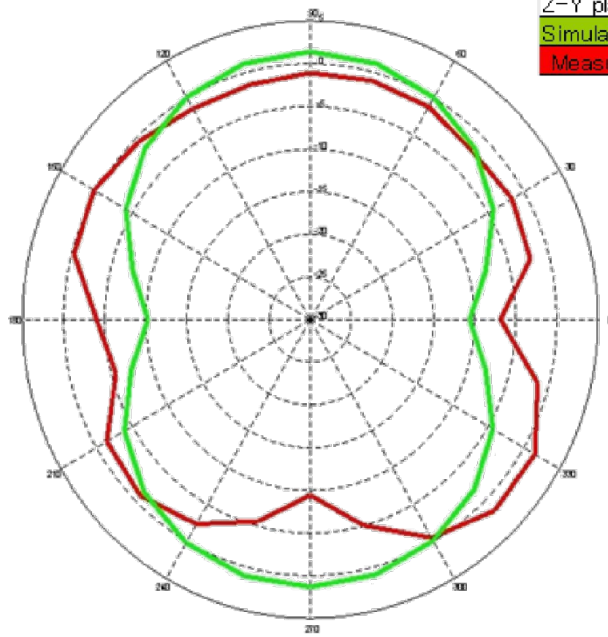
Z-Y Plane unit: dBi
