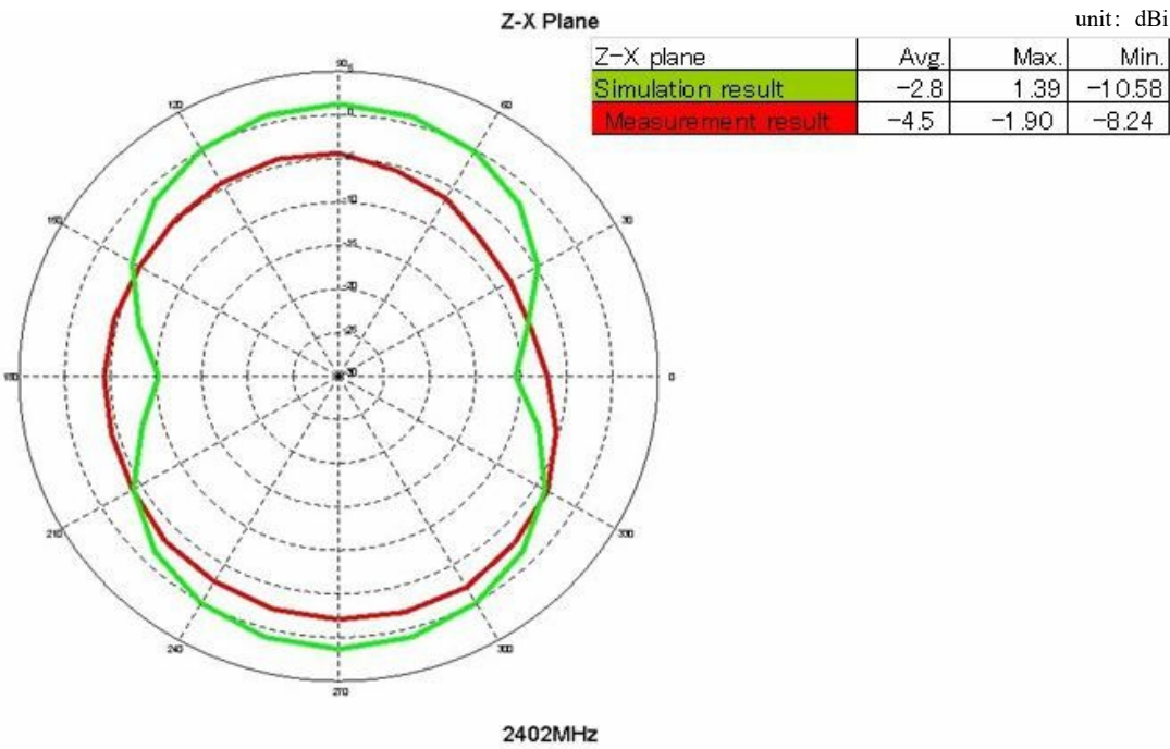
Radiation pattern @2.402GHz
