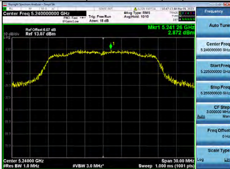
Power Spectral Density NVNT_ANT1_802_11ac(VHT20)_5240_20M
