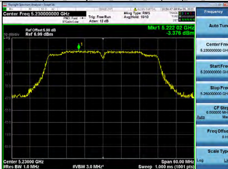
Power Spectral Density_NVNT_ANT1_802_11ac(VHT40)_5230_40M
