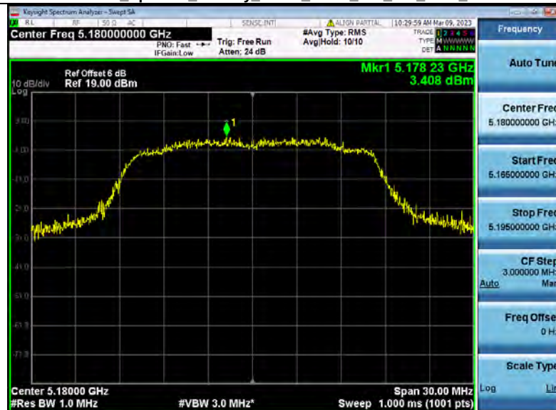
Power Spectral Density NVNT ANT1 802_11a 5180_20M
