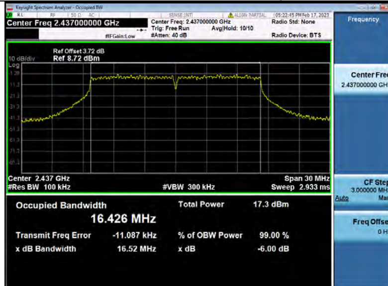
-6dB Bandwidth NVNT ANT2 802 11g 2437
