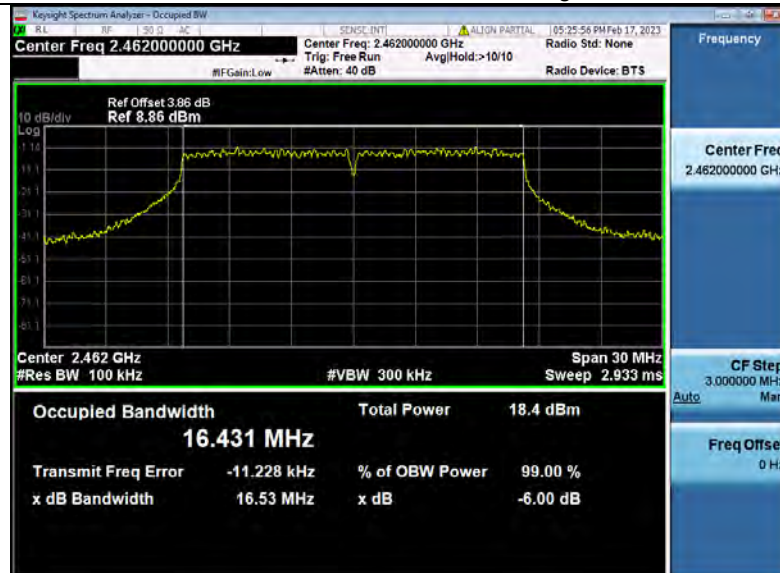
-6dB Bandwidth NVNT ANT2 802 11g 2462
