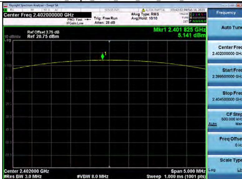
Peak Output Power_NVNT_ANT1_2-DH5_2402
