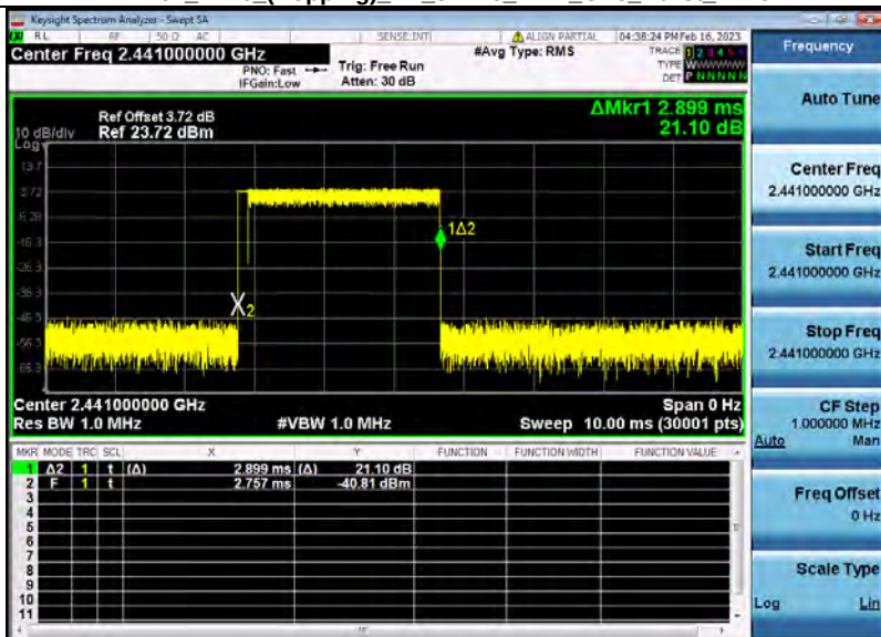
Dwell Time (Hopping) BT 3-DH5 2441 One Burst Time
