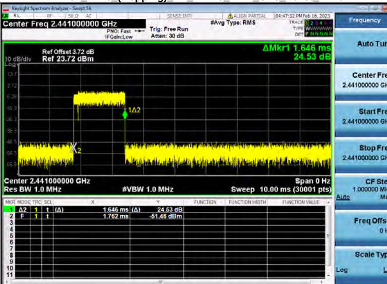
Dwell Time (Hopping) BT 2-DH3 2441 One Burst Time
