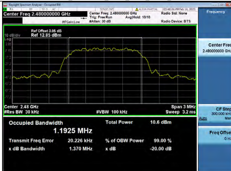
-20dB Bandwidth_NVNT_ANT1_2-DH5_2480
