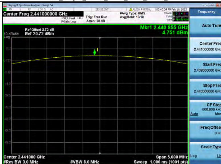
Peak Output Power_NVNT_ANT1_2-DH5_2441
