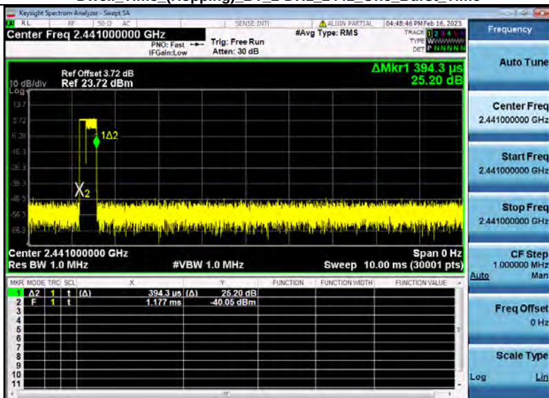
Dwell Time (Hopping) BT 2-DH1 2441 One Burst Time
