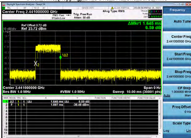
Dwell Time (Hopping) BT 3-DH3 2441 One Burst Time
