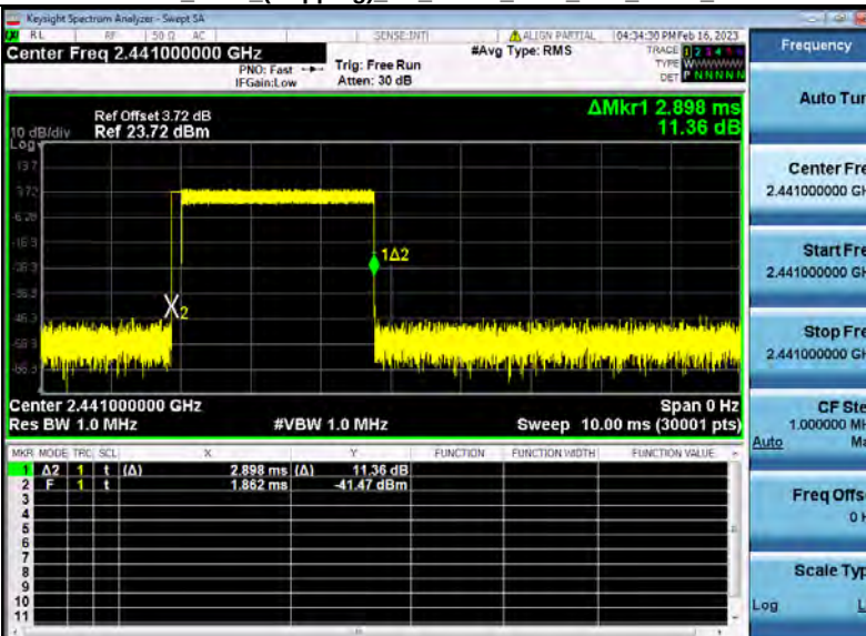
Dwell Time (Hopping) BT 2-DH5 2441 One Burst Time
