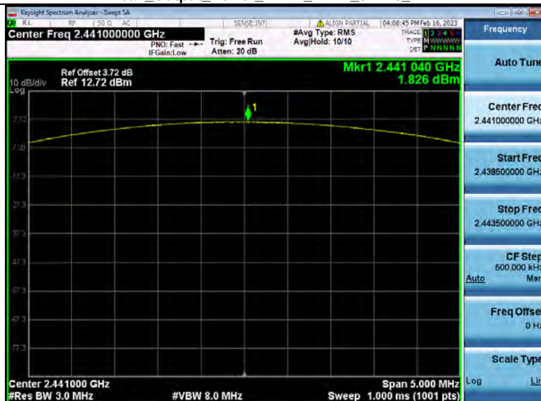
Peak Output Power_NVNT_ANT1_3-DH5_2441
