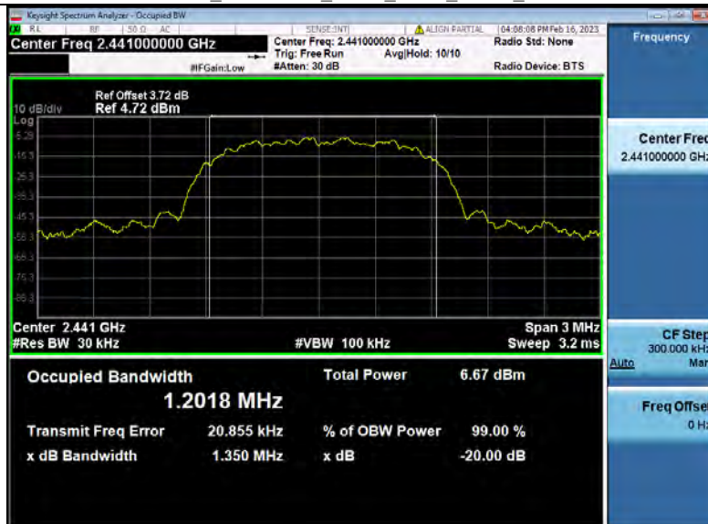
-20dB Bandwidth_NVNT_ANT1_3-DH5_2441
