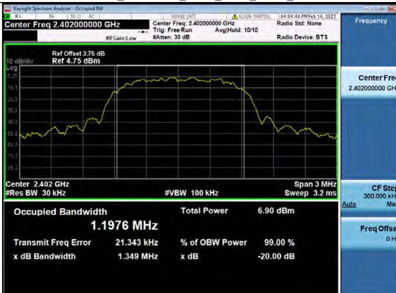
-20dB Bandwidth_NVNT_ANT1_3-DH5_2402
