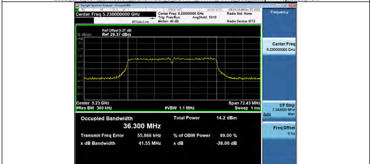
-26dB and 99% Emission Bandwidth 5 2GWiFi_NVNT_ANT1_802_11ac(VHT40)_5230_40M
