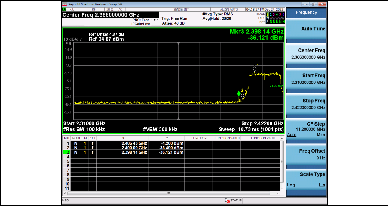
2_Bandedge_2_4GWiFi_NVNT_ANT1_802_11g_2412
