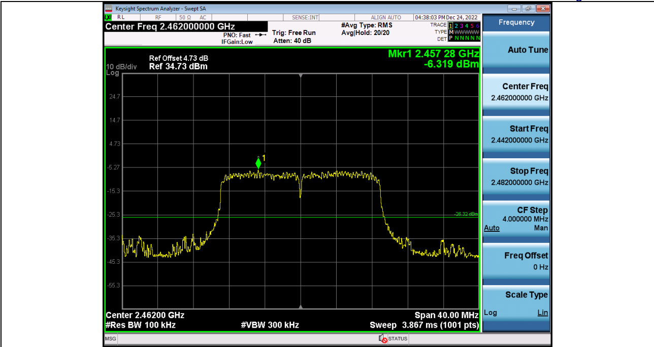
2_Bandedge_2_4GWiFi_NVNT_ANT1_802_11n(HT20)_2462
