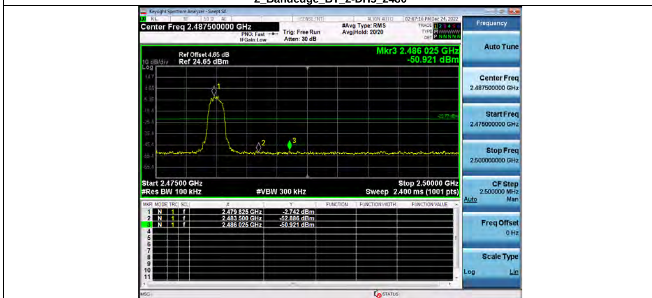
2. Bandedge BT_2-DH5_2480
