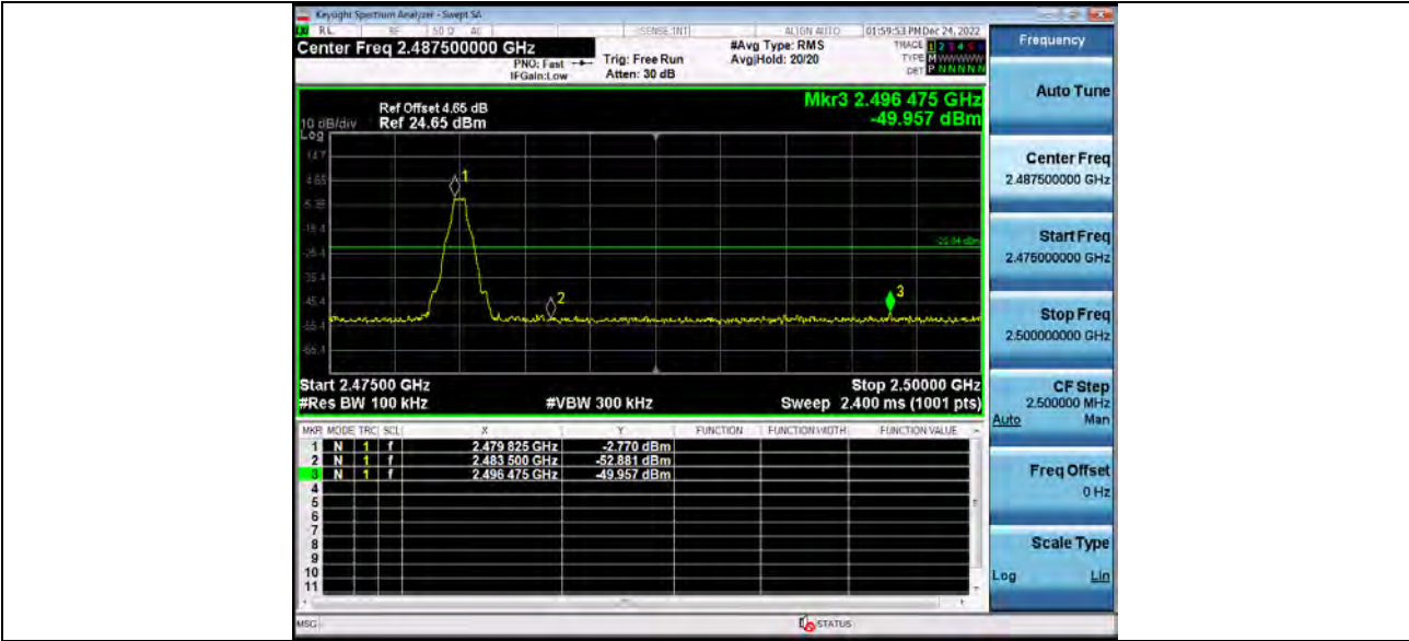
1 Reference_Level_BT_1-DH5_Hopping
