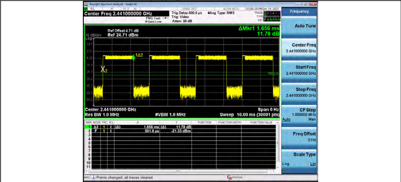
Dwell Time (Hopping) BT 3-DH3 2441 One Burst Time
