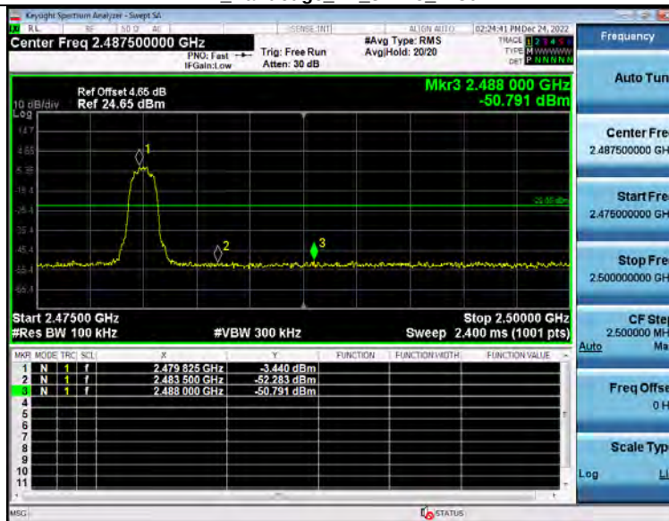
2_Bandedge_BT_3-DH5_2480
