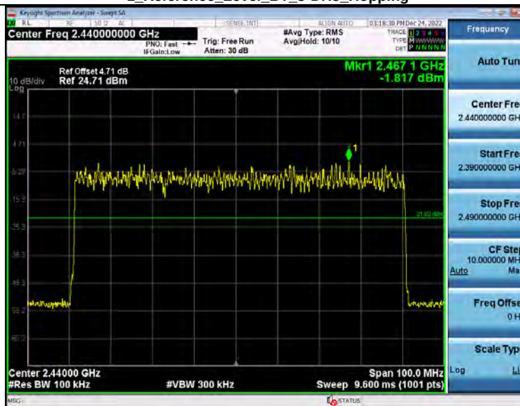
2_Band_Edge_(Hopping)_BT_3-DH5_Hopping
