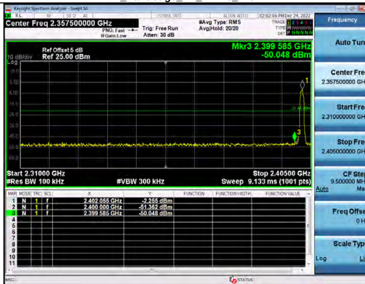
2_Bandedge_BT_2-DH5_2402
