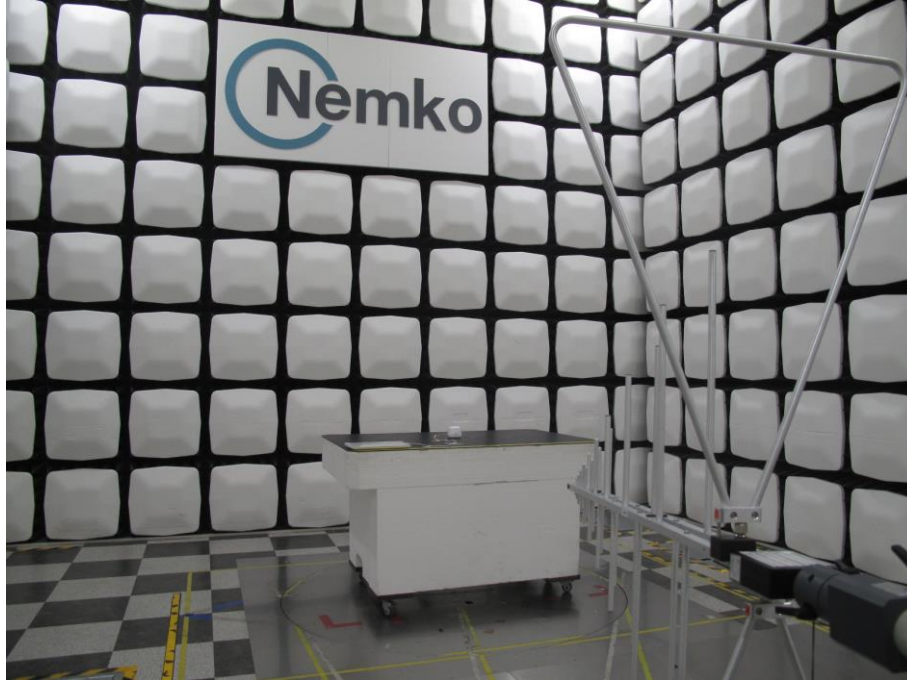
Radiated Test Picture_Below 1GHz
