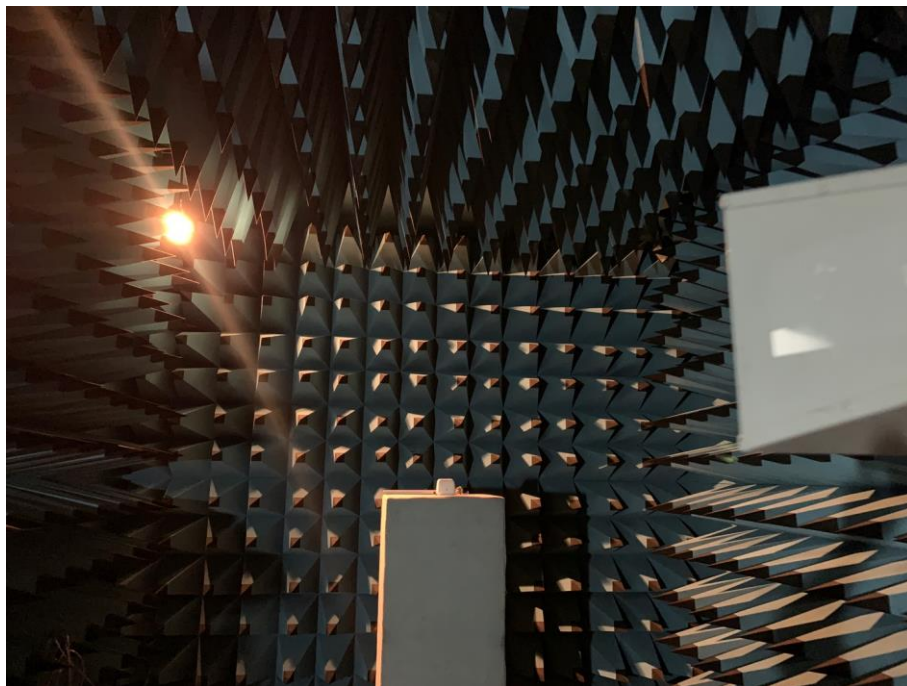
Radiated Test Picture_Above 1GHz
