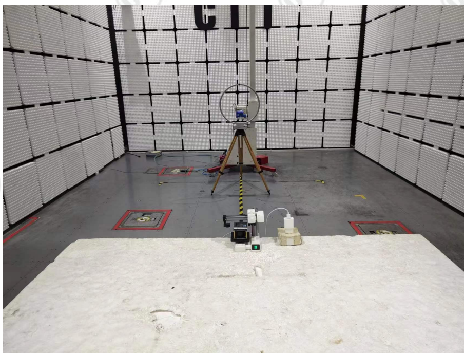
Radiated Emissions Test Setup (9kHz-30MHz) Mode b to Mode e
