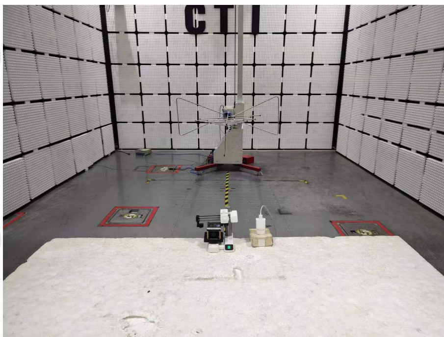
Radiated Emissions Test Setup (30MHz-1GHz)Mode b to Mode e
