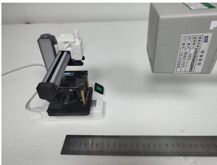
Test Setup of Front (Mode b to Mode e)
