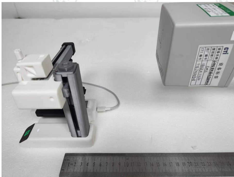
Test Setup of Rear (Mode a)
