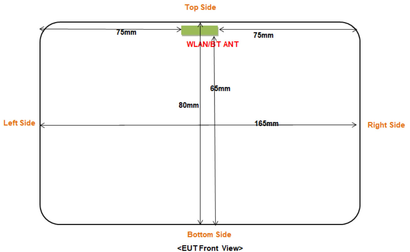
Fig 7.1 Block Diagram for EUT Antenna Position EUT Sizes: Long 165mm; width 80mm; height: 40mm
