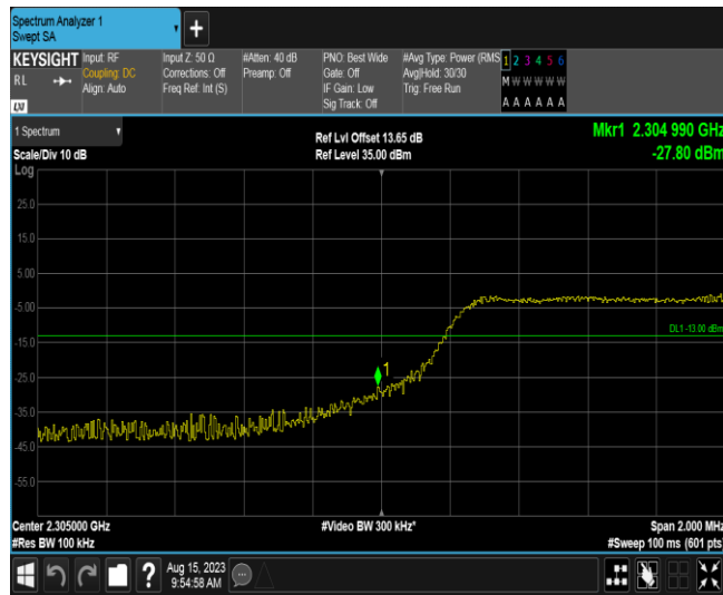
Band40-5MHz-16QAM-38775-1RB#0
