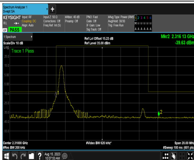
Band40-10MHz-16QAM-38750-1RB#0
