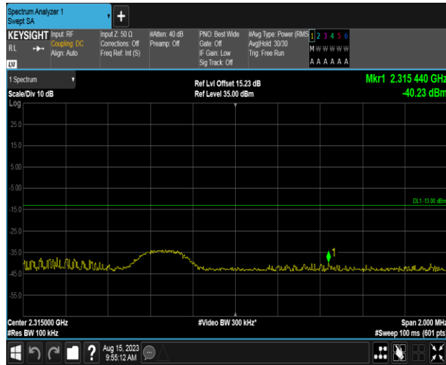
Band40-5MHz-QPSK-38775-1RB#24
