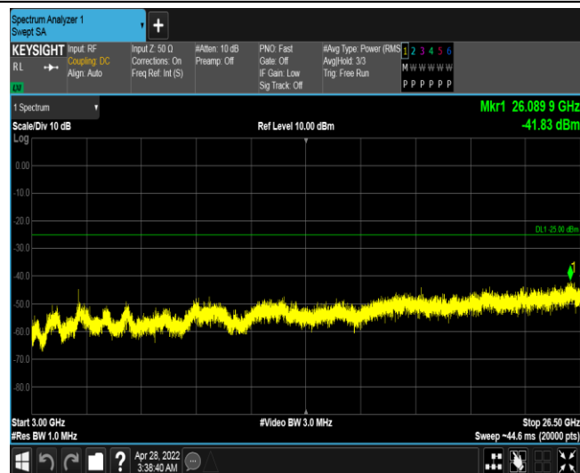
Band41-10MHz-16QAM-39700-1RB#0-Range3:3000~26500MHz
