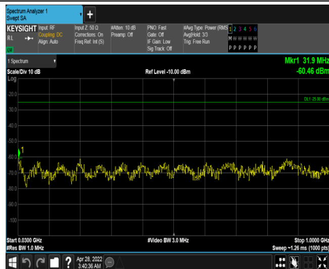
Band41-10MHz-QPSK-41540-1RB#0-Range1:30~1000MHz
