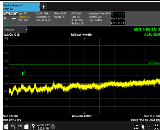
Band41-5MHz-16QAM-40620-1RB#0-Range3:3000~26500MHz
