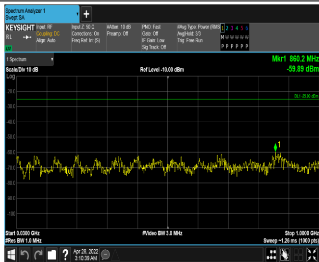
Band41-5MHz-16QAM-39675-1RB#0-Range1:30~1000MHz
