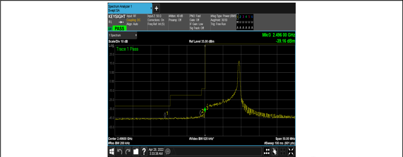
Band41-10MHz-QPSK-39700-1RB#49
