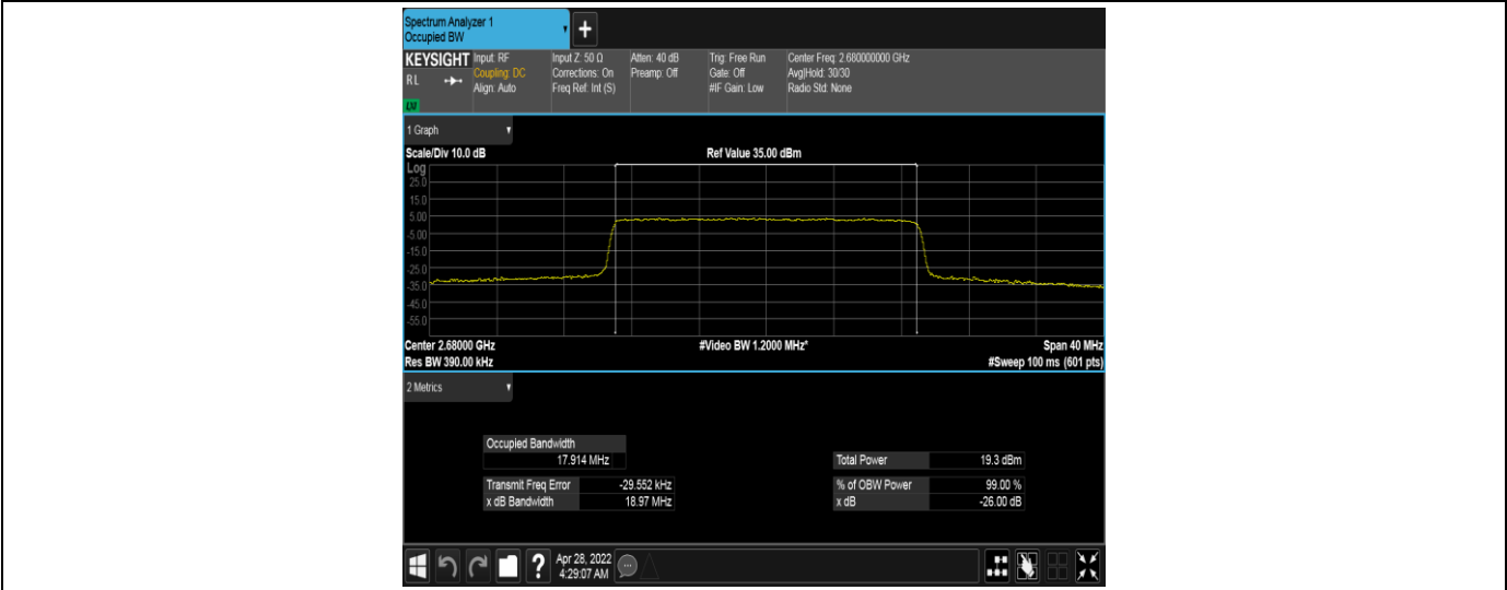
Band41-20MHz-16QAM-41490-100RB#0
