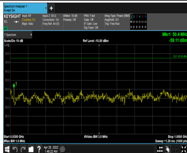
Band38-10MHz-QPSK-38200-1RB#0-Range1:30~1000MHz
