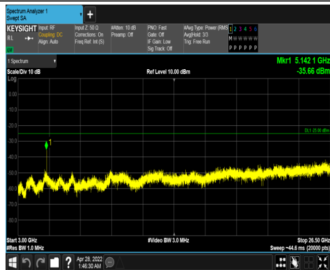
Band38-10MHz-16QAM-37800-1RB#0-Range3:3000~26500MHz
