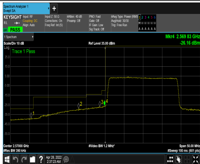
Band38-20MHz-QPSK-37850-100RB#0
