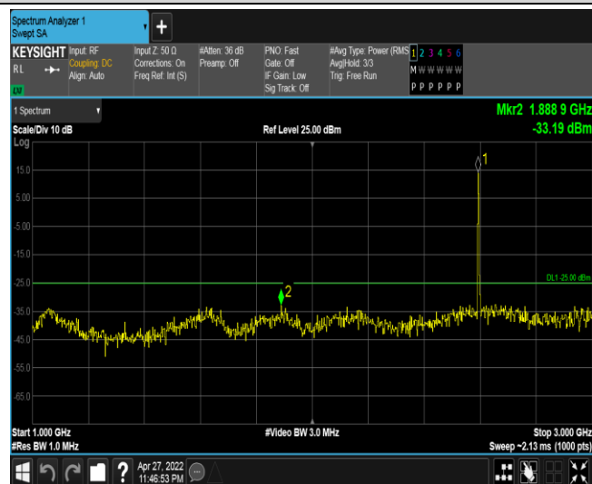
Band38-5MHz-QPSK-38000-1RB#0-Range2:1000~3000MHz
