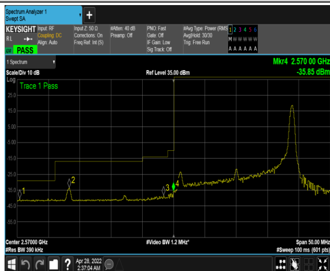
Band38-20MHz-16QAM-37850-1RB#99
