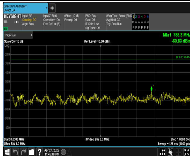
Band38-5MHz-16QAM-37775-1RB#0-Range1:30~1000MHz
