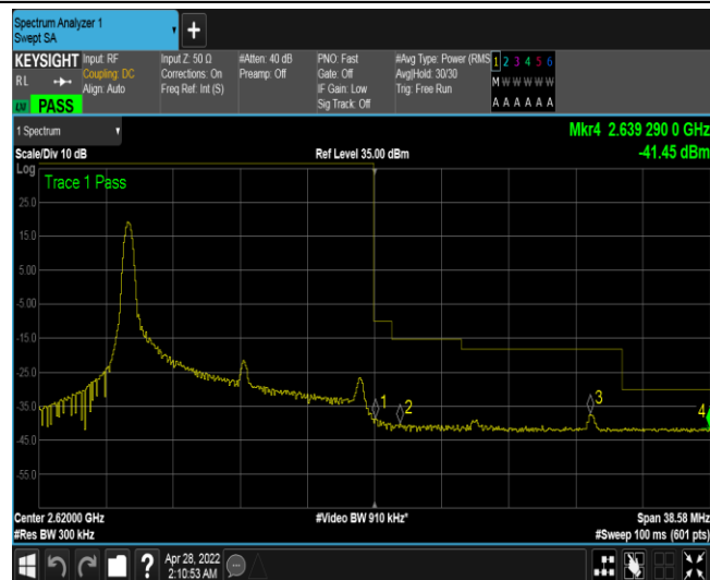
Band38-15MHz-16QAM-38175-1RB#0
