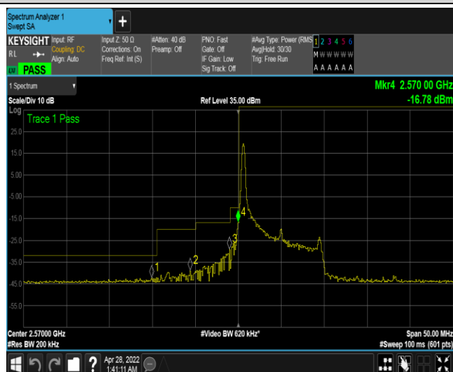
Band38-10MHz-QPSK-37800-1RB#49
