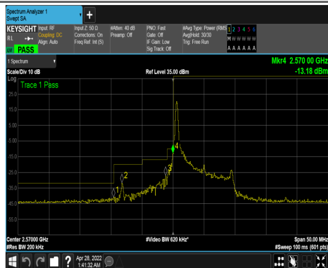
Band38-10MHz-16QAM-37800-1RB#0
