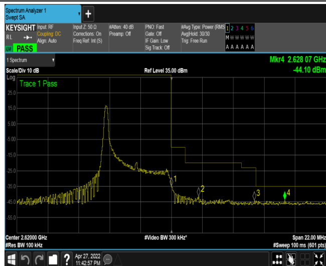
Band38-5MHz-QPSK-38225-1RB#0
