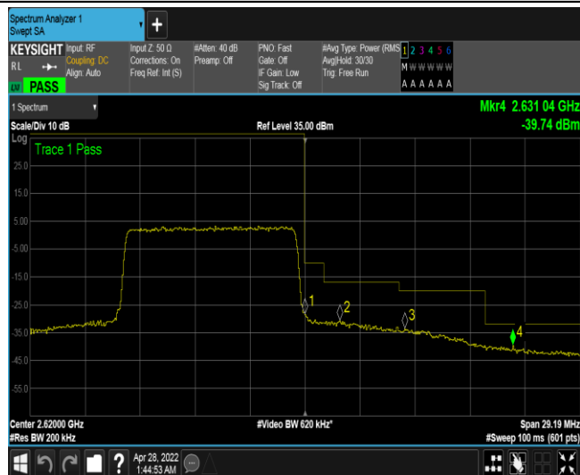
Band38-10MHz-16QAM-38200-50RB#0
