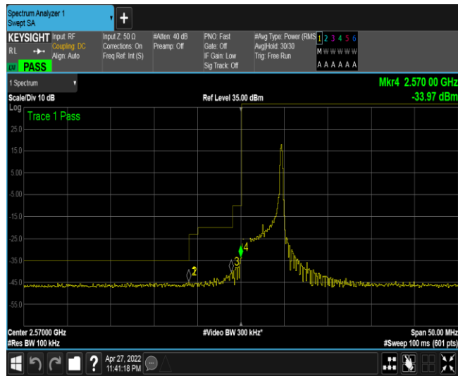
Band38-5MHz-QPSK-37775-25RB#0
