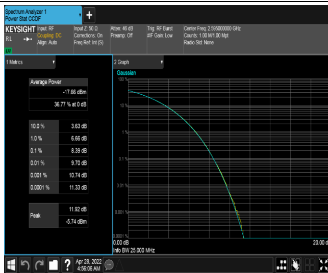
Band38-15MHz-QPSK-38000-75RB#0
