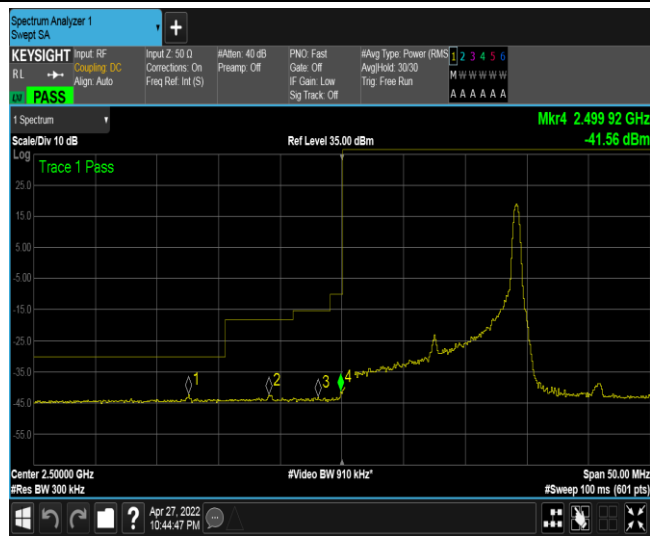
Band7-15MHz-16QAM-20825-75RB#0
