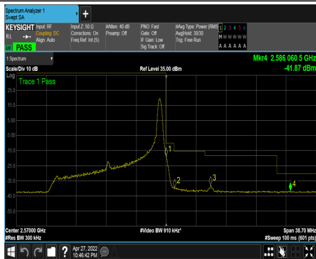
Band7-15MHz-QPSK-21375-1RB#74
