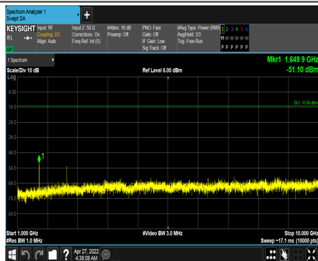
Band5-3MHz-16QAM-20415-1RB#0-Range3:1000~10000MHz
