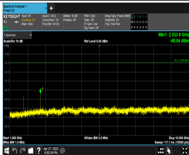
Band5-5MHz-QPSK-20625-1RB#0-Range3:1000~10000MHz
