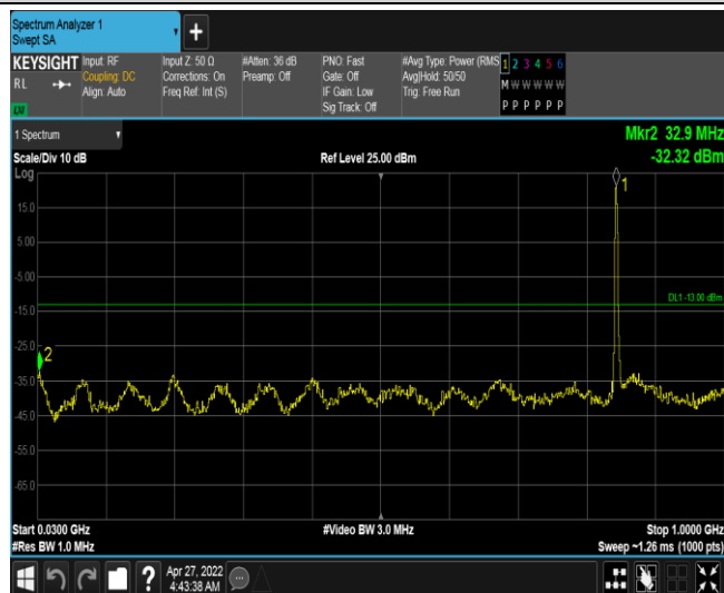
Band5-3MHz-16QAM-20635-1RB#0-Range2:30~1000MHz
