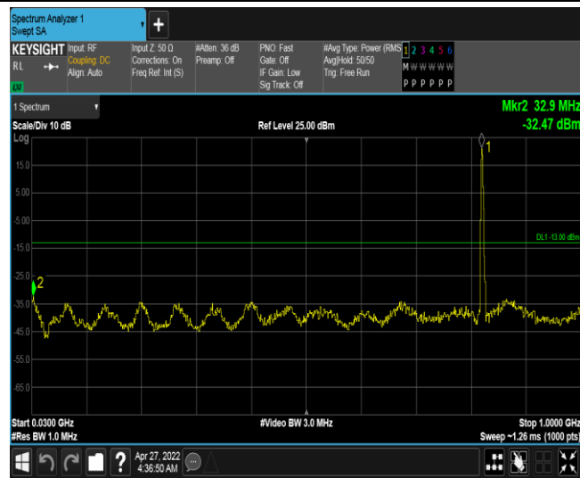
Band5-3MHz-16QAM-20415-1RB#0-Range2:30~1000MHz
