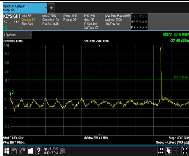
Band5-5MHz-QPSK-20625-1RB#0-Range1:30~1000MHz
