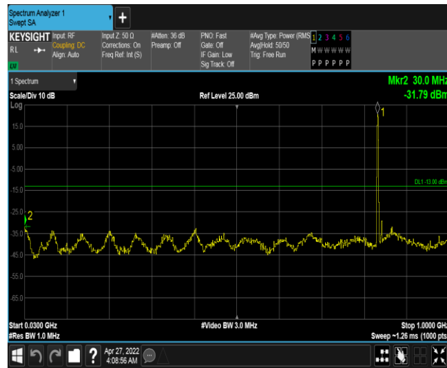
Band5-1.4MHz-16QAM-20525-1RB#0-Range2:30~1000MHz
