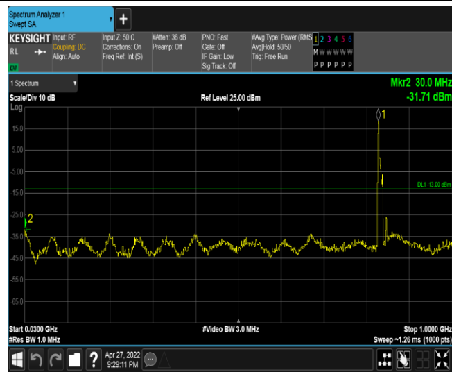
Band5-10MHz-QPSK-20525-1RB#0-Range2:30~1000MHz
