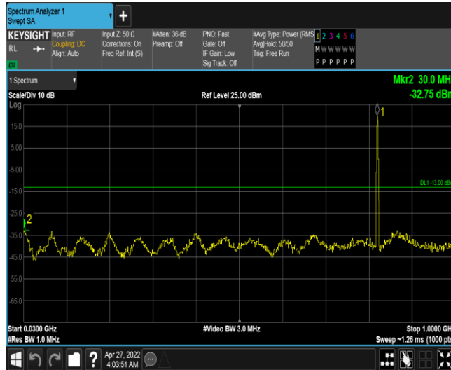
Band5-1.4MHz-QPSK-20407-1RB#0-Range1:30~1000MHz
