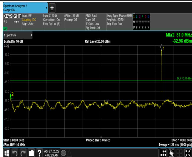
Band5-1.4MHz-QPSK-20525-1RB#0-Range2:30~1000MHz
