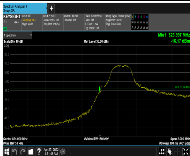
Band5-3MHz-16QAM-20415-1RB#0
